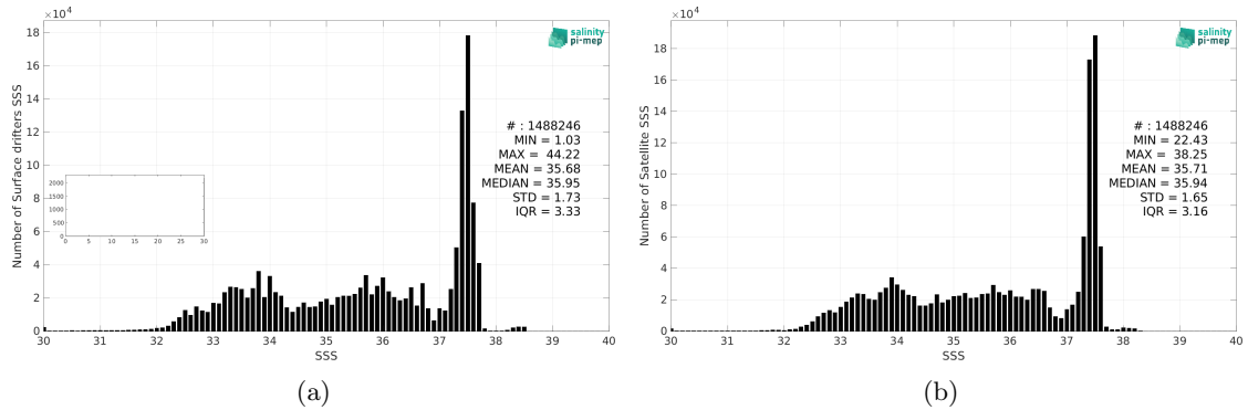
Figure 2: Histograms of SSS from Surface drifters (a) and CCI SSS L4 Merged-OI v4.4 - 7-day running (ESA) (b) considering all match-up pairs per bins of 0.1 over the Global Ocean Pi-MEP region and for the full satellite product period.
