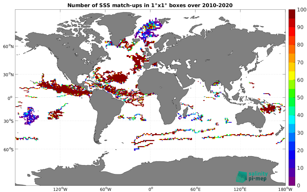
Figure 3: Number of SSS match-ups between Surface drifters SSS and the CCI SSS L4 Merged-OI v4.4 - 7-day running (ESA) SSS product for the Global Ocean Pi-MEP region over 1^\circ \times 1^\circ boxes and for the full satellite product period.
