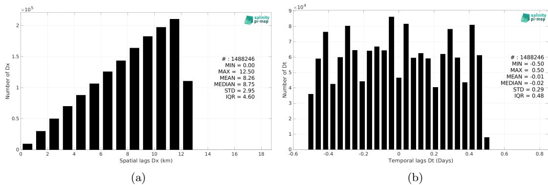
Figure 4: Histograms of the spatial (a) and temporal (b) lags between the location/time of the Surface drifters measurement and the date of the corresponding CCI SSS L4 Merged-OI v4.4 - 7-day running (ESA) SSS pixel.
