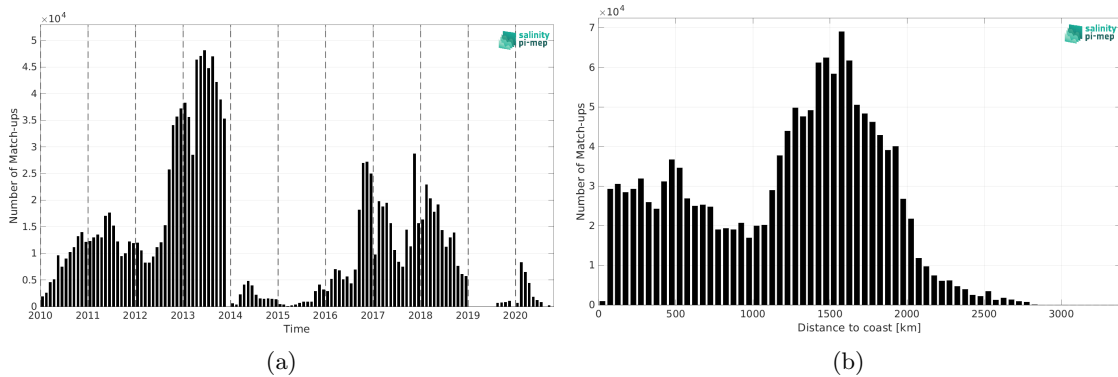
Figure 1: Number of match-ups between Surface drifters and CCI SSS L4 Merged-OI v4.4 - 7-day running (ESA) SSS as a function of time (a) and as function of the distance to coast (b) over the Global Ocean Pi-MEP region and for the full satellite product period.
