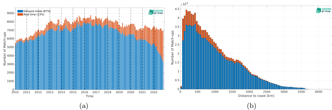
Figure 1: Number of match-ups between Argo and CCI SSS L4 Merged-OI v4.4 - 7-day running (ESA) SSS as a function of time (a) and as function of the distance to coast (b) over the Global Ocean Pi-MEP region and for the full satellite product period.
