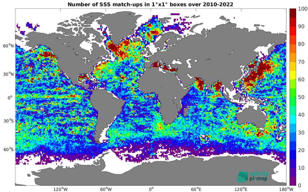
Figure 4: Number of SSS match-ups between Argo SSS and the CCI SSS L4 Merged-OI v4.4 - 7-day running (ESA) SSS product for the Global Ocean Pi-MEP region over 1^\circ \times 1^\circ boxes and for the full satellite product period.
