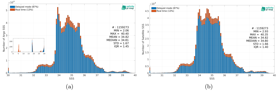
Figure 2: Histograms of SSS from Argo (a) and CCI SSS L4 Merged-OI v4.4 - 7-day running (ESA) (b) considering all match-up pairs per bins of 0.1 over the Global Ocean Pi-MEP region and for the full satellite product period.
