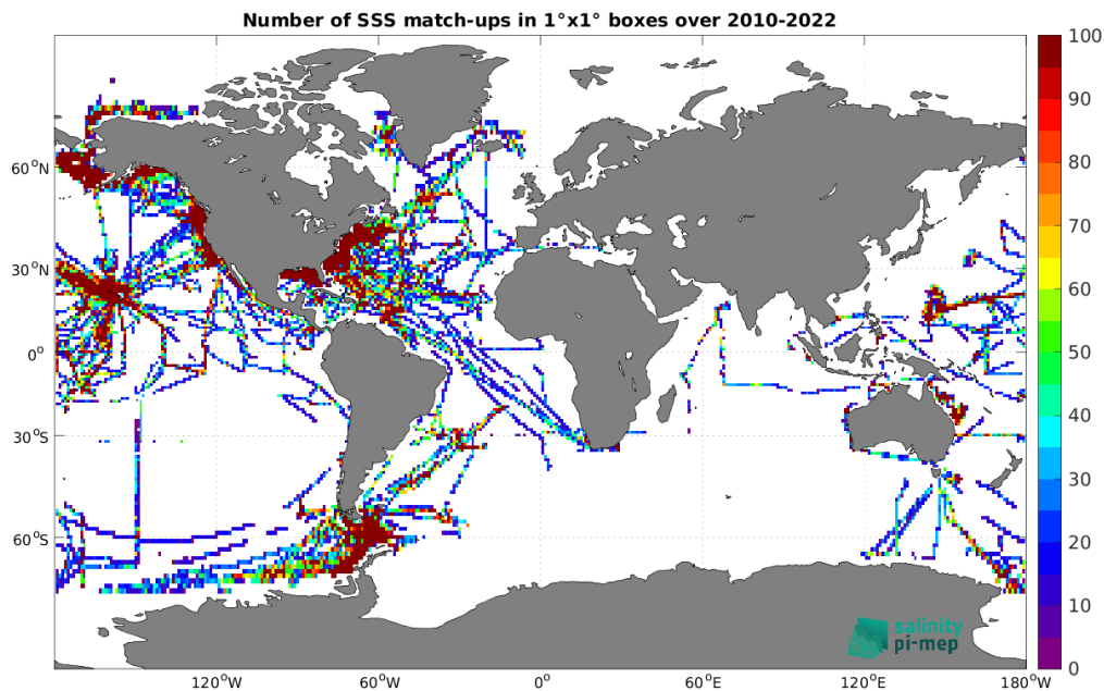
Figure 4: Number of SSS match-ups between TSG (SAMOS) SSS and the CCI SSS L4 Merged-OI v4.4 - 30-day running (ESA) SSS product for the Global Ocean Pi-MEP region over 1^\circ \times 1^\circ boxes and for the full satellite product period.
