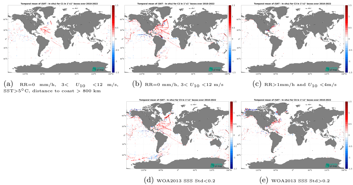
Figure 12: Temporal mean gridded over spatial boxes of size 1^\circ \times 1^\circ of \Delta\text{SSS} (CCI SSS L4 Merged-OI v4.4 - 30-day running (ESA) - TSG (SAMOS)) for 5 different subdatasets corresponding to:RR=0 mm/h, 3 < U_{10} < 12 m/s, SST >5^\circ\text{C} , distance to coast > 800 km (a), RR=0 mm/h, 3 < U_{10} < 12 m/s (b), RR >1 mm/h and U_{10} < 4 m/s (c), WOA2013 SSS Std <0.2 (d), WOA2013 SSS Std >0.2 (e).
