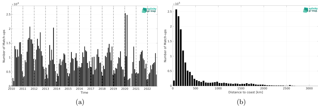
Figure 1: Number of match-ups between TSG (SAMOS) and CCI SSS L4 Merged-OI v4.4 - 30-day running (ESA) SSS as a function of time (a) and as function of the distance to coast (b) over the Global Ocean Pi-MEP region and for the full satellite product period.
