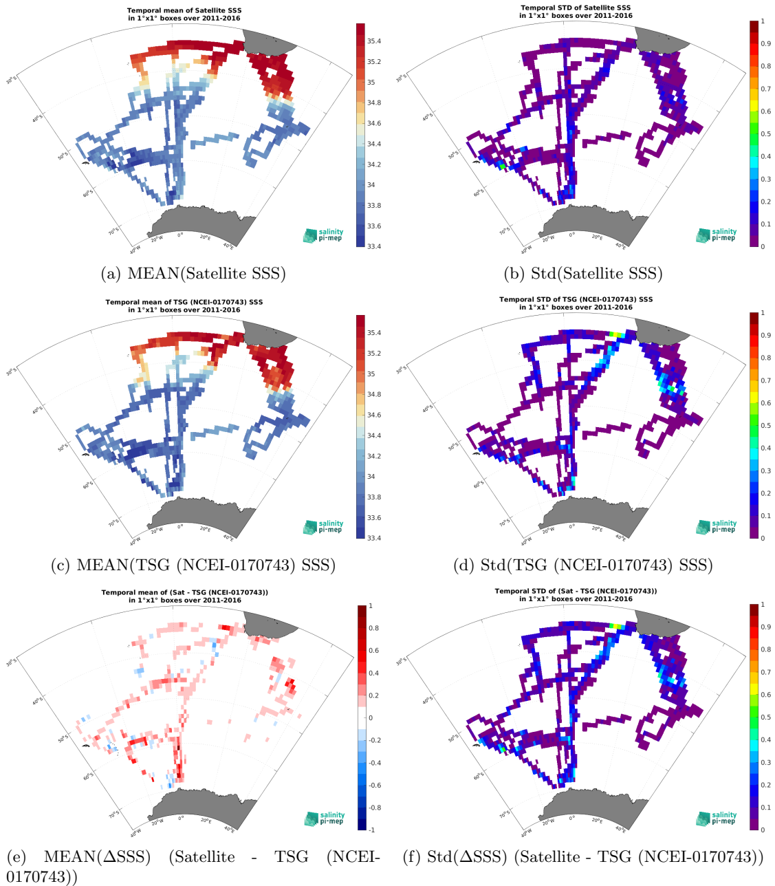
Figure 6: Temporal mean (left) and Std (right) of SSS from CCI SSS L4 Merged-OI v4.4 - 30-day running (ESA) (top), TSG (NCEI-0170743) (middle), and of \Delta SSS (Satellite - TSG (NCEI-0170743)). Only match-up pairs are used to generate these maps.
