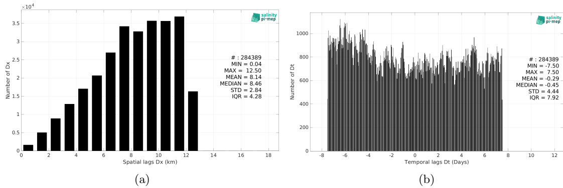
Figure 5: Histograms of the spatial (a) and temporal (b) lags between the location/time of the TSG (NCEI-0170743) measurement and the date of the corresponding CCI SSS L4 Merged-OI v4.4 - 30-day running (ESA) SSS pixel.
