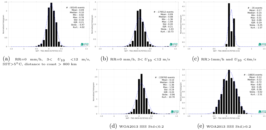
Figure 13: Normalized histogram of \Delta SSS (CCI SSS L4 Merged-OI v4.4 - 30-day running (ESA) - TSG (NCEI-0170743)) for 5 different subdatasets corresponding to: RR=0 mm/h, 3 < U_{10} < 12 m/s, SST>5°C, distance to coast > 800 km (a), RR=0 mm/h, 3 < U_{10} < 12 m/s (b), RR>1mm/h and U_{10} < 4 m/s (c), WOA2013 SSS Std<0.2 (d), WOA2013 SSS Std>0.2 (e).
