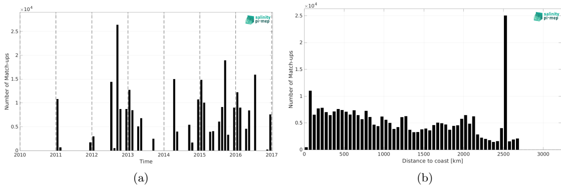
Figure 1: Number of match-ups between TSG (NCEI-0170743) and CCI SSS L4 Merged-OI v4.4 - 30-day running (ESA) SSS as a function of time (a) and as function of the distance to coast (b) over the Global Ocean Pi-MEP region and for the full satellite product period.
