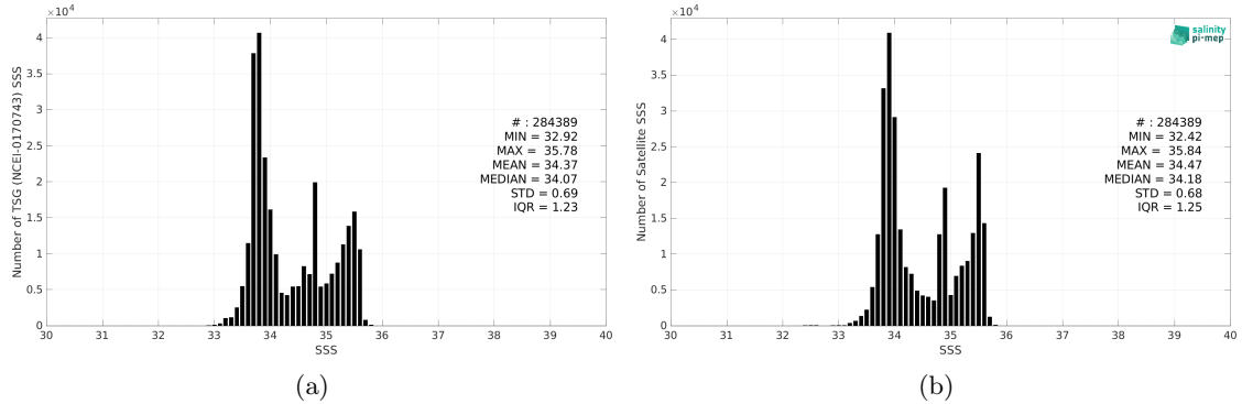
Figure 2: Histograms of SSS from TSG (NCEI-0170743) (a) and CCI SSS L4 Merged-OI v4.4 - 30-day running (ESA) (b) considering all match-up pairs per bins of 0.1 over the Global Ocean Pi-MEP region and for the full satellite product period.
