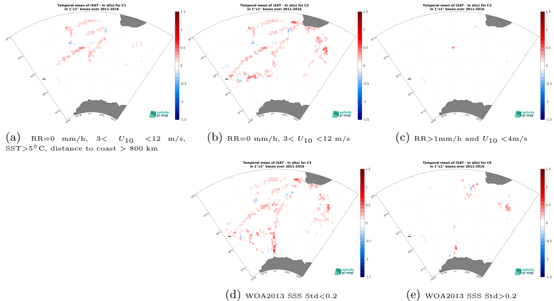
Figure 12: Temporal mean gridded over spatial boxes of size 1^{\circ}\times 1^{\circ} of \Delta\text{SSS} (CCI SSS L4 Merged-OI v4.4 - 30-day running (ESA) - TSG (NCEI-0170743)) for 5 different subdatasets corresponding to:RR=0 mm/h, 3 < U_{10} < 12 m/s, SST >5^{\circ}\text{C} , distance to coast > 800 km (a), RR=0 mm/h, 3 < U_{10} < 12 m/s (b), RR >1 mm/h and U_{10} < 4 m/s (c), WOA2013 SSS Std <0.2 (d), WOA2013 SSS Std >0.2 (e).
