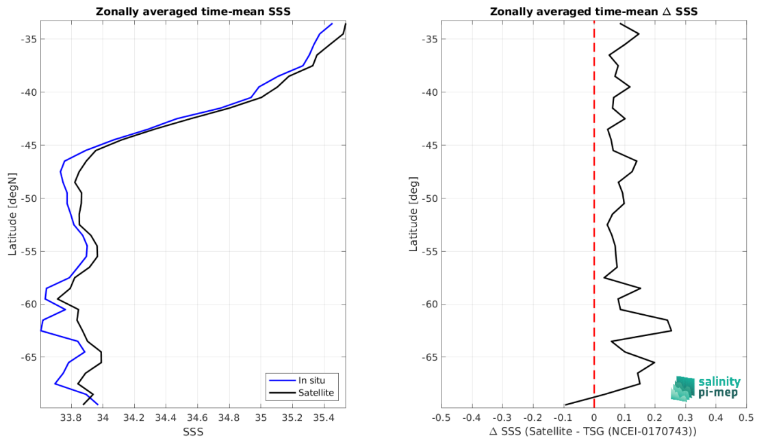
Figure 8: Left panel: Zonal mean SSS from CCI SSS L4 Merged-OI v4.4 - 30-day running (ESA) satellite product (black) and from TSG (NCEI-0170743) (blue). Right panel: Zonal mean of \Delta SSS (Satellite - TSG (NCEI-0170743)) for all the collected Pi-MEP match-up pairs estimated over the full satellite product period.
