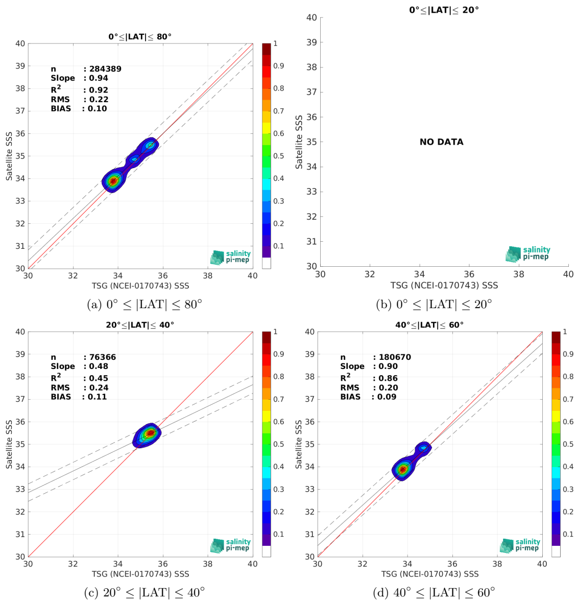
Figure 9: Contour maps of the concentration of CCI SSS L4 Merged-OI v4.4 - 30-day running (ESA) SSS (y-axis) versus TSG (NCEI-0170743) SSS (x-axis) at match-up pairs for different latitude bands. For each plot, the red line shows x=y . The black thin and dashed lines indicate a linear fit through the data cloud and the \pm 95\% confidence levels, respectively. The number match-up pairs n , the slope and R^2 coefficient of the linear fit, the root mean square (RMS) and the mean bias between satellite and in situ data are indicated for each latitude band in each plots.
