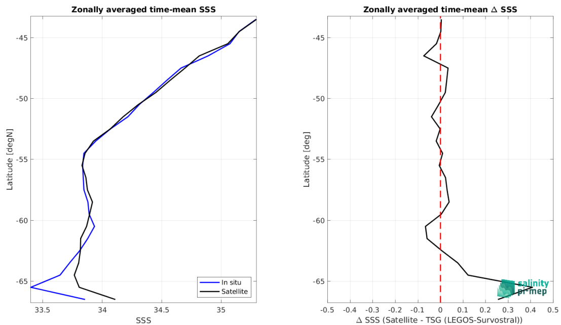
Figure 8: Left panel: Zonal mean SSS from CCI SSS L4 Merged-OI v4.4 - 30-day running (ESA) satellite product (black) and from TSG (LEGOS-Survostral) (blue). Right panel: Zonal mean of \Delta SSS (Satellite - TSG (LEGOS-Survostral)) for all the collected Pi-MEP match-up pairs estimated over the full satellite product period.
