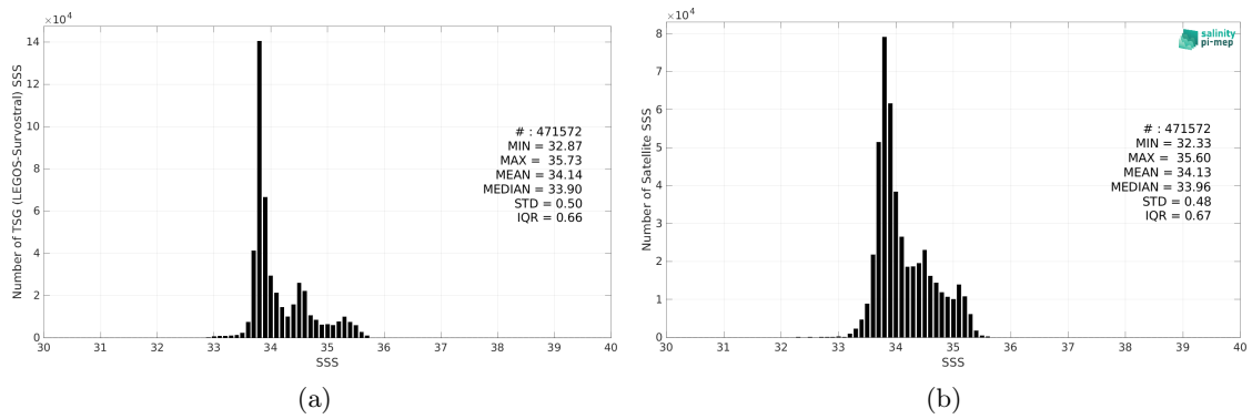
Figure 2: Histograms of SSS from TSG (LEGOS-Survostral) (a) and CCI SSS L4 Merged-OI v4.4 - 30-day running (ESA) (b) considering all match-up pairs per bins of 0.1 over the Global Ocean Pi-MEP region and for the full satellite product period.
