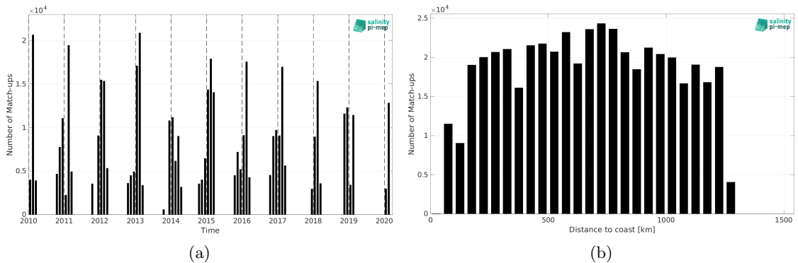
Figure 1: Number of match-ups between TSG (LEGOS-Survostral) and CCI SSS L4 Merged-OI v4.4 - 30-day running (ESA) SSS as a function of time (a) and as function of the distance to coast (b) over the Global Ocean Pi-MEP region and for the full satellite product period.
