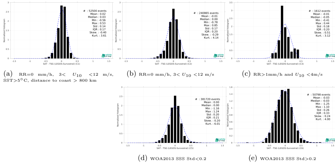
Figure 13: Normalized histogram of \Delta SSS (CCI SSS L4 Merged-OI v4.4 - 30-day running (ESA) - TSG (LEGOS-Survostral)) for 5 different subdatasets corresponding to: RR=0 mm/h, 3 < U_{10} < 12 m/s, SST>5°C, distance to coast > 800 km (a), RR=0 mm/h, 3 < U_{10} < 12 m/s (b), RR>1mm/h and U_{10} < 4 m/s (c), WOA2013 SSS Std<0.2 (d), WOA2013 SSS Std>0.2 (e).
