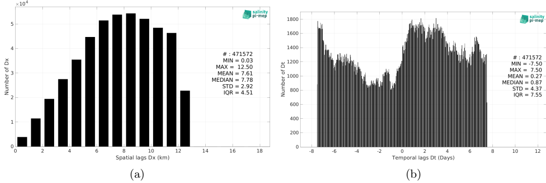
Figure 5: Histograms of the spatial (a) and temporal (b) lags between the location/time of the TSG (LEGOS-Survostral) measurement and the date of the corresponding CCI SSS L4 Merged-OI v4.4 - 30-day running (ESA) SSS pixel.
