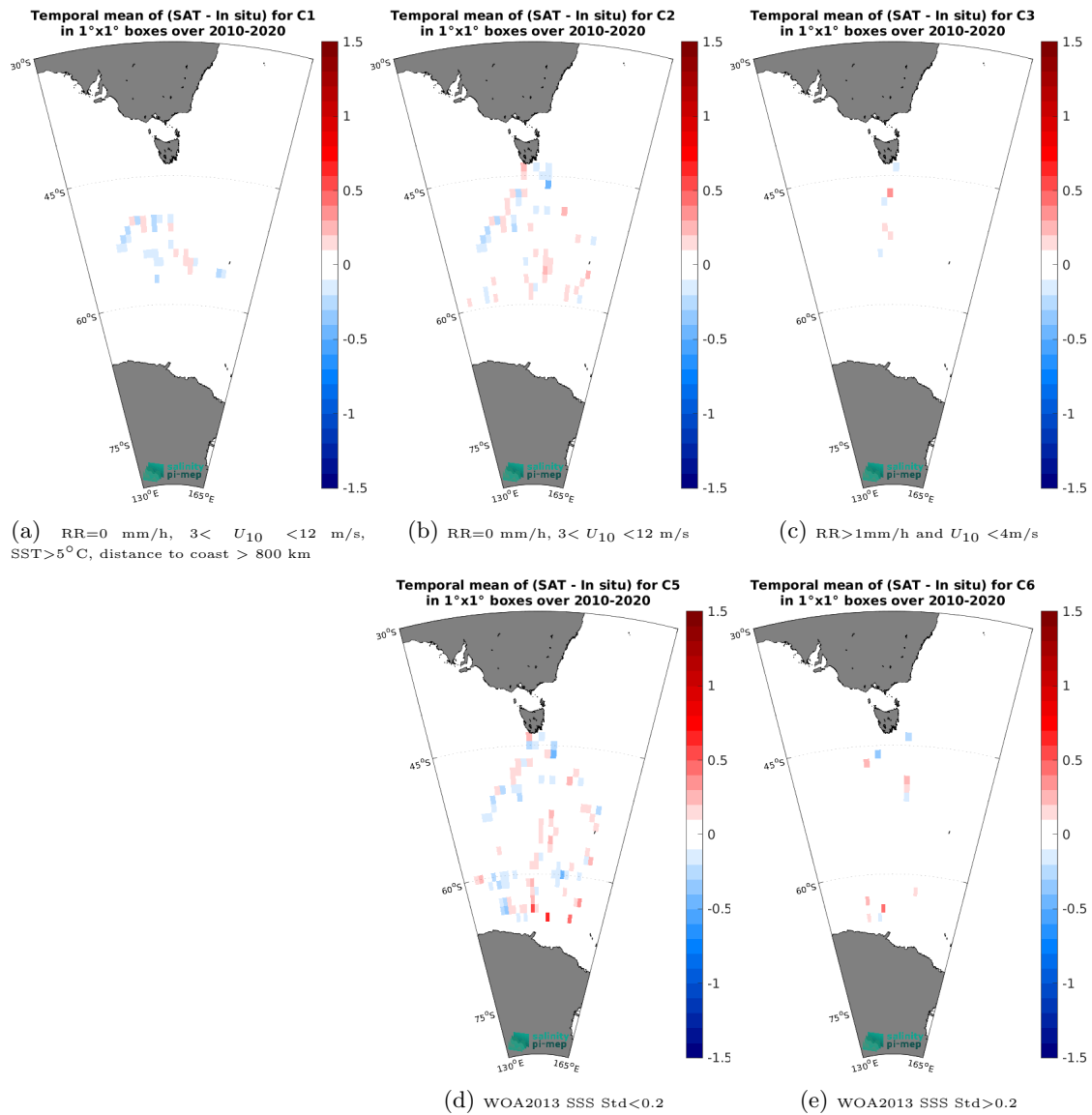
Figure 12: Temporal mean gridded over spatial boxes of size 1^\circ \times 1^\circ of \Delta\text{SSS} (CCI SSS L4 Merged-OI v4.4 - 30-day running (ESA) - TSG (LEGOS-Survostral)) for 5 different subdatasets corresponding to: RR=0 mm/h, 3 < U_{10} < 12 m/s, SST > 5^\circ\text{C} , distance to coast > 800 km (a), RR=0 mm/h, 3 < U_{10} < 12 m/s (b), RR > 1 mm/h and U_{10} < 4 m/s (c), WOA2013 SSS Std < 0.2 (d), WOA2013 SSS Std > 0.2 (e).
