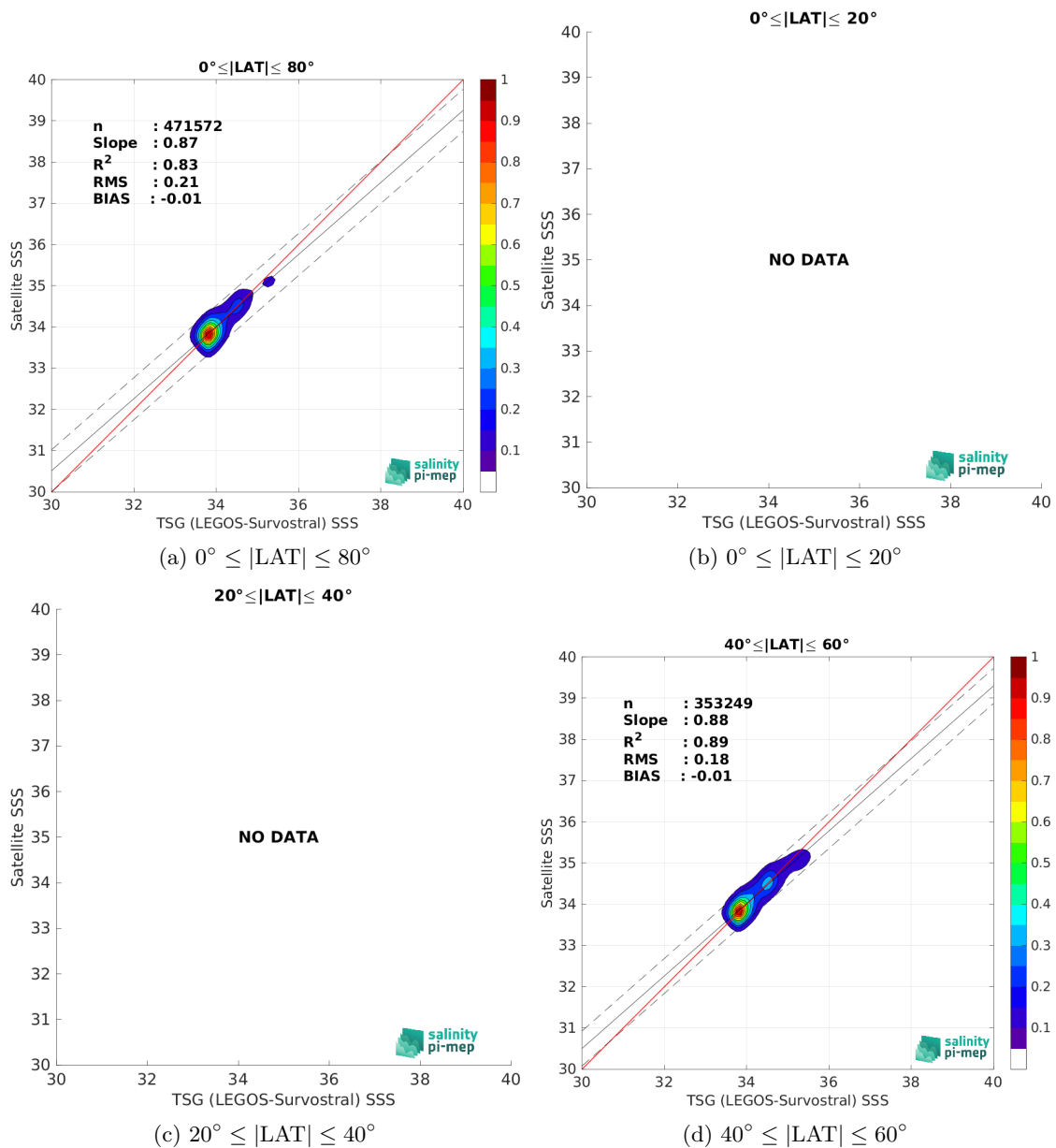
Figure 9: Contour maps of the concentration of CCI SSS L4 Merged-OI v4.4 - 30-day running (ESA) SSS (y-axis) versus TSG (LEGOS-Survostral) SSS (x-axis) at match-up pairs for different latitude bands. For each plot, the red line shows x=y . The black thin and dashed lines indicate a linear fit through the data cloud and the \pm 95\% confidence levels, respectively. The number match-up pairs n , the slope and R^2 coefficient of the linear fit, the root mean square (RMS) and the mean bias between satellite and in situ data are indicated for each latitude band in each plots.
