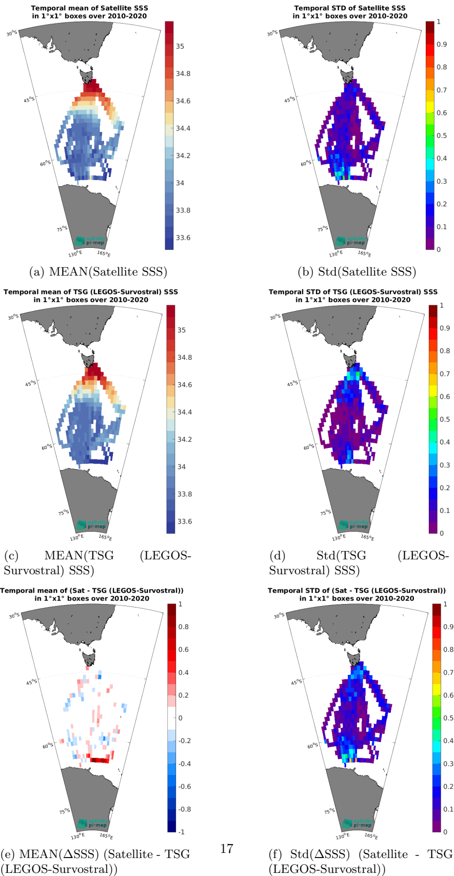
Figure 6: Temporal mean (left) and Std (right) of SSS from CCI SSS L4 Merged-OI v4.4 - 30-day running (ESA) (top), TSG (LEGOS-Survostral) (middle), and of \Delta SSS (Satellite - TSG (LEGOS-Survostral)). Only match-up pairs are used to generate these maps.
