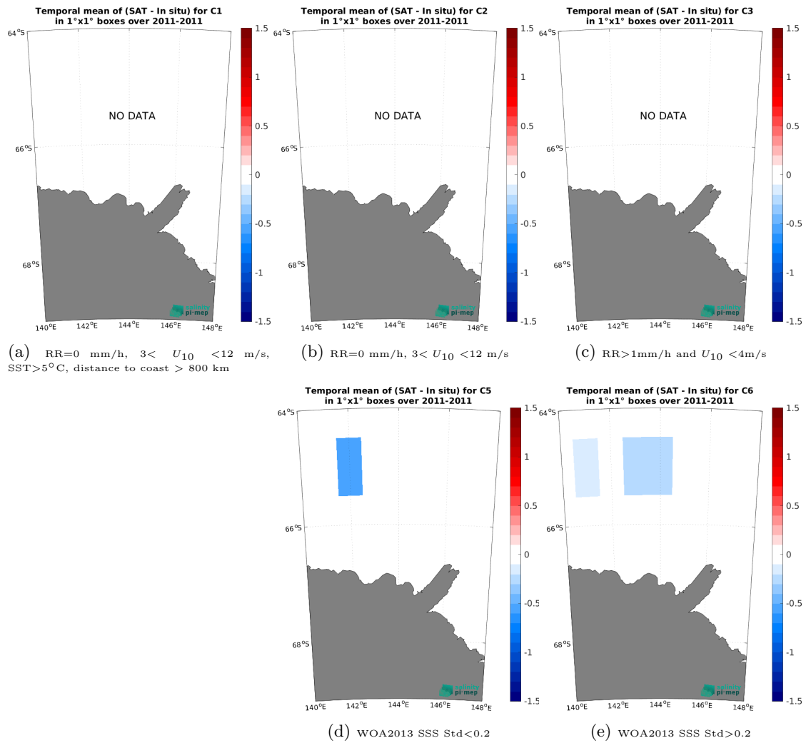
Figure 12: Temporal mean gridded over spatial boxes of size 1^\circ \times 1^\circ of \Delta SSS (CCI SSS L4 Merged-OI v4.4 - 30-day running (ESA) - TSG (LEGOS-Surv-Adel)) for 5 different subdatasets corresponding to: RR=0 mm/h, 3 < U_{10} < 12 m/s, SST>5°C, distance to coast > 800 km (a), RR=0 mm/h, 3 < U_{10} < 12 m/s (b), RR>1mm/h and U_{10} < 4 m/s (c), WOA2013 SSS Std<0.2 (d), WOA2013 SSS Std>0.2 (e).
