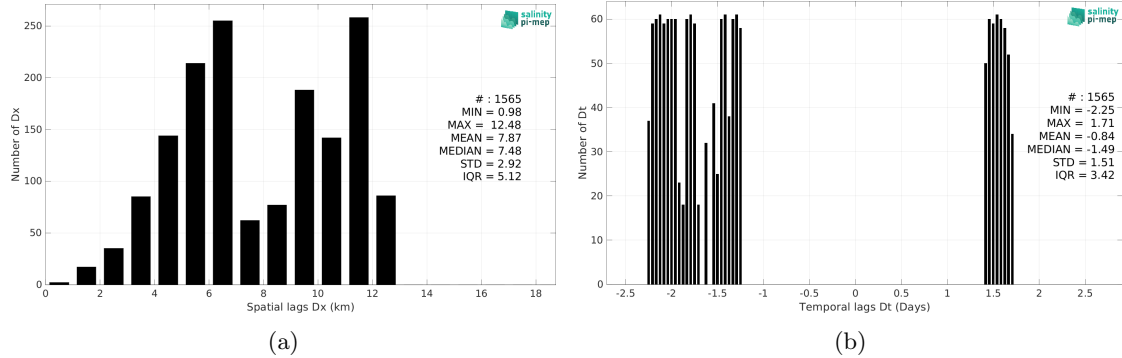
Figure 5: Histograms of the spatial (a) and temporal (b) lags between the location/time of the TSG (LEGOS-Surv-Adel) measurement and the date of the corresponding CCI SSS L4 Merged-OI v4.4 - 30-day running (ESA) SSS pixel.
