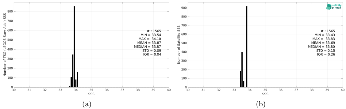
Figure 2: Histograms of SSS from TSG (LEGOS-Surv-Adel) (a) and CCI SSS L4 Merged-OI v4.4 - 30-day running (ESA) (b) considering all match-up pairs per bins of 0.1 over the Global Ocean Pi-MEP region and for the full satellite product period.
