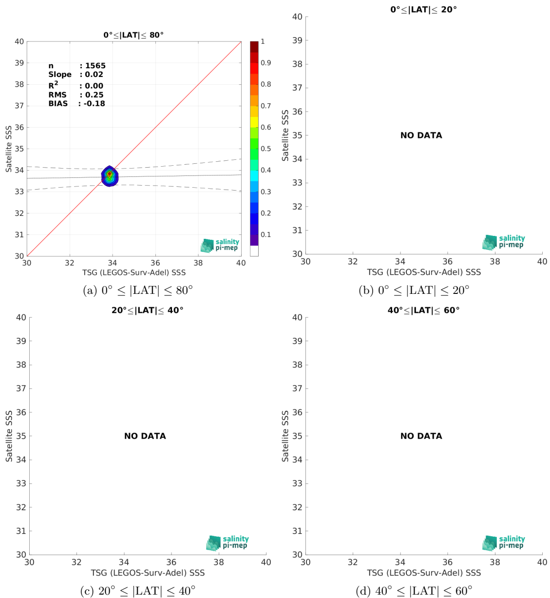
Figure 9: Contour maps of the concentration of CCI SSS L4 Merged-OI v4.4 - 30-day running (ESA) SSS (y-axis) versus TSG (LEGOS-Surv-Adel) SSS (x-axis) at match-up pairs for different latitude bands. For each plot, the red line shows x=y . The black thin and dashed lines indicate a linear fit through the data cloud and the \pm 95\% confidence levels, respectively. The number match-up pairs n , the slope and R^2 coefficient of the linear fit, the root mean square (RMS) and the mean bias between satellite and in situ data are indicated for each latitude band in each plots.
