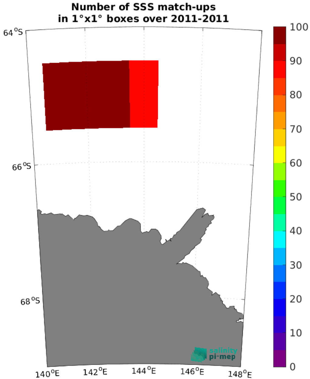
Figure 4: Number of SSS match-ups between TSG (LEGOS-Surv-Adel) SSS and the CCI SSS L4 Merged-OI v4.4 - 30-day running (ESA) SSS product for the Global Ocean Pi-MEP region over 1^\circ \times 1^\circ boxes and for the full satellite product period.
