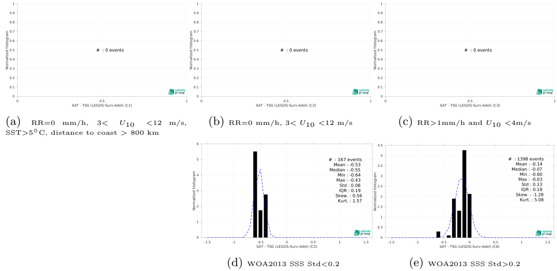
Figure 13: Normalized histogram of \Delta SSS (CCI SSS L4 Merged-OI v4.4 - 30-day running (ESA) - TSG (LEGOS-Surv-Adel)) for 5 different subdatasets corresponding to: RR=0 mm/h, 3 < U_{10} < 12 m/s, SST>5°C, distance to coast > 800 km (a), RR=0 mm/h, 3 < U_{10} < 12 m/s (b), RR>1mm/h and U_{10} < 4 m/s (c), WOA2013 SSS Std<0.2 (d), WOA2013 SSS Std>0.2 (e).
