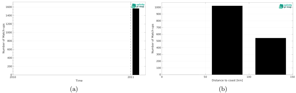
Figure 1: Number of match-ups between TSG (LEGOS-Surv-Adel) and CCI SSS L4 Merged-OI v4.4 - 30-day running (ESA) SSS as a function of time (a) and as function of the distance to coast (b) over the Global Ocean Pi-MEP region and for the full satellite product period.
