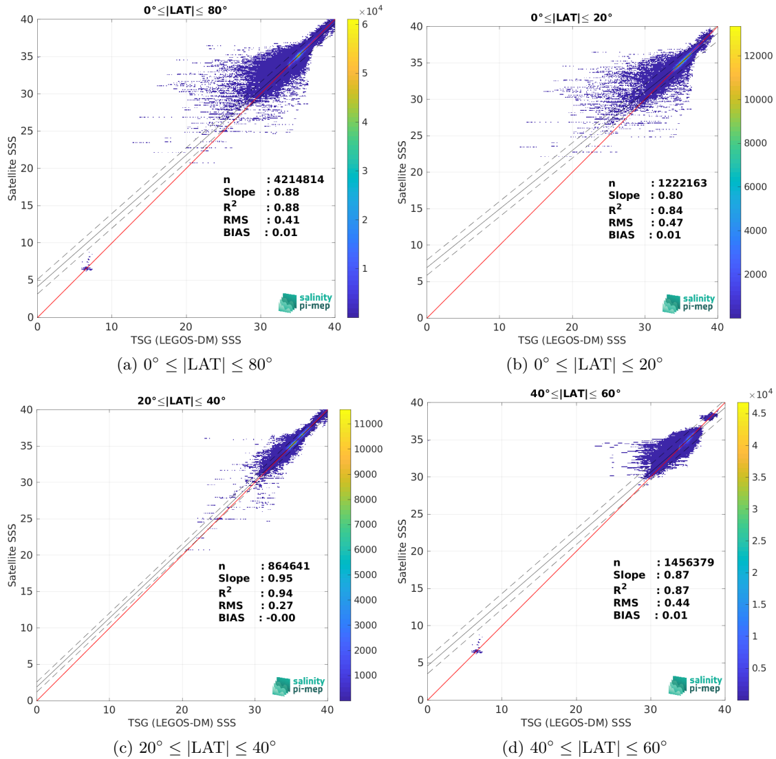
Figure 9: Contour maps of the concentration of CCI SSS L4 Merged-OI v4.4 - 30-day running (ESA) SSS (y-axis) versus TSG (LEGOS-DM) SSS (x-axis) at match-up pairs for different latitude bands. For each plot, the red line shows x=y . The black thin and dashed lines indicate a linear fit through the data cloud and the \pm 95\% confidence levels, respectively. The number match-up pairs n , the slope and R^2 coefficient of the linear fit, the root mean square (RMS) and the mean bias between satellite and in situ data are indicated for each latitude band in each plots.
