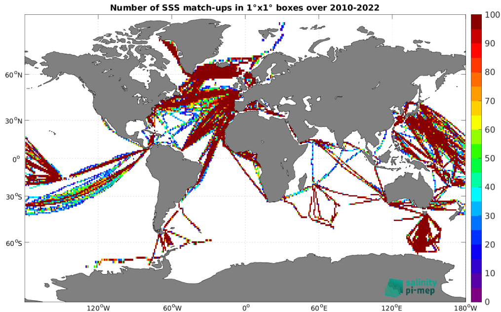
Figure 4: Number of SSS match-ups between TSG (LEGOS-DM) SSS and the CCI SSS L4 Merged-OI v4.4 - 30-day running (ESA) SSS product for the Global Ocean Pi-MEP region over 1^\circ \times 1^\circ boxes and for the full satellite product period.
