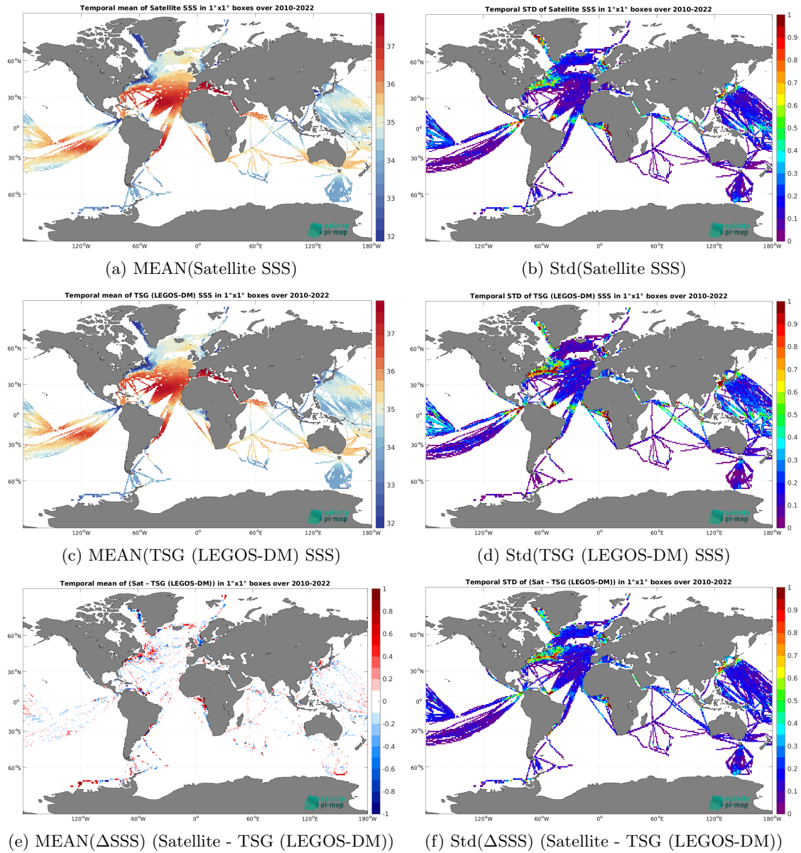
Figure 6: Temporal mean (left) and Std (right) of SSS from CCI SSS L4 Merged-OI v4.4 - 30-day running (ESA) (top), TSG (LEGOS-DM) (middle), and of \Delta SSS (Satellite - TSG (LEGOS-DM)). Only match-up pairs are used to generate these maps.
