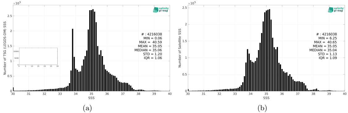
Figure 2: Histograms of SSS from TSG (LEGOS-DM) (a) and CCI SSS L4 Merged-OI v4.4 - 30-day running (ESA) (b) considering all match-up pairs per bins of 0.1 over the Global Ocean Pi-MEP region and for the full satellite product period.
