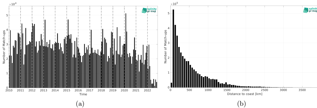
Figure 1: Number of match-ups between TSG (LEGOS-DM) and CCI SSS L4 Merged-OI v4.4 - 30-day running (ESA) SSS as a function of time (a) and as function of the distance to coast (b) over the Global Ocean Pi-MEP region and for the full satellite product period.
