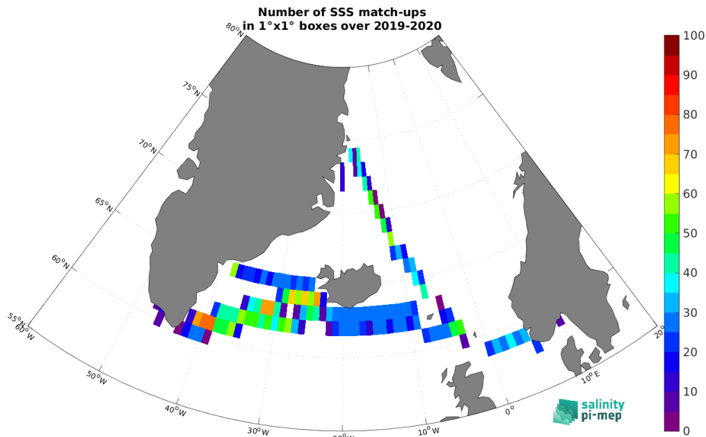
Figure 4: Number of SSS match-ups between TSG (Lauge-Koch) SSS and the CCI SSS L4 Merged-OI v4.4 - 30-day running (ESA) SSS product for the Global Ocean Pi-MEP region over 1^\circ \times 1^\circ boxes and for the full satellite product period.
