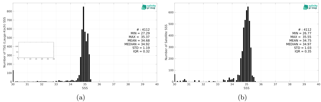
Figure 2: Histograms of SSS from TSG (Lauge-Koch) (a) and CCI SSS L4 Merged-OI v4.4 - 30-day running (ESA) (b) considering all match-up pairs per bins of 0.1 over the Global Ocean Pi-MEP region and for the full satellite product period.
