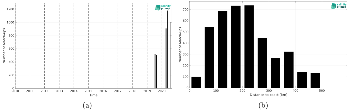
Figure 1: Number of match-ups between TSG (Lauge-Koch) and CCI SSS L4 Merged-OI v4.4 - 30-day running (ESA) SSS as a function of time (a) and as function of the distance to coast (b) over the Global Ocean Pi-MEP region and for the full satellite product period.
