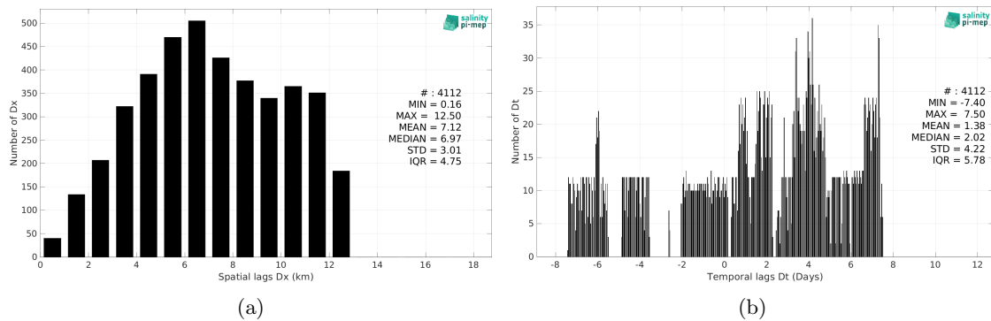
Figure 5: Histograms of the spatial (a) and temporal (b) lags between the location/time of the TSG (Lauge-Koch) measurement and the date of the corresponding CCI SSS L4 Merged-OI v4.4 - 30-day running (ESA) SSS pixel.
