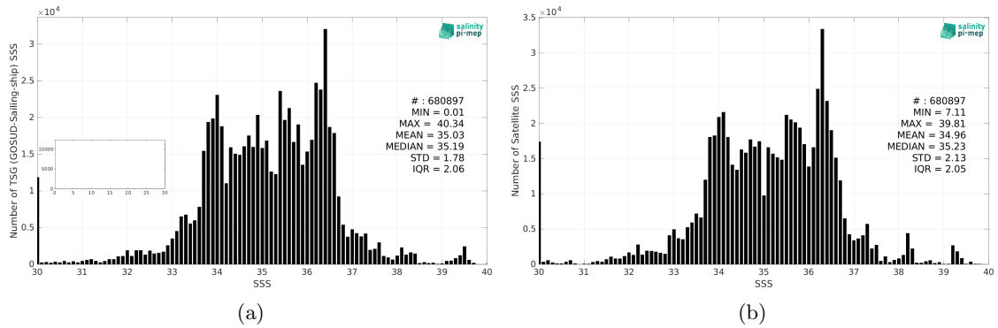
Figure 2: Histograms of SSS from TSG (GOSUD-Sailing-ship) (a) and CCI SSS L4 Merged-OI v4.4 - 30-day running (ESA) (b) considering all match-up pairs per bins of 0.1 over the Global Ocean Pi-MEP region and for the full satellite product period.
