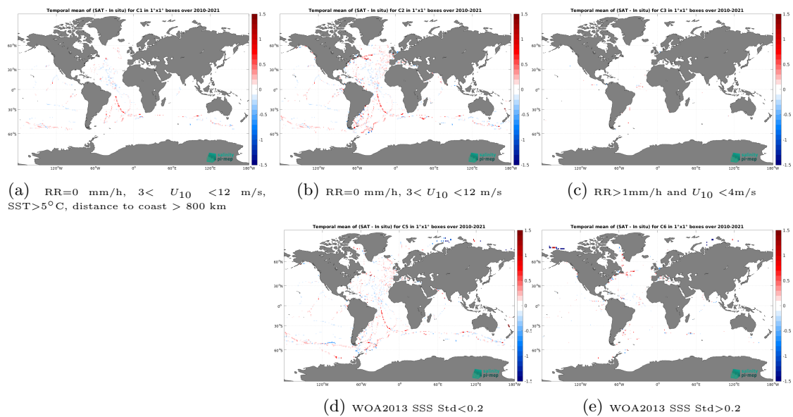
Figure 12: Temporal mean gridded over spatial boxes of size 1^\circ \times 1^\circ of \Delta SSS (CCI SSS L4 Merged-OI v4.4 - 30-day running (ESA) - TSG (GOSUD-Sailing-ship)) for 5 different subdatasets corresponding to:RR=0 mm/h, 3 < U_{10} < 12 m/s, SST >5^\circ C, distance to coast > 800 km (a), RR=0 mm/h, 3 < U_{10} < 12 m/s (b), RR >1 mm/h and U_{10} < 4 m/s (c), WOA2013 SSS Std <0.2 (d), WOA2013 SSS Std >0.2 (e).
