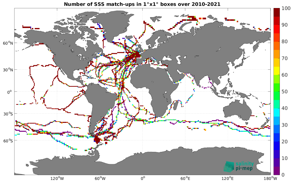
Figure 4: Number of SSS match-ups between TSG (GOSUD-Sailing-ship) SSS and the CCI SSS L4 Merged-OI v4.4 - 30-day running (ESA) SSS product for the Global Ocean Pi-MEP region over 1°×1° boxes and for the full satellite product period.
