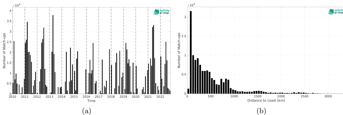
Figure 1: Number of match-ups between TSG (CSIC-UTM) and CCI SSS L4 Merged-OI v4.4 - 30-day running (ESA) SSS as a function of time (a) and as function of the distance to coast (b) over the Global Ocean Pi-MEP region and for the full satellite product period.
