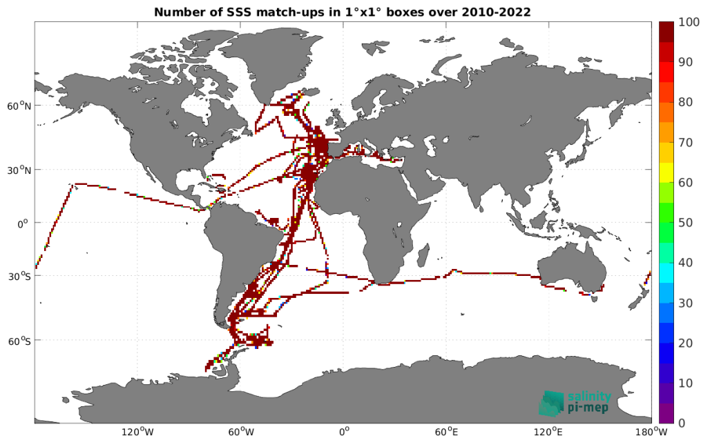
Figure 4: Number of SSS match-ups between TSG (CSIC-UTM) SSS and the CCI SSS L4 Merged-OI v4.4 - 30-day running (ESA) SSS product for the Global Ocean Pi-MEP region over 1^\circ \times 1^\circ boxes and for the full satellite product period.
