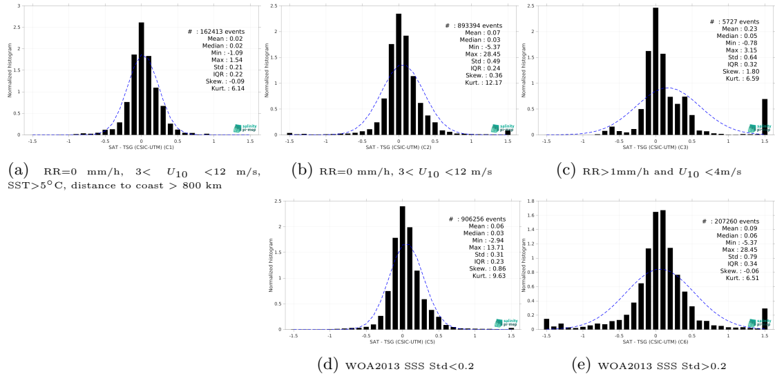
Figure 13: Normalized histogram of \Delta\text{SSS} (CCI SSS L4 Merged-OI v4.4 - 30-day running (ESA) - TSG (CSIC-UTM)) for 5 different subdatasets corresponding to: RR=0 mm/h, 3 < U_{10} < 12 m/s, SST>5°C, distance to coast > 800 km (a), RR=0 mm/h, 3 < U_{10} < 12 m/s (b), RR>1mm/h and U_{10} < 4 m/s (c), WOA2013 SSS Std<0.2 (d), WOA2013 SSS Std>0.2 (e).
