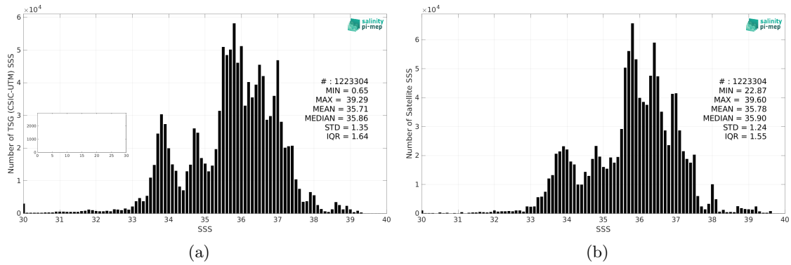
Figure 2: Histograms of SSS from TSG (CSIC-UTM) (a) and CCI SSS L4 Merged-OI v4.4 - 30-day running (ESA) (b) considering all match-up pairs per bins of 0.1 over the Global Ocean Pi-MEP region and for the full satellite product period.
