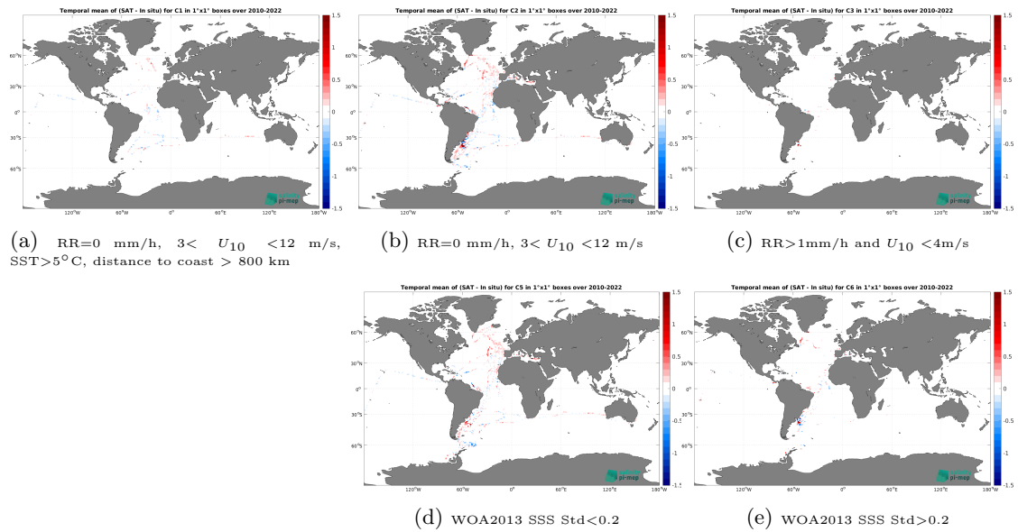
Figure 12: Temporal mean gridded over spatial boxes of size 1^\circ \times 1^\circ of \Delta SSS (CCI SSS L4 Merged-OI v4.4 - 30-day running (ESA) - TSG (CSIC-UTM)) for 5 different subdatasets corresponding to:RR=0 mm/h, 3 < U_{10} < 12 m/s, SST > 5^\circ\text{C} , distance to coast > 800 km (a), RR=0 mm/h, 3 < U_{10} < 12 m/s (b), RR > 1 mm/h and U_{10} < 4 m/s (c), WOA2013 SSS Std < 0.2 (d), WOA2013 SSS Std > 0.2 (e).
