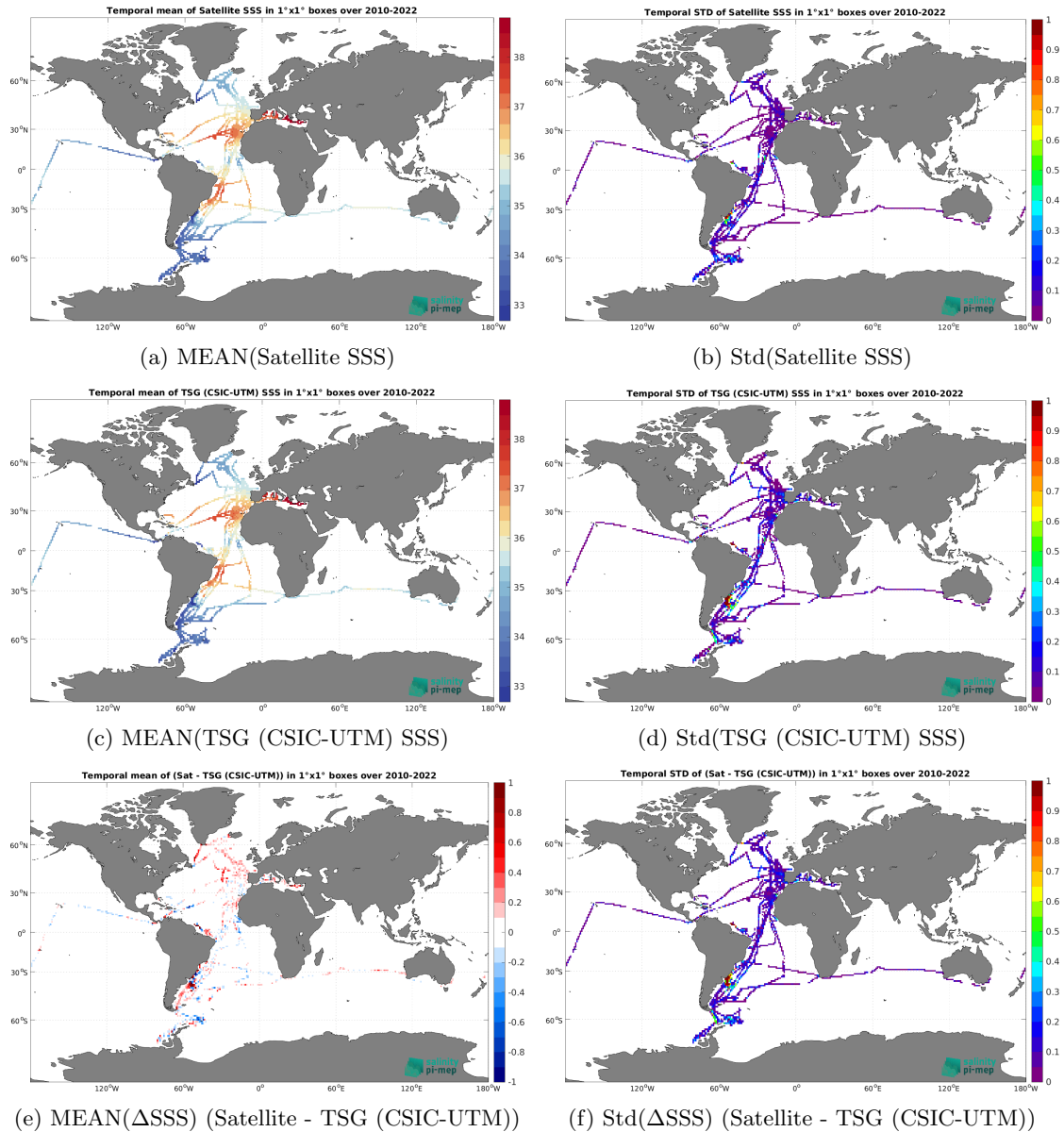
Figure 6: Temporal mean (left) and Std (right) of SSS from CCI SSS L4 Merged-OI v4.4 - 30-day running (ESA) (top), TSG (CSIC-UTM) (middle), and of \Delta SSS (Satellite - TSG (CSIC-UTM)). Only match-up pairs are used to generate these maps.
