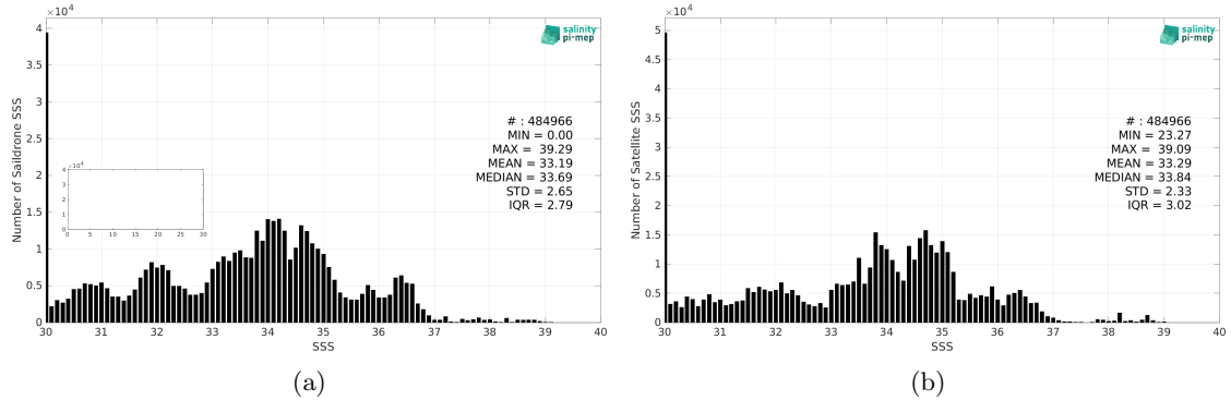
Figure 2: Histograms of SSS from Saildrone (a) and CCI SSS L4 Merged-OI v4.4 - 30-day running (ESA) (b) considering all match-up pairs per bins of 0.1 over the Global Ocean Pi-MEP region and for the full satellite product period.
