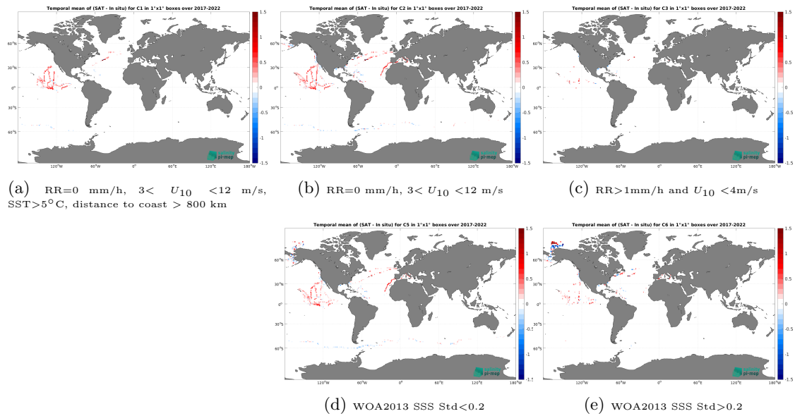
Figure 12: Temporal mean gridded over spatial boxes of size 1^\circ \times 1^\circ of \Delta\text{SSS} (CCI SSS L4 Merged-OI v4.4 - 30-day running (ESA) - Saildrone) for 5 different subdatasets corresponding to:RR=0 mm/h, 3 < U_{10} < 12 m/s, SST >5^\circ\text{C} , distance to coast > 800 km (a), RR=0 mm/h, 3 < U_{10} < 12 m/s (b), RR >1 mm/h and U_{10} < 4 m/s (c), WOA2013 SSS Std <0.2 (d), WOA2013 SSS Std >0.2 (e).
