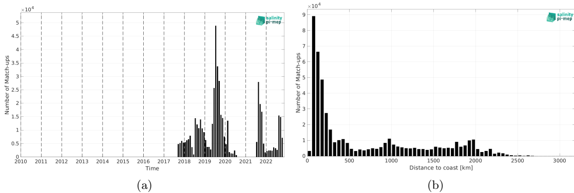
Figure 1: Number of match-ups between Saildrone and CCI SSS L4 Merged-OI v4.4 - 30-day running (ESA) SSS as a function of time (a) and as function of the distance to coast (b) over the Global Ocean Pi-MEP region and for the full satellite product period.
