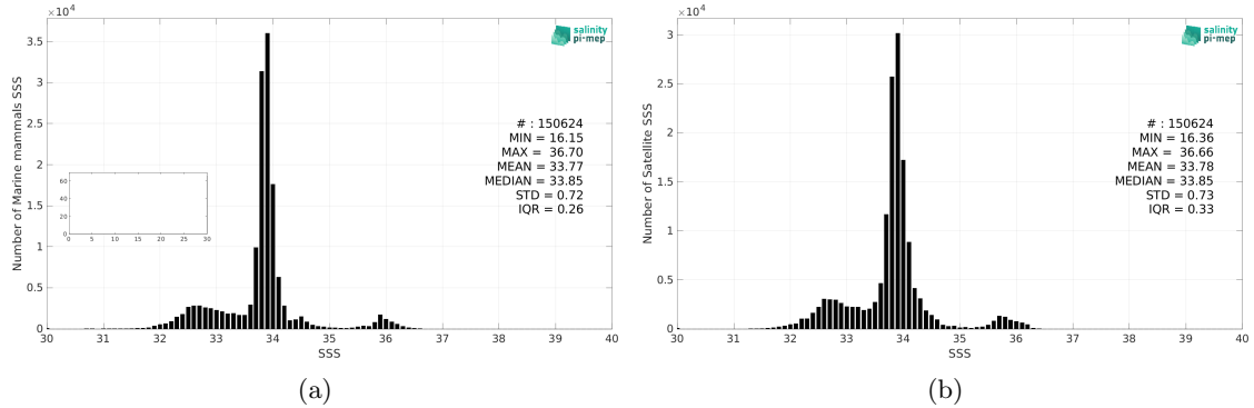
Figure 2: Histograms of SSS from Marine mammals (a) and CCI SSS L4 Merged-OI v4.4 - 30-day running (ESA) (b) considering all match-up pairs per bins of 0.1 over the Global Ocean Pi-MEP region and for the full satellite product period.
