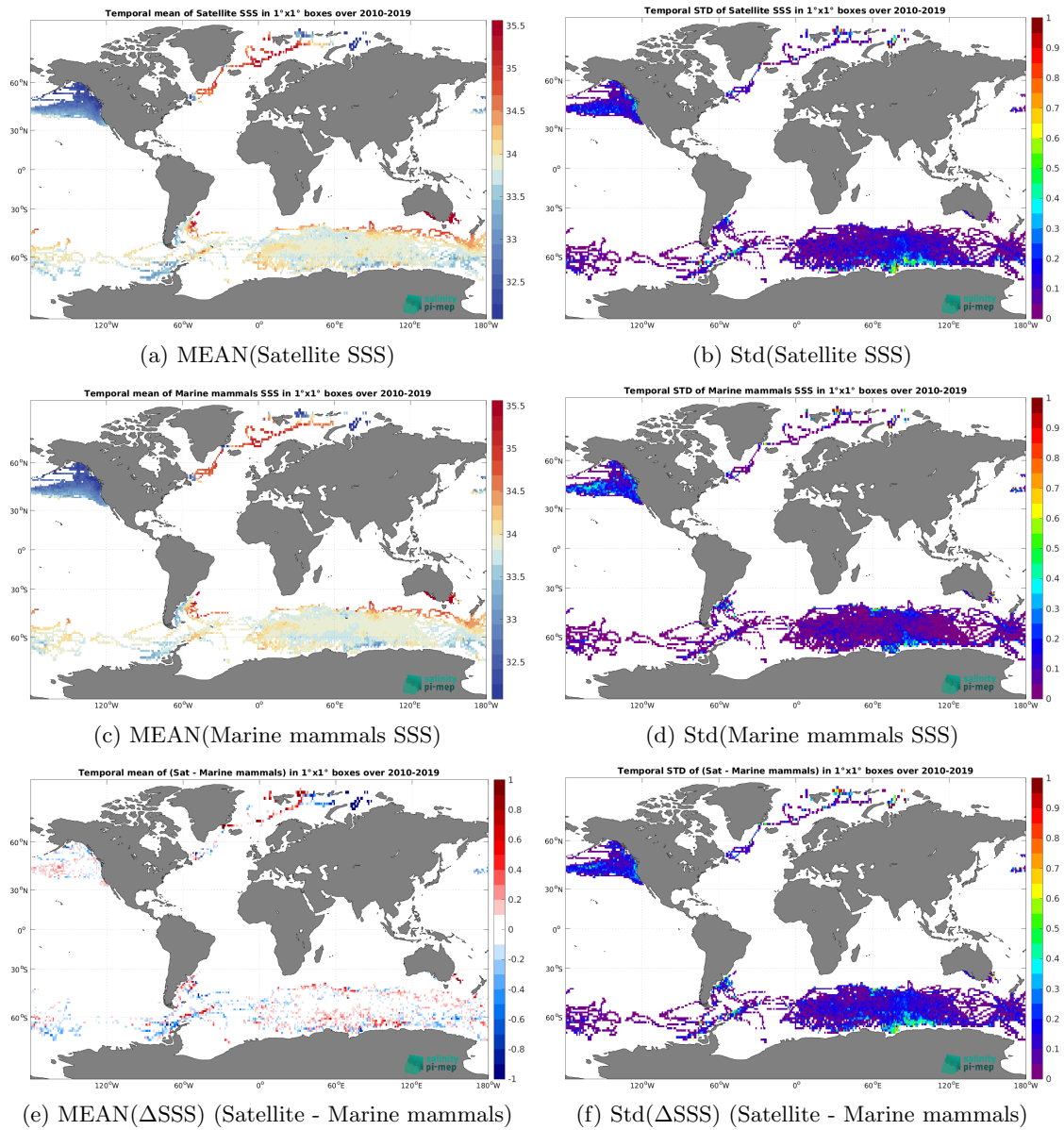
Figure 6: Temporal mean (left) and Std (right) of SSS from CCI SSS L4 Merged-OI v4.4 - 30-day running (ESA) (top), Marine mammals (middle), and of \Delta SSS (Satellite - Marine mammals). Only match-up pairs are used to generate these maps.
