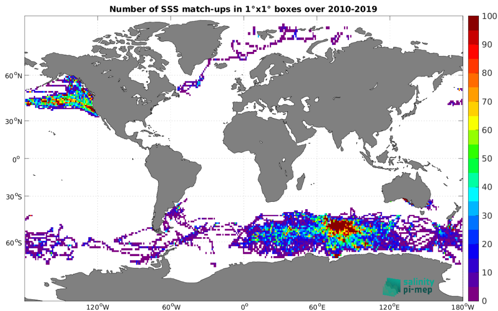
Figure 4: Number of SSS match-ups between Marine mammals SSS and the CCI SSS L4 Merged-OI v4.4 - 30-day running (ESA) SSS product for the Global Ocean Pi-MEP region over 1^\circ \times 1^\circ boxes and for the full satellite product period.
