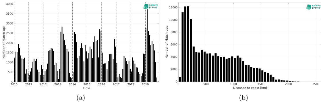
Figure 1: Number of match-ups between Marine mammals and CCI SSS L4 Merged-OI v4.4 - 30-day running (ESA) SSS as a function of time (a) and as function of the distance to coast (b) over the Global Ocean Pi-MEP region and for the full satellite product period.
