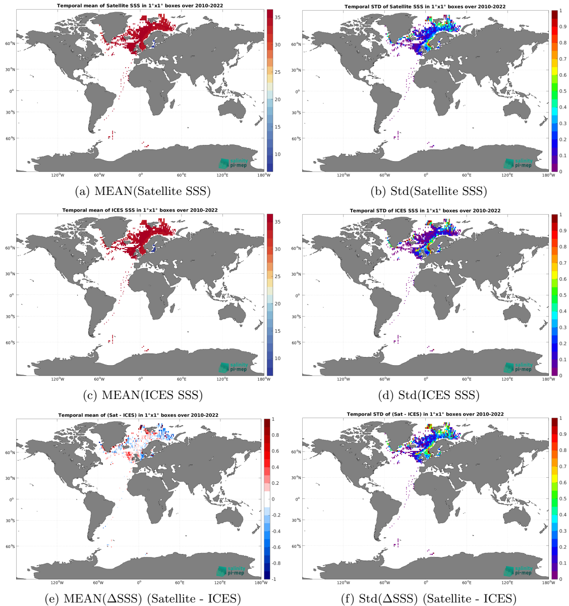
Figure 6: Temporal mean (left) and Std (right) of SSS from CCI SSS L4 Merged-OI v4.4 - 30-day running (ESA) (top), ICES (middle), and of \Delta SSS (Satellite - ICES). Only match-up pairs are used to generate these maps.
