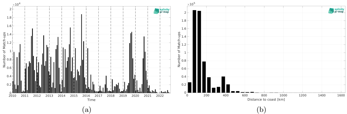
Figure 1: Number of match-ups between ICES and CCI SSS L4 Merged-OI v4.4 - 30-day running (ESA) SSS as a function of time (a) and as function of the distance to coast (b) over the Global Ocean Pi-MEP region and for the full satellite product period.
