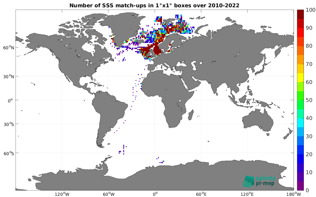
Figure 4: Number of SSS match-ups between ICES SSS and the CCI SSS L4 Merged-OI v4.4 - 30-day running (ESA) SSS product for the Global Ocean Pi-MEP region over 1^\circ \times 1^\circ boxes and for the full satellite product period.
