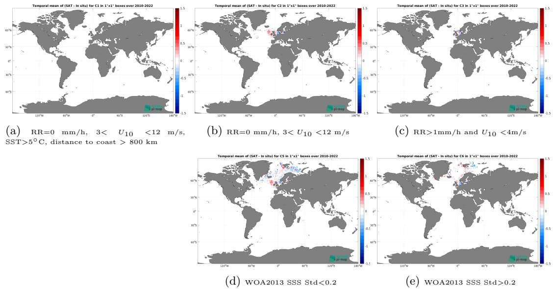
Figure 12: Temporal mean gridded over spatial boxes of size 1^\circ \times 1^\circ of \Delta\text{SSS} (CCI SSS L4 Merged-OI v4.4 - 30-day running (ESA) - ICES) for 5 different subdatasets corresponding to:RR=0 mm/h, 3 < U_{10} < 12 m/s, SST >5^\circ\text{C} , distance to coast > 800 km (a), RR=0 mm/h, 3 < U_{10} < 12 m/s (b), RR >1 mm/h and U_{10} < 4 m/s (c), WOA2013 SSS Std <0.2 (d), WOA2013 SSS Std >0.2 (e).
