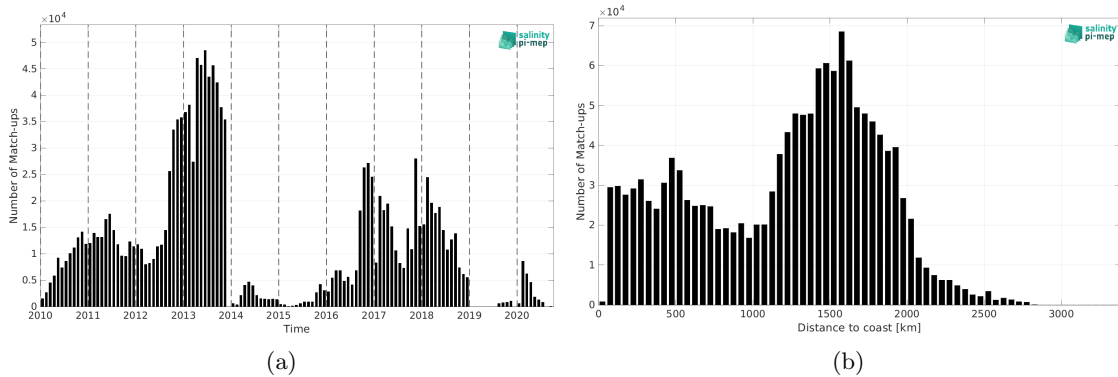
Figure 1: Number of match-ups between Surface drifters and CCI SSS L4 Merged-OI v4.4 - 30-day running (ESA) SSS as a function of time (a) and as function of the distance to coast (b) over the Global Ocean Pi-MEP region and for the full satellite product period.
