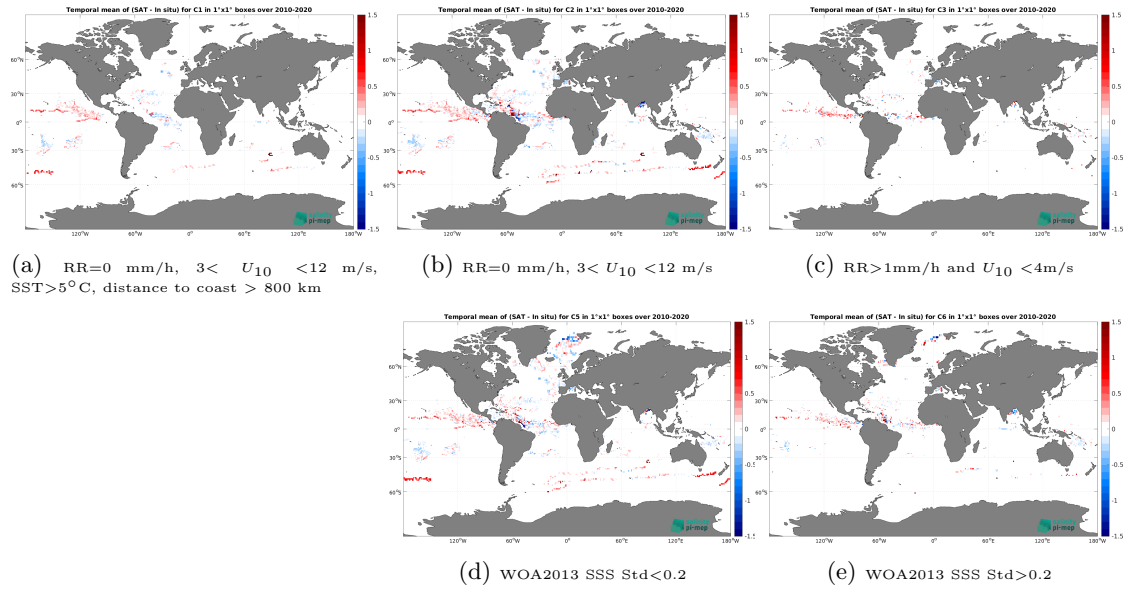
Figure 11: Temporal mean gridded over spatial boxes of size 1^\circ \times 1^\circ of \Delta SSS (CCI SSS L4 Merged-OI v4.4 - 30-day running (ESA) - Surface drifters) for 5 different subdatasets corresponding to:RR=0 mm/h, 3 < U_{10} < 12 m/s, SST >5^\circ C, distance to coast > 800 km (a), RR=0 mm/h, 3 < U_{10} < 12 m/s (b), RR >1 mm/h and U_{10} < 4 m/s (c), WOA2013 SSS Std <0.2 (d), WOA2013 SSS Std >0.2 (e).
