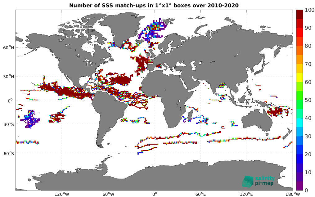
Figure 3: Number of SSS match-ups between Surface drifters SSS and the CCI SSS L4 Merged-OI v4.4 - 30-day running (ESA) SSS product for the Global Ocean Pi-MEP region over 1^\circ \times 1^\circ boxes and for the full satellite product period.
