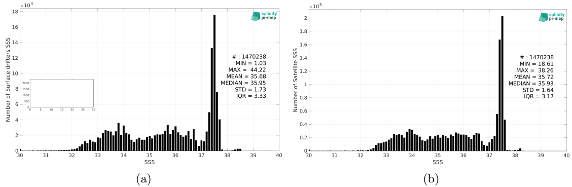
Figure 2: Histograms of SSS from Surface drifters (a) and CCI SSS L4 Merged-OI v4.4 - 30-day running (ESA) (b) considering all match-up pairs per bins of 0.1 over the Global Ocean Pi-MEP region and for the full satellite product period.
