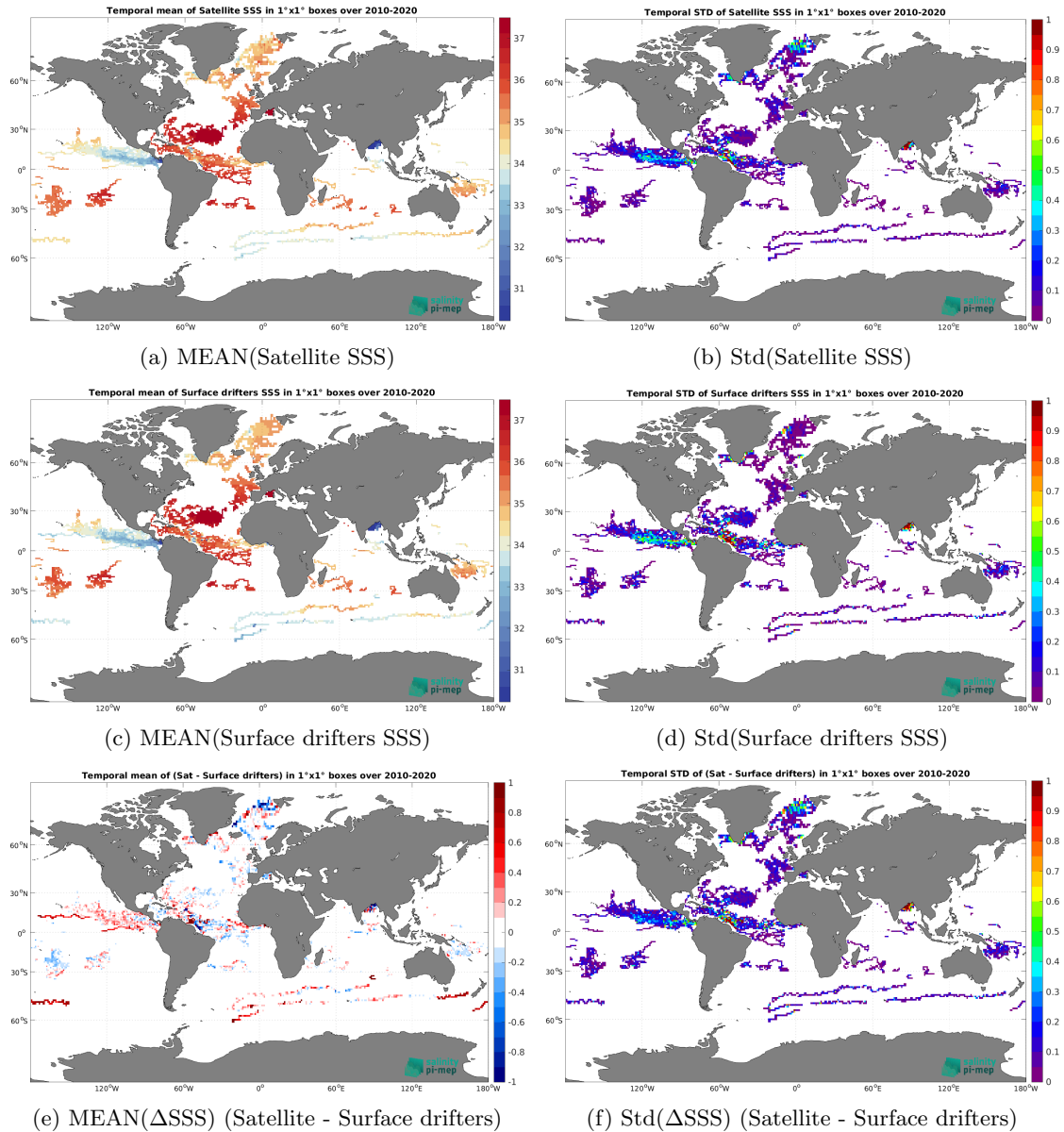
Figure 5: Temporal mean (left) and Std (right) of SSS from CCI SSS L4 Merged-OI v4.4 - 30-day running (ESA) (top), Surface drifters (middle), and of \Delta SSS (Satellite - Surface drifters). Only match-up pairs are used to generate these maps.
