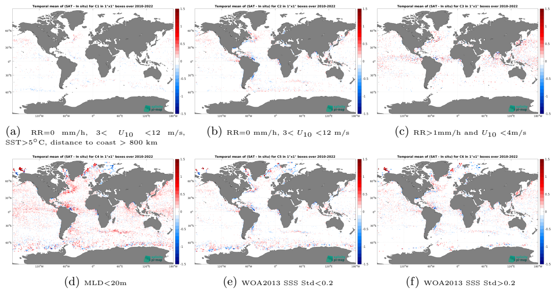
Figure 12: Temporal mean gridded over spatial boxes of size 1^\circ \times 1^\circ of \Delta SSS (CCI SSS L4 Merged-OI v4.4 - 30-day running (ESA) - Argo) for 6 different subdatasets corresponding to:RR=0 mm/h, 3 < U_{10} < 12 m/s, SST >5^\circ C, distance to coast > 800 km (a), RR=0 mm/h, 3 < U_{10} < 12 m/s (b), RR >1 mm/h and U_{10} < 4 m/s (c),MLD <20 m (d),WOA2013 SSS Std <0.2 (e),WOA2013 SSS Std >0.2 (f).
