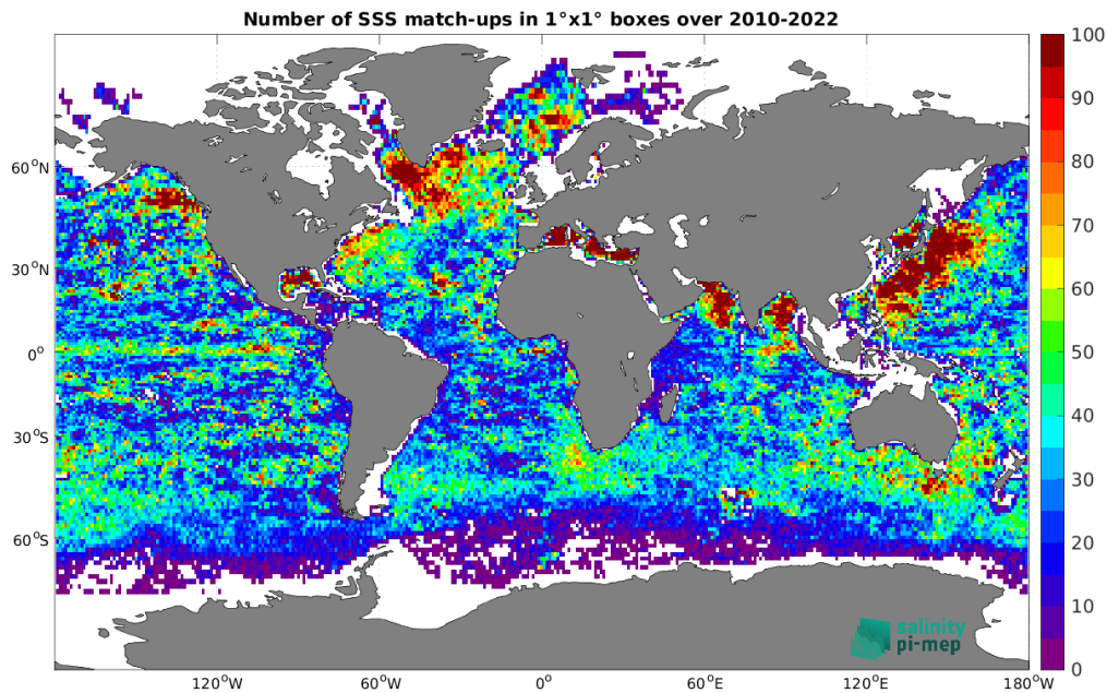
Figure 4: Number of SSS match-ups between Argo SSS and the CCI SSS L4 Merged-OI v4.4 - 30-day running (ESA) SSS product for the Global Ocean Pi-MEP region over 1^\circ \times 1^\circ boxes and for the full satellite product period.
