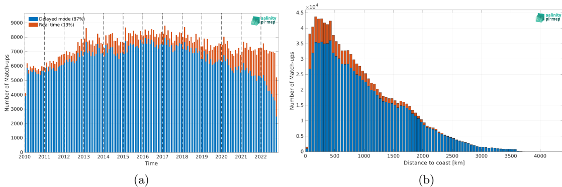
Figure 1: Number of match-ups between Argo and CCI SSS L4 Merged-OI v4.4 - 30-day running (ESA) SSS as a function of time (a) and as function of the distance to coast (b) over the Global Ocean Pi-MEP region and for the full satellite product period.
