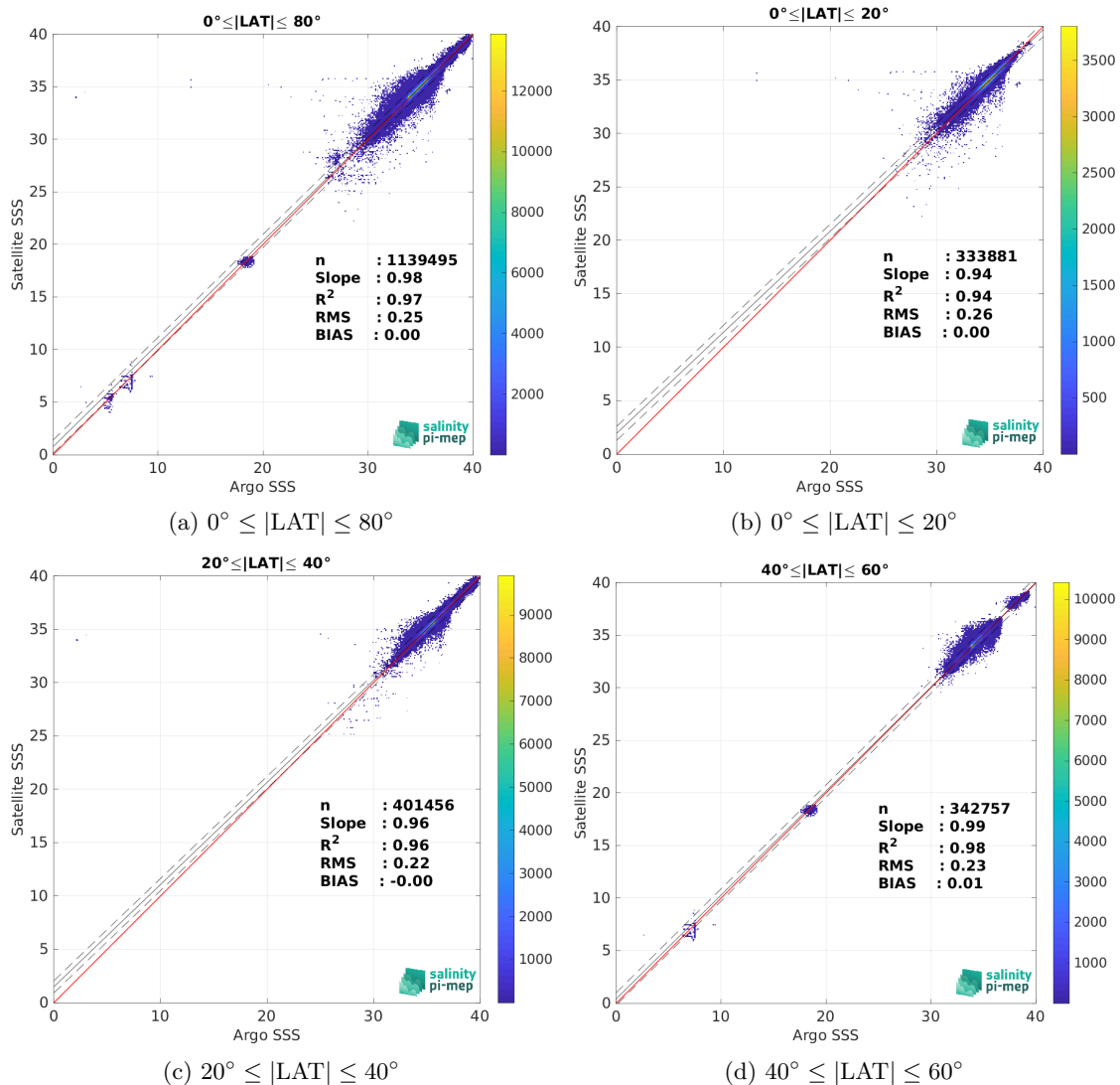
Figure 9: Contour maps of the concentration of CCI SSS L4 Merged-OI v4.4 - 30-day running (ESA) SSS (y-axis) versus Argo SSS (x-axis) at match-up pairs for different latitude bands. For each plot, the red line shows x=y . The black thin and dashed lines indicate a linear fit through the data cloud and the \pm 95\% confidence levels, respectively. The number match-up pairs n , the slope and R^2 coefficient of the linear fit, the root mean square (RMS) and the mean bias between satellite and in situ data are indicated for each latitude band in each plot.
