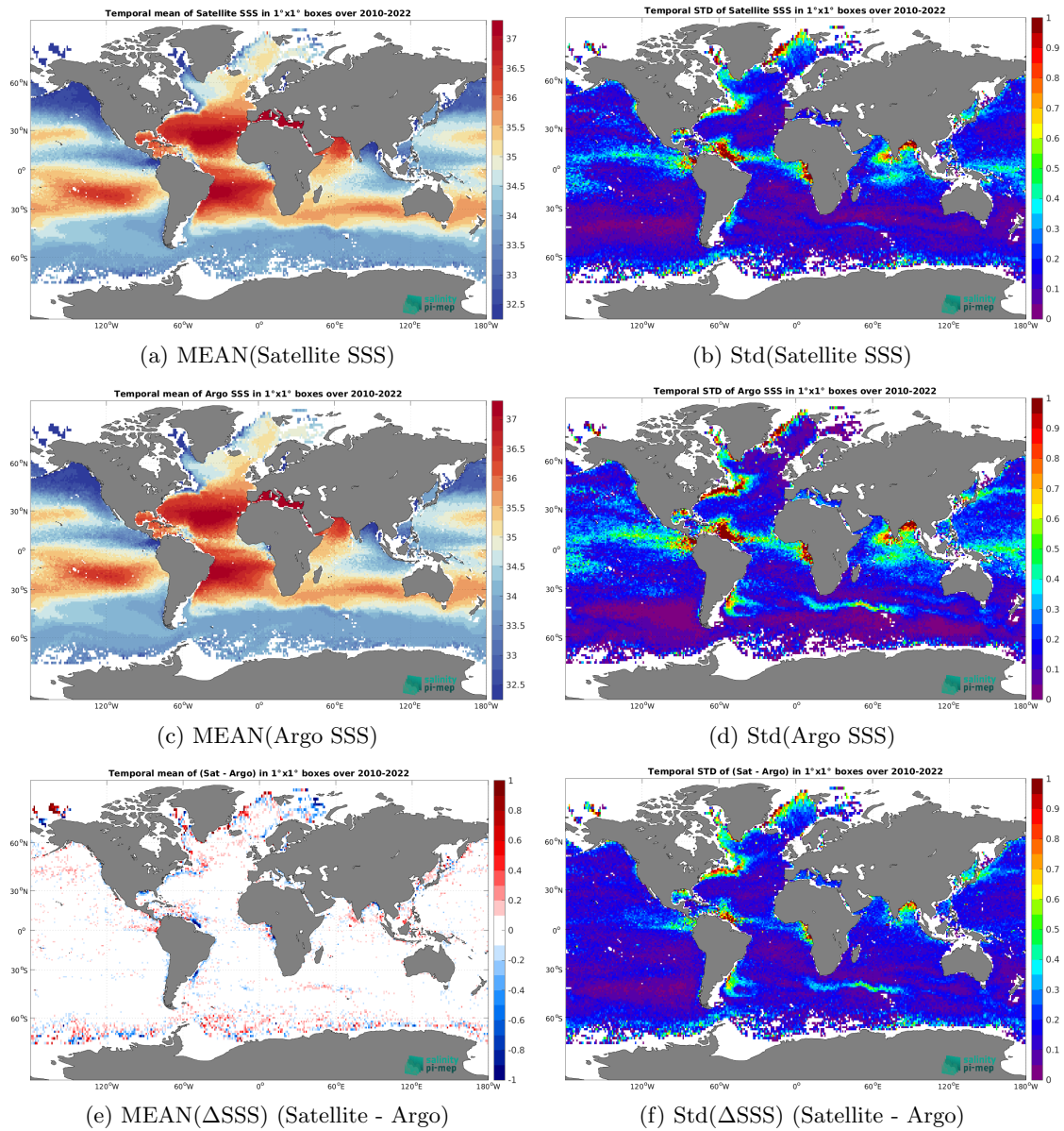
Figure 6: Temporal mean (left) and Std (right) of SSS from CCI SSS L4 Merged-OI v4.4 - 30-day running (ESA) (top), Argo (middle), and of \Delta SSS (Satellite - Argo). Only match-up pairs are used to generate these maps.
