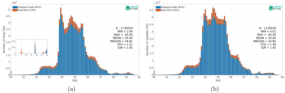
Figure 2: Histograms of SSS from Argo (a) and CCI SSS L4 Merged-OI v4.4 - 30-day running (ESA) (b) considering all match-up pairs per bins of 0.1 over the Global Ocean Pi-MEP region and for the full satellite product period.
