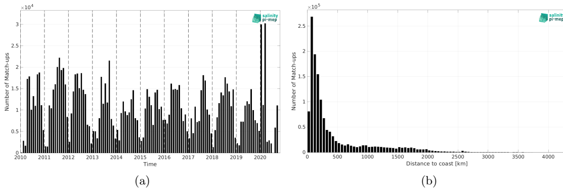
Figure 1: Number of match-ups between TSG (SAMOS) and CCI SSS L4 Merged-OI v3.2 - 7-day running (ESA) SSS as a function of time (a) and as function of the distance to coast (b) over the Global Ocean Pi-MEP region and for the full satellite product period.
