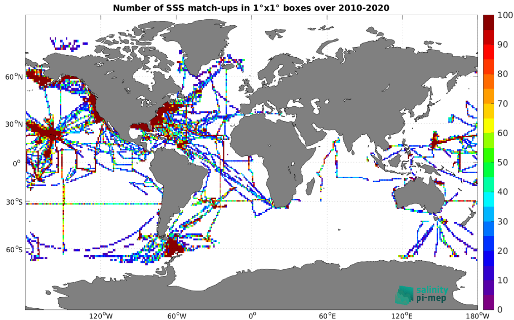
Figure 4: Number of SSS match-ups between TSG (SAMOS) SSS and the CCI SSS L4 Merged-OI v3.2 - 7-day running (ESA) SSS product for the Global Ocean Pi-MEP region over 1^\circ \times 1^\circ boxes and for the full satellite product period.
