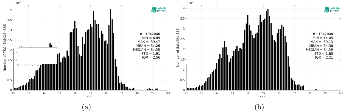
Figure 2: Histograms of SSS from TSG (SAMOS) (a) and CCI SSS L4 Merged-OI v3.2 - 7-day running (ESA) (b) considering all match-up pairs per bins of 0.1 over the Global Ocean Pi-MEP region and for the full satellite product period.
