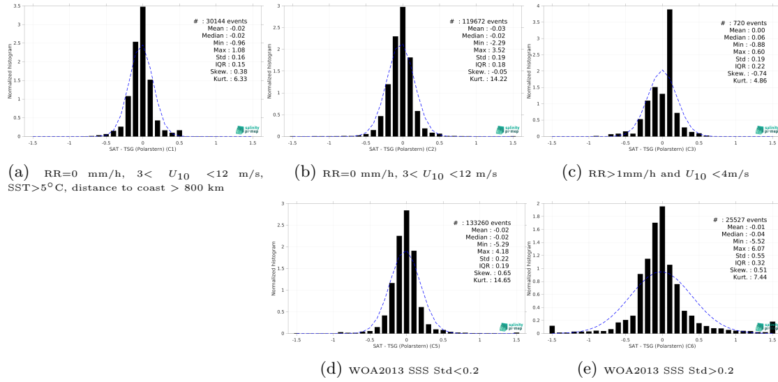
Figure 13: Normalized histogram of \Delta\text{SSS} (CCI SSS L4 Merged-OI v3.2 - 7-day running (ESA) - TSG (Polarstern)) for 5 different subdatasets corresponding to: RR=0 mm/h, 3 < U_{10} < 12 m/s, SST>5°C, distance to coast > 800 km (a), RR=0 mm/h, 3 < U_{10} < 12 m/s (b), RR>1mm/h and U_{10} < 4 m/s (c), WOA2013 SSS Std<0.2 (d), WOA2013 SSS Std>0.2 (e).
