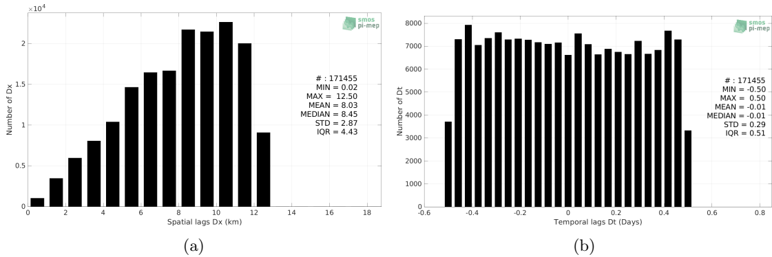
Figure 5: Histograms of the spatial (a) and temporal (b) lags between the location/time of the TSG (Polarstern) measurement and the date of the corresponding CCI SSS L4 Merged-OI v3.2 - 7-day running (ESA) SSS pixel.
