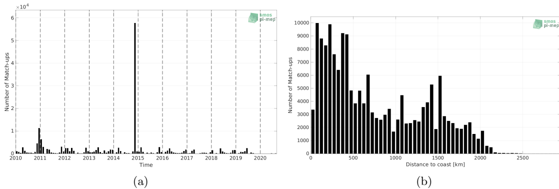
Figure 1: Number of match-ups between TSG (Polarstern) and CCI SSS L4 Merged-OI v3.2 - 7-day running (ESA) SSS as a function of time (a) and as function of the distance to coast (b) over the Global Ocean Pi-MEP region and for the full satellite product period.
