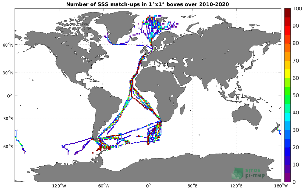
Figure 4: Number of SSS match-ups between TSG (Polarstern) SSS and the CCI SSS L4 Merged-OI v3.2 - 7-day running (ESA) SSS product for the Global Ocean Pi-MEP region over 1^\circ \times 1^\circ boxes and for the full satellite product period.
