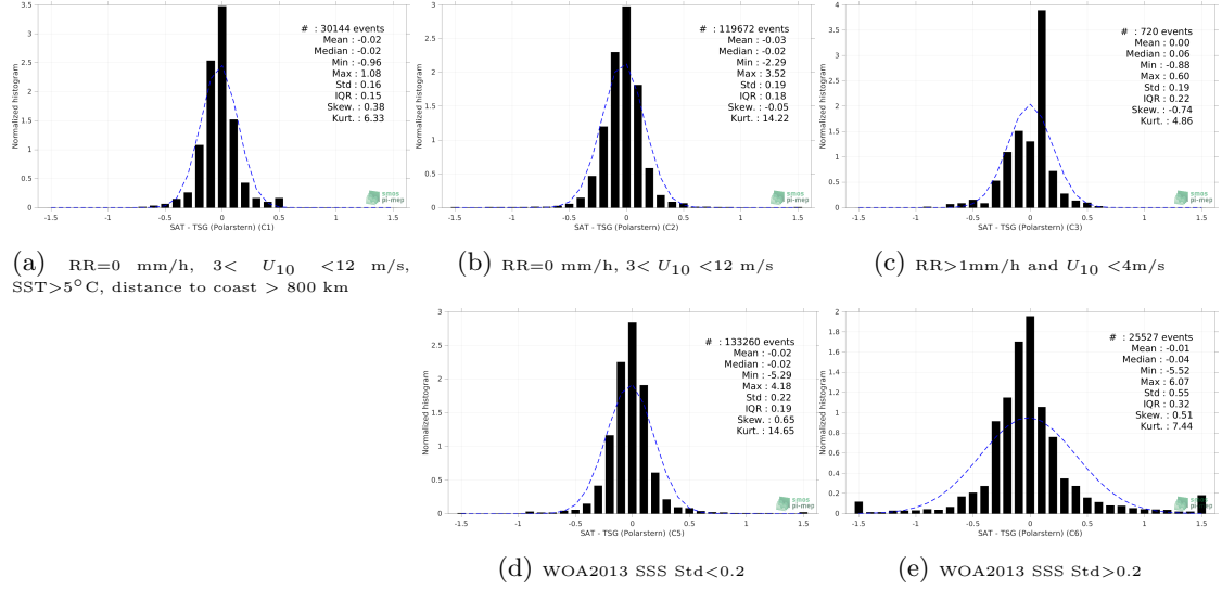
Figure 13: Normalized histogram of \Delta\text{SSS} (CCI SSS L4 Merged-OI v3.2 - 7-day running (ESA) - TSG (Polarstern)) for 5 different subdatasets corresponding to: RR=0 mm/h, 3 < U_{10} < 12 m/s, SST>5°C, distance to coast > 800 km (a), RR=0 mm/h, 3 < U_{10} < 12 m/s (b), RR>1mm/h and U_{10} < 4 m/s (c), WOA2013 SSS Std<0.2 (d), WOA2013 SSS Std>0.2 (e).
