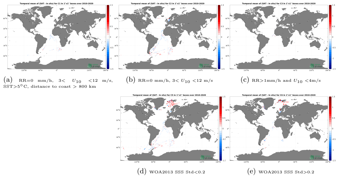
Figure 12: Temporal mean gridded over spatial boxes of size 1^\circ \times 1^\circ of \Delta SSS (CCI SSS L4 Merged-OI v3.2 - 7-day running (ESA) - TSG (Polarstern)) for 5 different subdatasets corresponding to:RR=0 mm/h, 3 < U_{10} < 12 m/s, SST > 5^\circ\text{C} , distance to coast > 800 km (a), RR=0 mm/h, 3 < U_{10} < 12 m/s (b), RR > 1 mm/h and U_{10} < 4 m/s (c), WOA2013 SSS Std < 0.2 (d), WOA2013 SSS Std > 0.2 (e).
