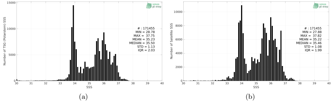
Figure 2: Histograms of SSS from TSG (Polarstern) (a) and CCI SSS L4 Merged-OI v3.2 - 7-day running (ESA) (b) considering all match-up pairs per bins of 0.1 over the Global Ocean Pi-MEP region and for the full satellite product period.
