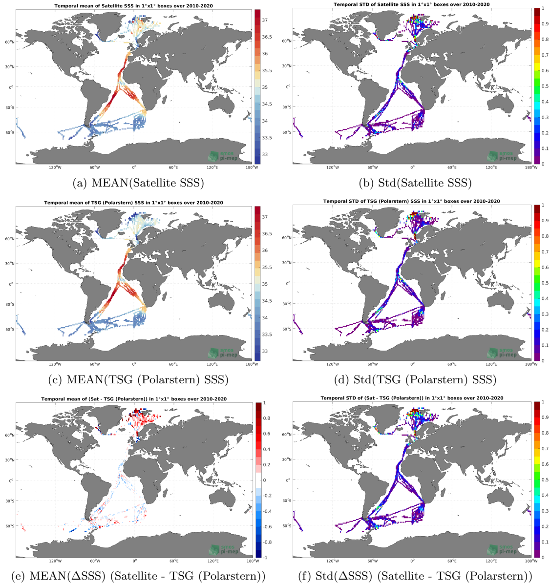
Figure 6: Temporal mean (left) and Std (right) of SSS from CCI SSS L4 Merged-OI v3.2 - 7-day running (ESA) (top), TSG (Polarstern) (middle), and of \Delta SSS (Satellite - TSG (Polarstern)). Only match-up pairs are used to generate these maps.
