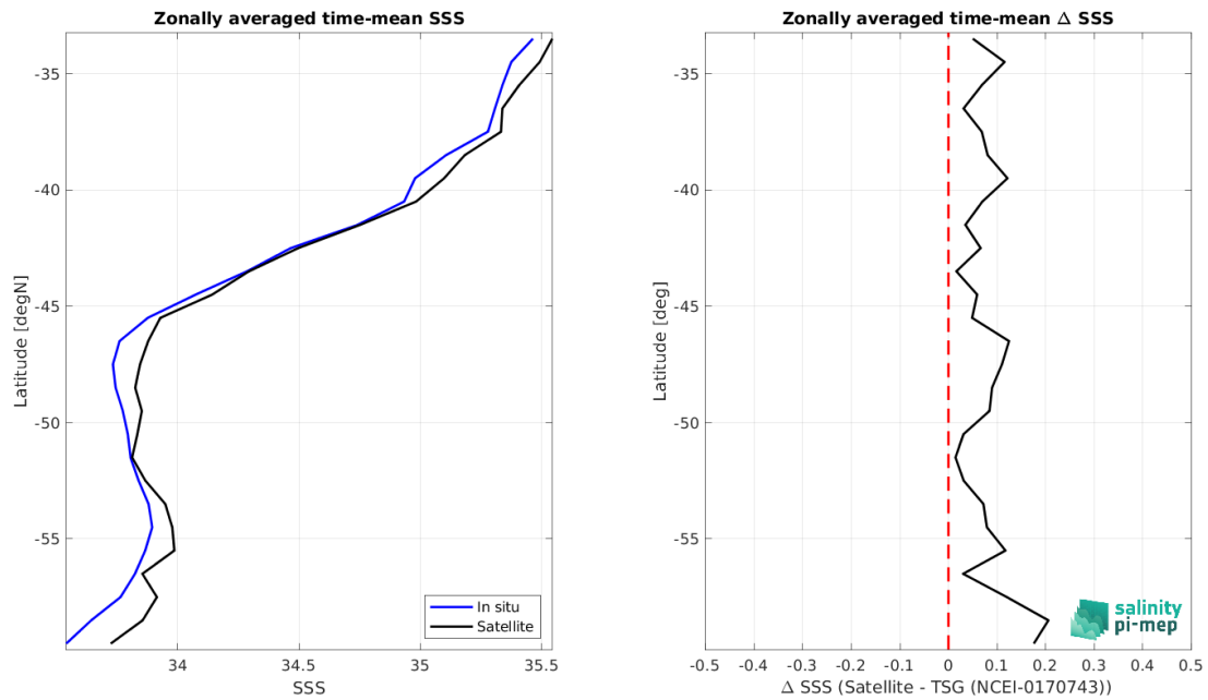
Figure 8: Left panel: Zonal mean SSS from CCI SSS L4 Merged-OI v3.2 - 7-day running (ESA) satellite product (black) and from TSG (NCEI-0170743) (blue). Right panel: Zonal mean of \Delta SSS (Satellite - TSG (NCEI-0170743)) for all the collected Pi-MEP match-up pairs estimated over the full satellite product period.
