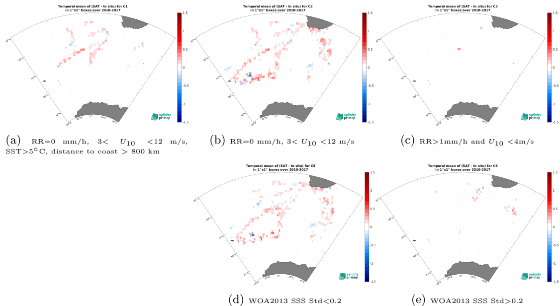
Figure 12: Temporal mean gridded over spatial boxes of size 1^{\circ}\times 1^{\circ} of \Delta\text{SSS} (CCI SSS L4 Merged-OI v3.2 - 7-day running (ESA) - TSG (NCEI-0170743)) for 5 different subdatasets corresponding to:RR=0 mm/h, 3 < U_{10} < 12 m/s, SST >5^{\circ}\text{C} , distance to coast > 800 km (a), RR=0 mm/h, 3 < U_{10} < 12 m/s (b), RR >1 mm/h and U_{10} < 4 m/s (c), WOA2013 SSS Std <0.2 (d), WOA2013 SSS Std >0.2 (e).
