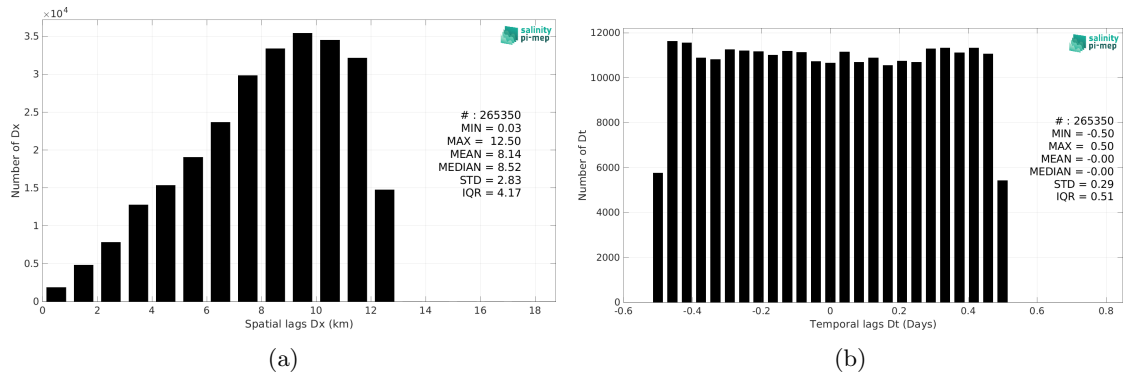
Figure 5: Histograms of the spatial (a) and temporal (b) lags between the location/time of the TSG (NCEI-0170743) measurement and the date of the corresponding CCI SSS L4 Merged-OI v3.2 - 7-day running (ESA) SSS pixel.
