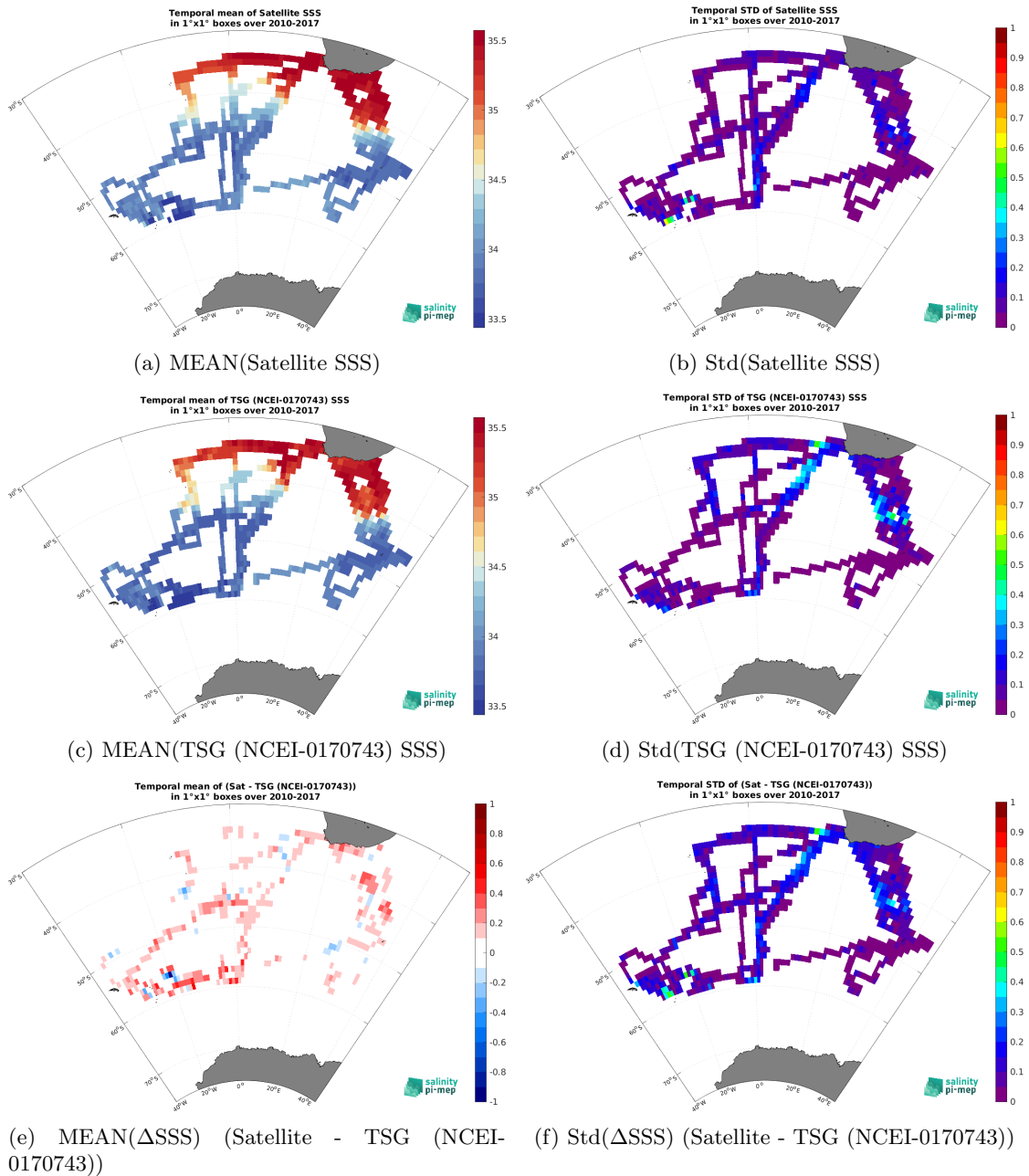
Figure 6: Temporal mean (left) and Std (right) of SSS from CCI SSS L4 Merged-OI v3.2 - 7-day running (ESA) (top), TSG (NCEI-0170743) (middle), and of \Delta SSS (Satellite - TSG (NCEI-0170743)). Only match-up pairs are used to generate these maps.
