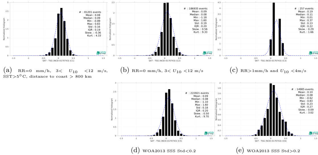
Figure 13: Normalized histogram of \Delta\text{SSS} (CCI SSS L4 Merged-OI v3.2 - 7-day running (ESA) - TSG (NCEI-0170743)) for 5 different subdatasets corresponding to: RR=0 mm/h, 3 < U_{10} < 12 m/s, SST>5°C, distance to coast > 800 km (a), RR=0 mm/h, 3 < U_{10} < 12 m/s (b), RR>1mm/h and U_{10} < 4 m/s (c), WOA2013 SSS Std<0.2 (d), WOA2013 SSS Std>0.2 (e).
