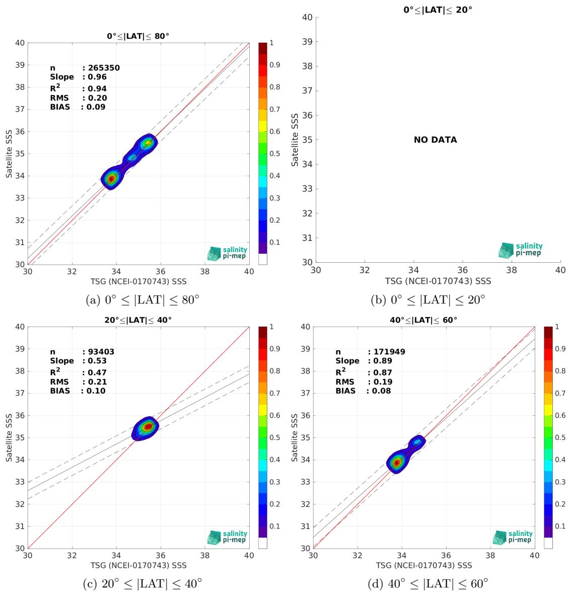
Figure 9: Contour maps of the concentration of CCI SSS L4 Merged-OI v3.2 - 7-day running (ESA) SSS (y-axis) versus TSG (NCEI-0170743) SSS (x-axis) at match-up pairs for different latitude bands. For each plot, the red line shows x=y . The black thin and dashed lines indicate a linear fit through the data cloud and the \pm 95\% confidence levels, respectively. The number match-up pairs n , the slope and R^2 coefficient of the linear fit, the root mean square (RMS) and the mean bias between satellite and in situ data are indicated for each latitude band in each plots.
