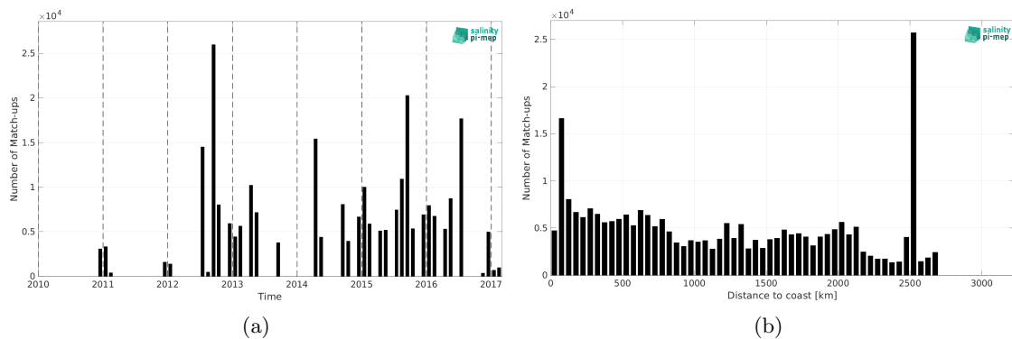
Figure 1: Number of match-ups between TSG (NCEI-0170743) and CCI SSS L4 Merged-OI v3.2 - 7-day running (ESA) SSS as a function of time (a) and as function of the distance to coast (b) over the Global Ocean Pi-MEP region and for the full satellite product period.
