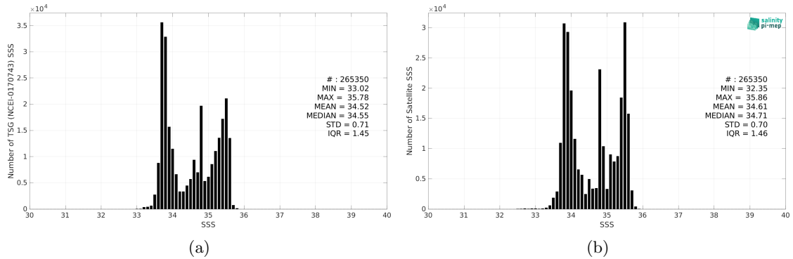
Figure 2: Histograms of SSS from TSG (NCEI-0170743) (a) and CCI SSS L4 Merged-OI v3.2 - 7-day running (ESA) (b) considering all match-up pairs per bins of 0.1 over the Global Ocean Pi-MEP region and for the full satellite product period.
