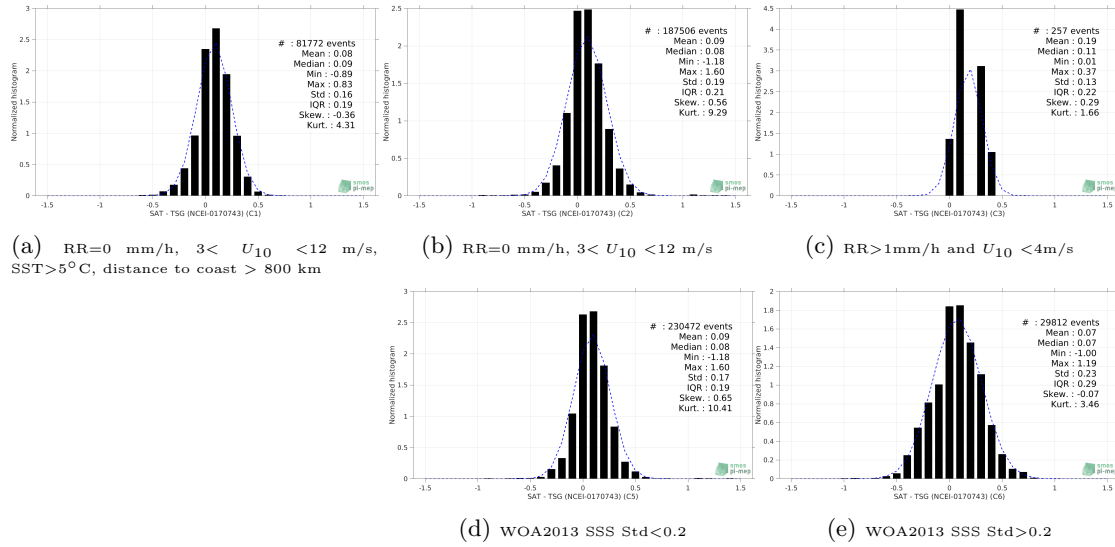
Figure 13: Normalized histogram of \Delta SSS (CCI SSS L4 Merged-OI v3.2 - 7-day running (ESA) - TSG (NCEI-0170743)) for 5 different subdatasets corresponding to: RR=0 mm/h, 3 < U_{10} < 12 m/s, SST>5°C, distance to coast > 800 km (a), RR=0 mm/h, 3 < U_{10} < 12 m/s, SST>5°C, distance to coast > 800 km (a), RR=0 mm/h, 3 < U_{10} < 12 m/s (b), RR>1mm/h and U_{10} < 4 m/s (c), WOA2013 SSS Std<0.2 (d), WOA2013 SSS Std>0.2 (e).
