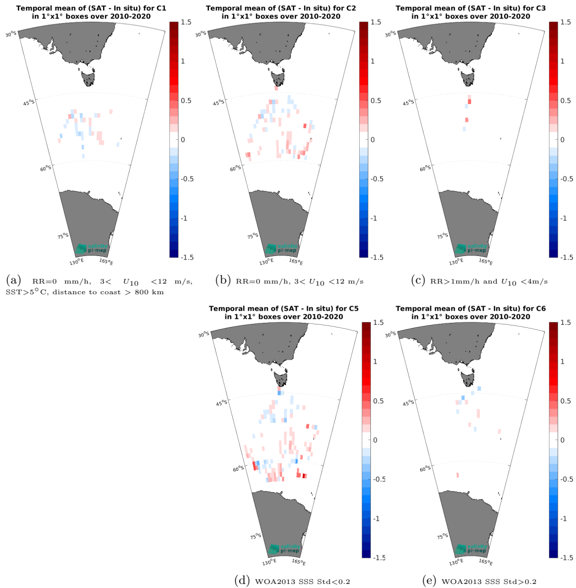
Figure 12: Temporal mean gridded over spatial boxes of size 1^\circ \times 1^\circ of \Delta\text{SSS} (CCI SSS L4 Merged-OI v3.2 - 7-day running (ESA) - TSG (LEGOS-Survostral)) for 5 different subdatasets corresponding to: RR=0 mm/h, 3 < U_{10} < 12 m/s, SST > 5^\circ\text{C} , distance to coast > 800 km (a), RR=0 mm/h, 3 < U_{10} < 12 m/s (b), RR > 1 mm/h and U_{10} < 4 m/s (c), WOA2013 SSS Std < 0.2 (d), WOA2013 SSS Std > 0.2 (e).
