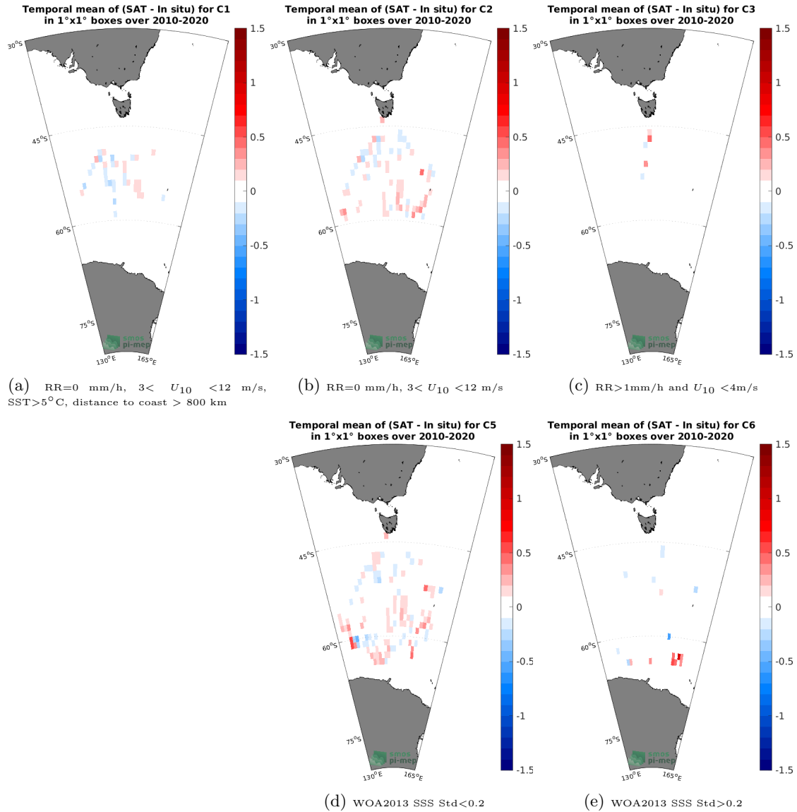
Figure 12: Temporal mean gridded over spatial boxes of size 1^\circ \times 1^\circ of \Delta SSS (CCI SSS L4 Merged-OI v3.2 - 7-day running (ESA) - TSG (LEGOS-Survostral)) for 5 different subdatasets corresponding to:RR=0 mm/h, 3 < U_{10} < 12 m/s, SST>5°C, distance to coast > 800 km (a), RR=0 mm/h, 3 < U_{10} < 12 m/s (b), RR>1mm/h and U_{10} < 4 m/s (c), WOA2013 SSS Std<0.2 (d), WOA2013 SSS Std>0.2 (e).
