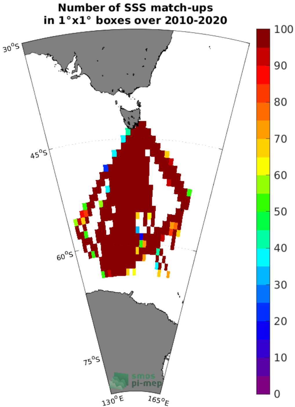
Figure 4: Number of SSS match-ups between TSG (LEGOS-Survostral) SSS and the CCI SSS L4 Merged-OI v3.2 - 7-day running (ESA) SSS product for the Global Ocean Pi-MEP region over 1°×1° boxes and for the full satellite product period.
