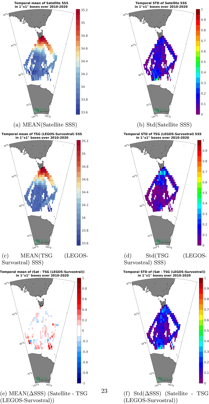
Figure 6: Temporal mean (left) and Std (right) of SSS from CCI SSS L4 Merged-OI v3.2 - 7-day running (ESA) (top), TSG (LEGOS-Survostral) (middle), and of \Delta SSS (Satellite - TSG (LEGOS-Survostral)). Only match-up pairs are used to generate these maps.
