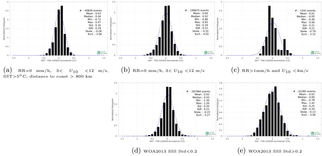
Figure 13: Normalized histogram of \Delta SSS (CCI SSS L4 Merged-OI v3.2 - 7-day running (ESA) - TSG (LEGOS-Survostral)) for 5 different subdatasets corresponding to: RR=0 mm/h, 3 < U_{10} < 12 m/s, SST>5°C, distance to coast > 800 km (a), RR=0 mm/h, 3 < U_{10} < 12 m/s (b), RR>1mm/h and U_{10} < 4 m/s (c), WOA2013 SSS Std<0.2 (d), WOA2013 SSS Std>0.2 (e).
