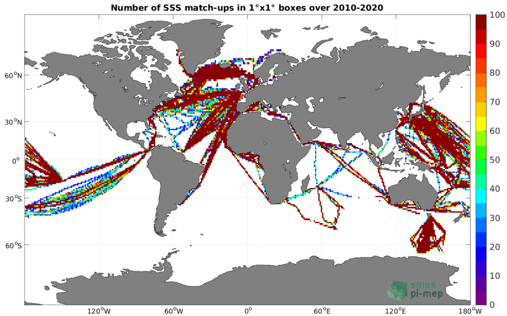
Figure 4: Number of SSS match-ups between TSG (LEGOS-DM) SSS and the CCI SSS L4 Merged-OI v3.2 - 7-day running (ESA) SSS product for the Global Ocean Pi-MEP region over 1^\circ \times 1^\circ boxes and for the full satellite product period.
