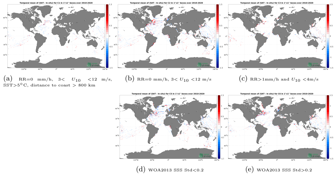
Figure 12: Temporal mean gridded over spatial boxes of size 1^\circ \times 1^\circ of \Delta SSS (CCI SSS L4 Merged-OI v3.2 - 7-day running (ESA) - TSG (LEGOS-DM)) for 5 different subdatasets corresponding to:RR=0 mm/h, 3 < U_{10} < 12 m/s, SST > 5^\circ\text{C} , distance to coast > 800 km (a), RR=0 mm/h, 3 < U_{10} < 12 m/s (b), RR > 1 mm/h and U_{10} < 4 m/s (c), WOA2013 SSS Std < 0.2 (d), WOA2013 SSS Std > 0.2 (e).
