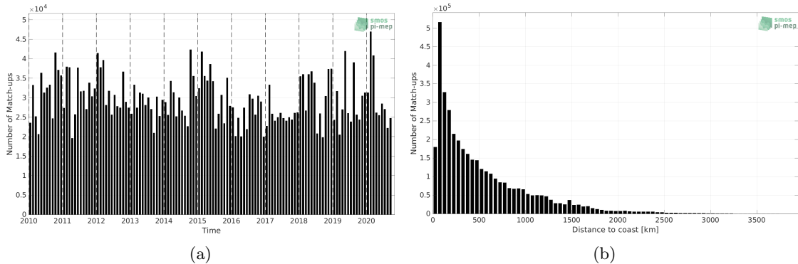
Figure 1: Number of match-ups between TSG (LEGOS-DM) and CCI SSS L4 Merged-OI v3.2 - 7-day running (ESA) SSS as a function of time (a) and as function of the distance to coast (b) over the Global Ocean Pi-MEP region and for the full satellite product period.
