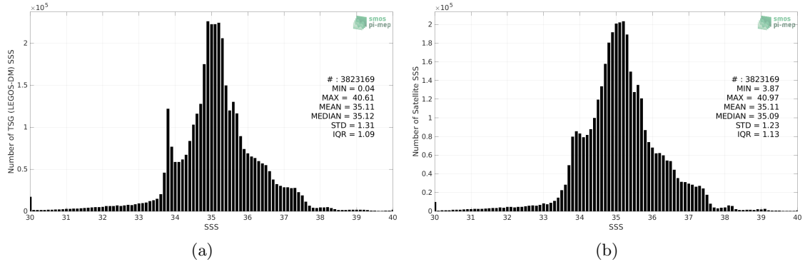
Figure 2: Histograms of SSS from TSG (LEGOS-DM) (a) and CCI SSS L4 Merged-OI v3.2 - 7-day running (ESA) (b) considering all match-up pairs per bins of 0.1 over the Global Ocean Pi-MEP region and for the full satellite product period.
