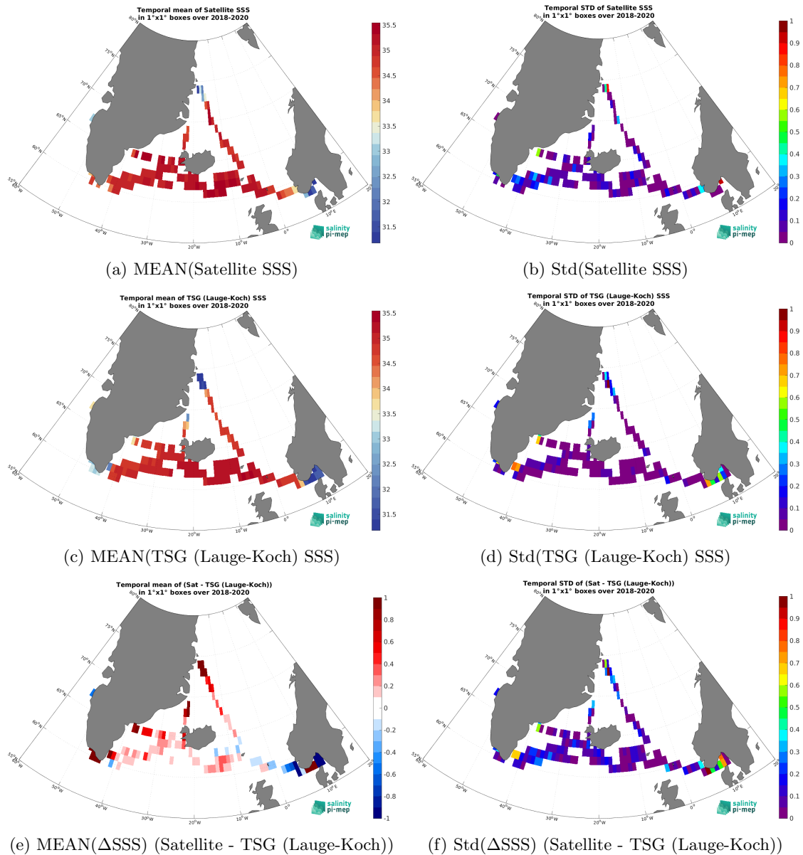
Figure 6: Temporal mean (left) and Std (right) of SSS from CCI SSS L4 Merged-OI v3.2 - 7-day running (ESA) (top), TSG (Lauge-Koch) (middle), and of \Delta SSS (Satellite - TSG (Lauge-Koch)). Only match-up pairs are used to generate these maps.
