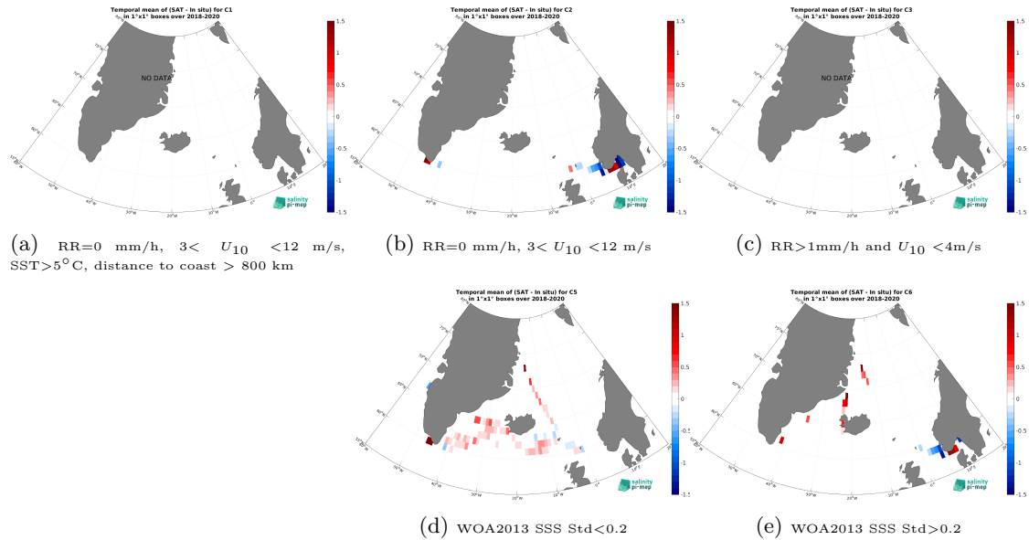
Figure 12: Temporal mean gridded over spatial boxes of size 1^{\circ}\times 1^{\circ} of \Delta\text{SSS} (CCI SSS L4 Merged-OI v3.2 - 7-day running (ESA) - TSG (Lauge-Koch)) for 5 different subdatasets corresponding to:RR=0 mm/h, 3 < U_{10} < 12 m/s, SST > 5^{\circ}\text{C} , distance to coast > 800 km (a), RR=0 mm/h, 3 < U_{10} < 12 m/s (b), RR > 1 mm/h and U_{10} < 4 m/s (c), WOA2013 SSS Std < 0.2 (d), WOA2013 SSS Std > 0.2 (e).
