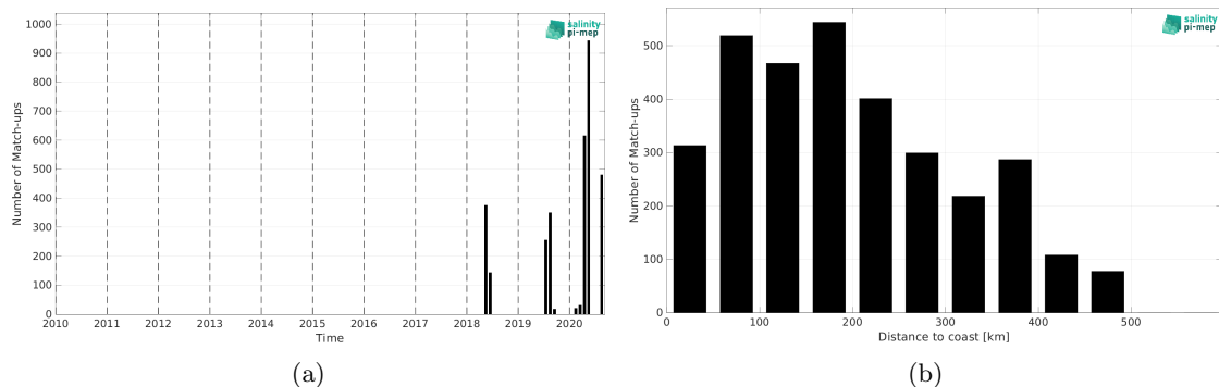
Figure 1: Number of match-ups between TSG (Lauge-Koch) and CCI SSS L4 Merged-OI v3.2 - 7-day running (ESA) SSS as a function of time (a) and as function of the distance to coast (b) over the Global Ocean Pi-MEP region and for the full satellite product period.
