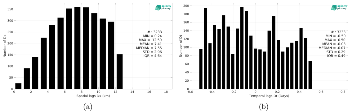
Figure 5: Histograms of the spatial (a) and temporal (b) lags between the location/time of the TSG (Lauge-Koch) measurement and the date of the corresponding CCI SSS L4 Merged-OI v3.2 - 7-day running (ESA) SSS pixel.
