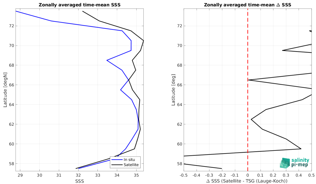
Figure 8: Left panel: Zonal mean SSS from CCI SSS L4 Merged-OI v3.2 - 7-day running (ESA) satellite product (black) and from TSG (Lauge-Koch) (blue). Right panel: Zonal mean of \Delta SSS (Satellite - TSG (Lauge-Koch)) for all the collected Pi-MEP match-up pairs estimated over the full satellite product period.
