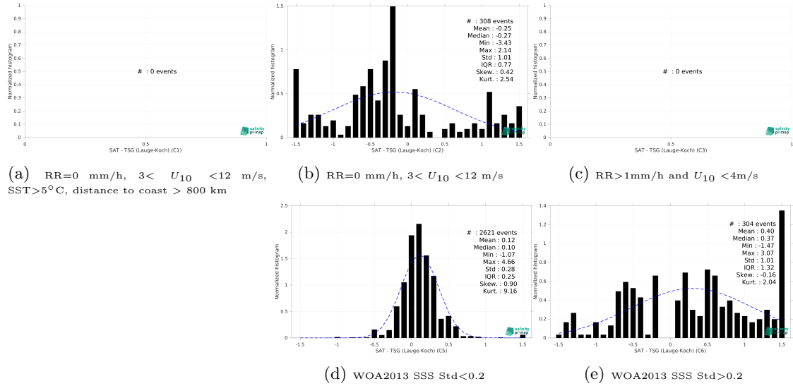
Figure 13: Normalized histogram of \Delta SSS (CCI SSS L4 Merged-OI v3.2 - 7-day running (ESA) - TSG (Lauge-Koch)) for 5 different subdatasets corresponding to: RR=0 mm/h, 3 < U_{10} < 12 m/s, SST>5°C, distance to coast > 800 km (a), RR=0 mm/h, 3 < U_{10} < 12 m/s (b), RR>1mm/h and U_{10} < 4 m/s (c), WOA2013 SSS Std<0.2 (d), WOA2013 SSS Std>0.2 (e).
