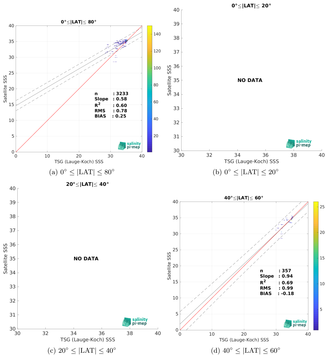
Figure 9: Contour maps of the concentration of CCI SSS L4 Merged-OI v3.2 - 7-day running (ESA) SSS (y-axis) versus TSG (Lauge-Koch) SSS (x-axis) at match-up pairs for different latitude bands. For each plot, the red line shows x=y . The black thin and dashed lines indicate a linear fit through the data cloud and the \pm 95\% confidence levels, respectively. The number match-up pairs n , the slope and R^2 coefficient of the linear fit, the root mean square (RMS) and the mean bias between satellite and in situ data are indicated for each latitude band in each plots.
