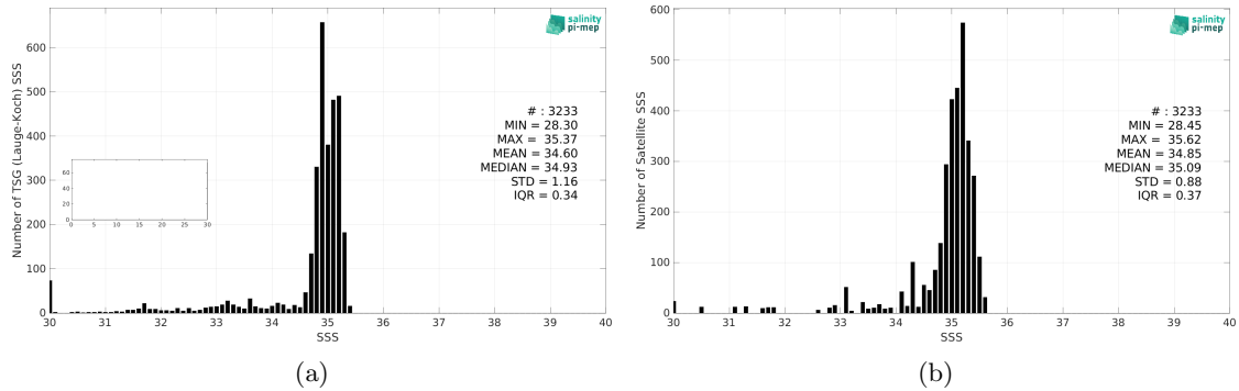
Figure 2: Histograms of SSS from TSG (Lauge-Koch) (a) and CCI SSS L4 Merged-OI v3.2 - 7-day running (ESA) (b) considering all match-up pairs per bins of 0.1 over the Global Ocean Pi-MEP region and for the full satellite product period.
