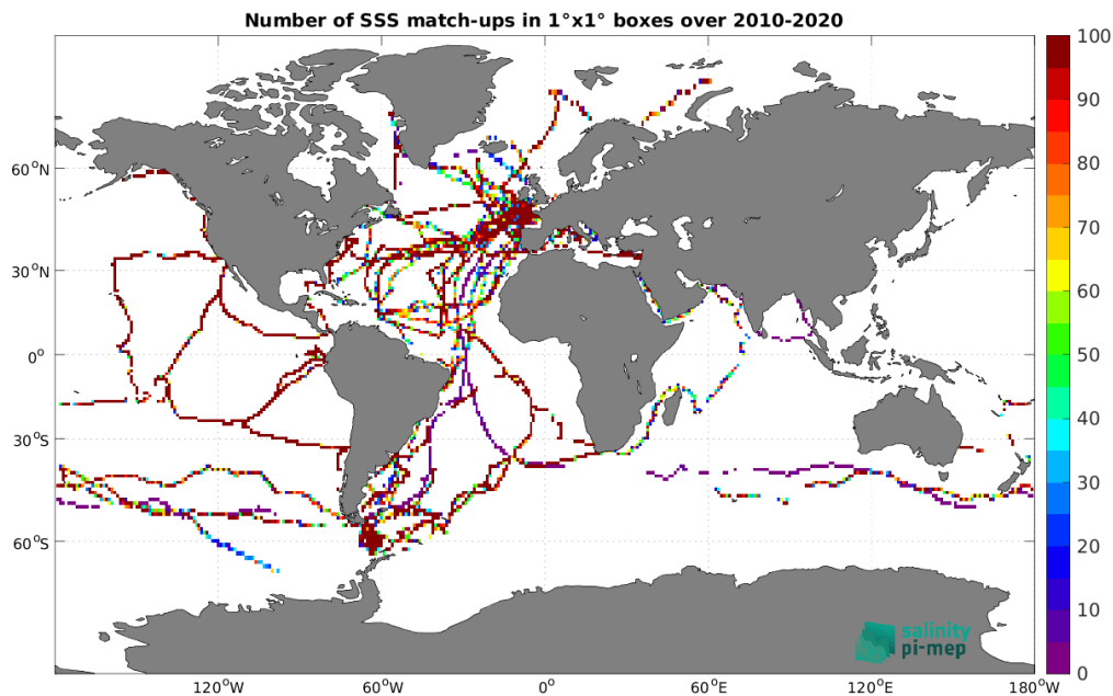
Figure 4: Number of SSS match-ups between TSG (GOSUD-Sailing-ship) SSS and the CCI SSS L4 Merged-OI v3.2 - 7-day running (ESA) SSS product for the Global Ocean Pi-MEP region over 1^\circ \times 1^\circ boxes and for the full satellite product period.
