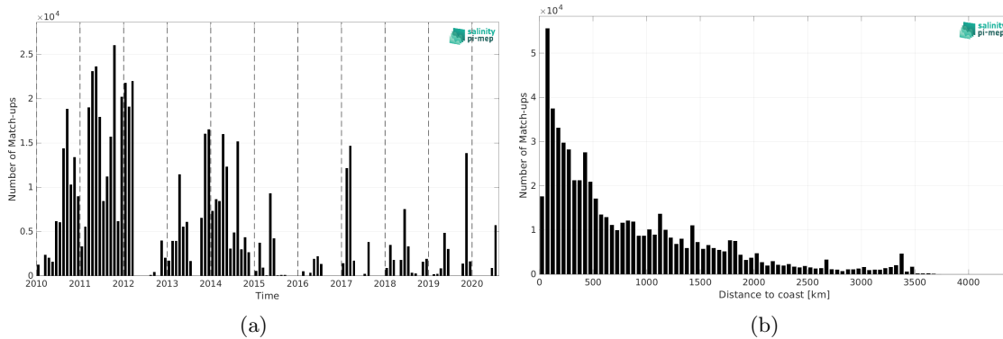
Figure 1: Number of match-ups between TSG (GOSUD-Sailing-ship) and CCI SSS L4 Merged-OI v3.2 - 7-day running (ESA) SSS as a function of time (a) and as function of the distance to coast (b) over the Global Ocean Pi-MEP region and for the full satellite product period.
