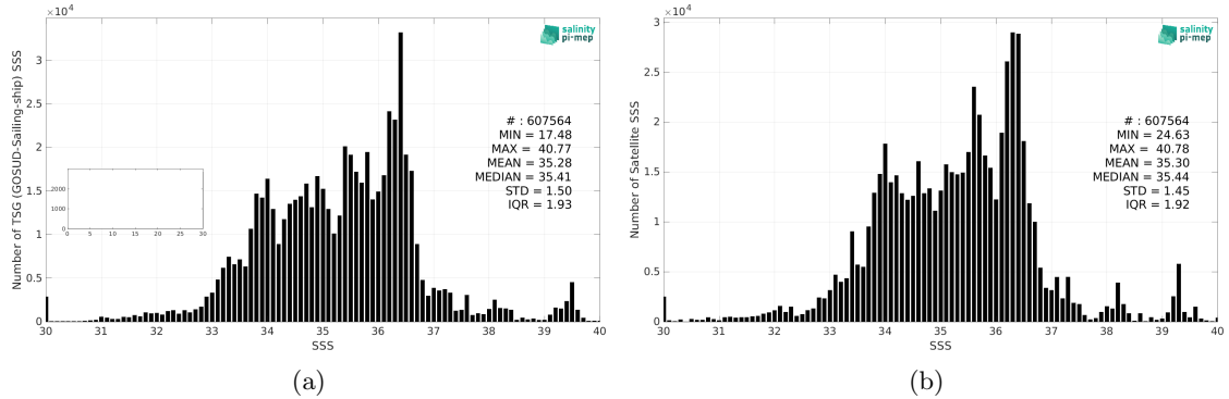
Figure 2: Histograms of SSS from TSG (GOSUD-Sailing-ship) (a) and CCI SSS L4 Merged-OI v3.2 - 7-day running (ESA) (b) considering all match-up pairs per bins of 0.1 over the Global Ocean Pi-MEP region and for the full satellite product period.
