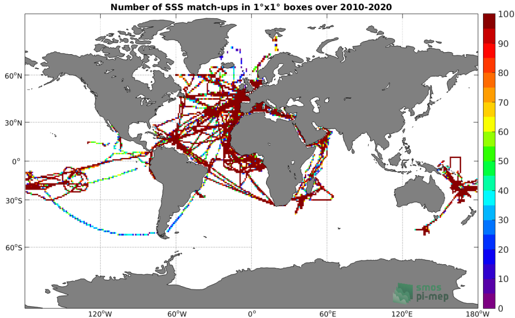
Figure 4: Number of SSS match-ups between TSG (GOSUD-Research-vessel) SSS and the CCI SSS L4 Merged-OI v3.2 - 7-day running (ESA) SSS product for the Global Ocean Pi-MEP region over 1^\circ \times 1^\circ boxes and for the full satellite product period.
