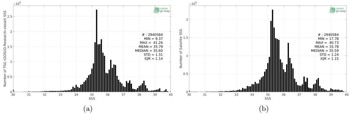
Figure 2: Histograms of SSS from TSG (GOSUD-Research-vessel) (a) and CCI SSS L4 Merged-OI v3.2 - 7-day running (ESA) (b) considering all match-up pairs per bins of 0.1 over the Global Ocean Pi-MEP region and for the full satellite product period.
