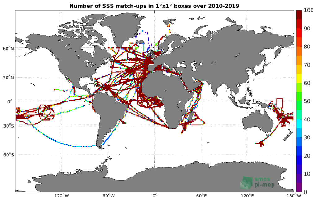
Figure 4: Number of SSS match-ups between TSG (GOSUD-Research-vessel) SSS and the CCI SSS L4 Merged-OI v3.2 - 7-day running (ESA) SSS product for the Global Ocean Pi-MEP region over 1°x1° boxes and for the full satellite product period.
