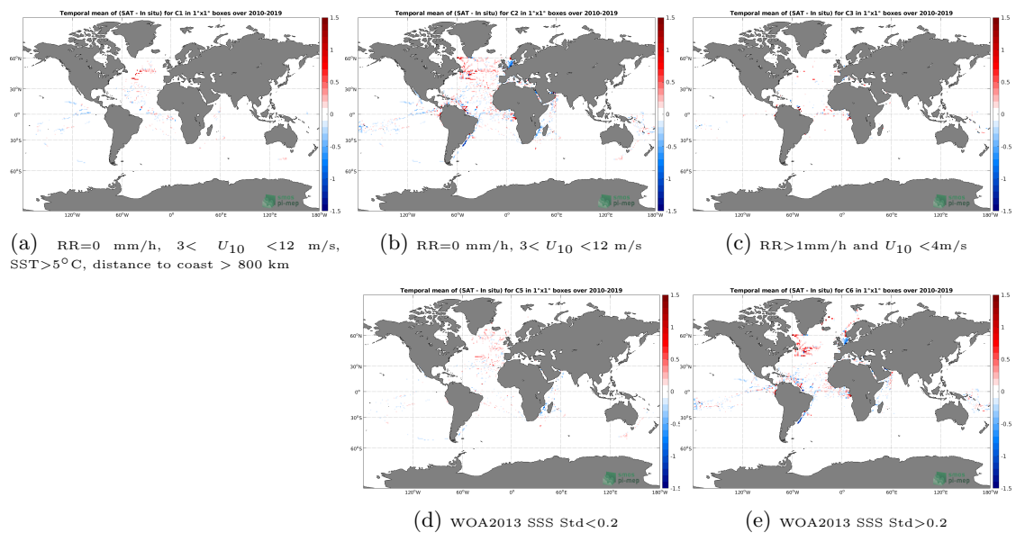
Figure 12: Temporal mean gridded over spatial boxes of size 1^\circ \times 1^\circ of \Delta\text{SSS} (CCI SSS L4 Merged-OI v3.2 - 7-day running (ESA) - TSG (GOSUD-Research-vessel)) for 5 different subdatasets corresponding to:RR=0 mm/h, 3 < U_{10} < 12 m/s, SST>5°C, distance to coast > 800 km (a), RR=0 mm/h, 3 < U_{10} < 12 m/s (b), RR>1mm/h and U_{10} < 4 m/s (c), WOA2013 SSS Std<0.2 (d), WOA2013 SSS Std>0.2 (e).
