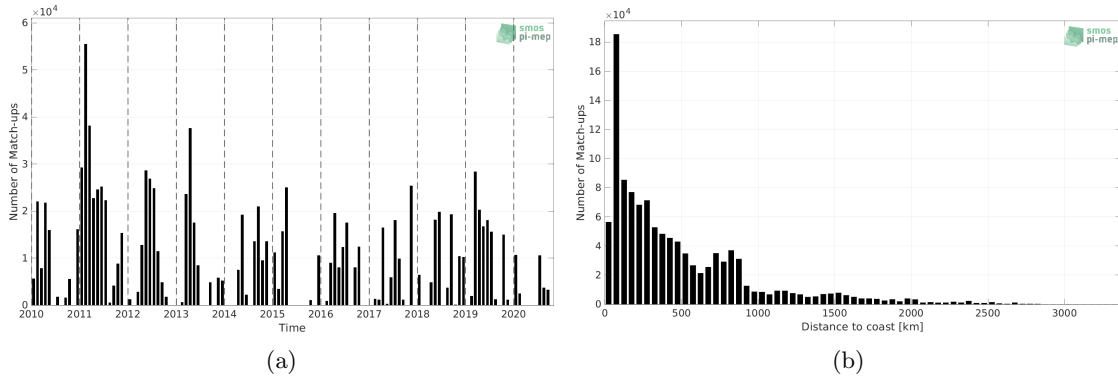
Figure 1: Number of match-ups between TSG (CSIC-UTM) and CCI SSS L4 Merged-OI v3.2 - 7-day running (ESA) SSS as a function of time (a) and as function of the distance to coast (b) over the Global Ocean Pi-MEP region and for the full satellite product period.
