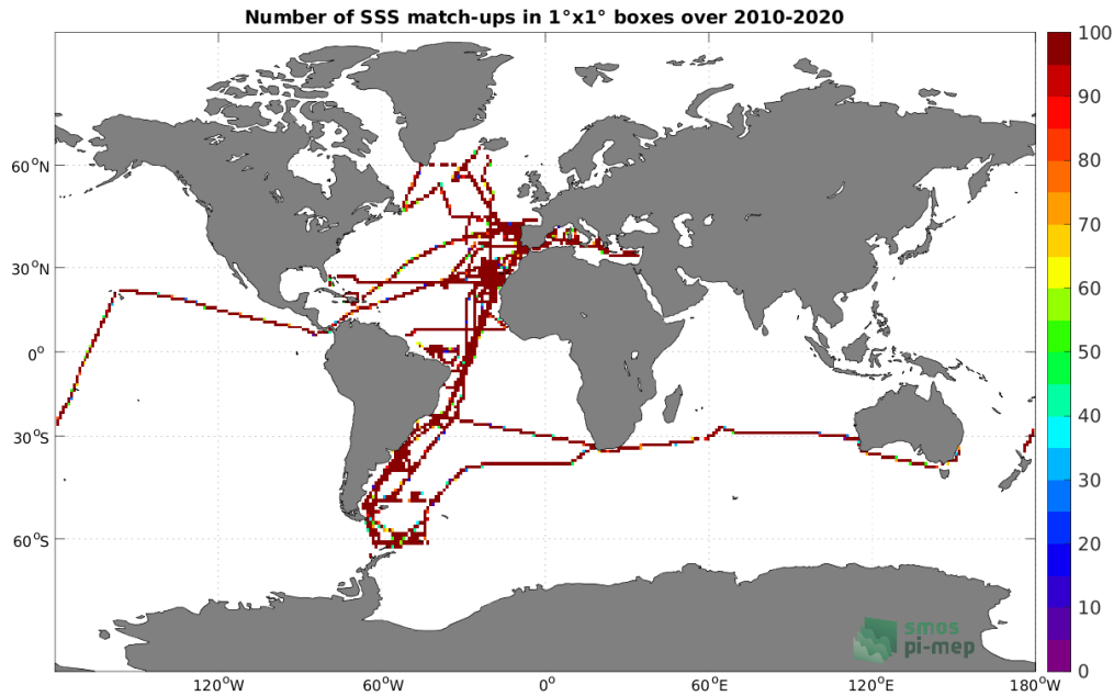
Figure 4: Number of SSS match-ups between TSG (CSIC-UTM) SSS and the CCI SSS L4 Merged-OI v3.2 - 7-day running (ESA) SSS product for the Global Ocean Pi-MEP region over 1^\circ \times 1^\circ boxes and for the full satellite product period.
