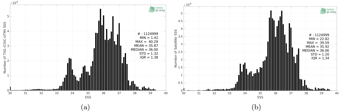
Figure 2: Histograms of SSS from TSG (CSIC-UTM) (a) and CCI SSS L4 Merged-OI v3.2 - 7-day running (ESA) (b) considering all match-up pairs per bins of 0.1 over the Global Ocean Pi-MEP region and for the full satellite product period.
