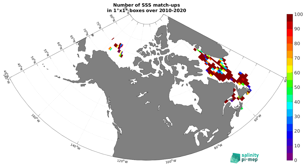
Figure 4: Number of SSS match-ups between TSG (Amundsen) SSS and the CCI SSS L4 Merged-OI v3.2 - 7-day running (ESA) SSS product for the Global Ocean Pi-MEP region over 1^\circ \times 1^\circ boxes and for the full satellite product period.
