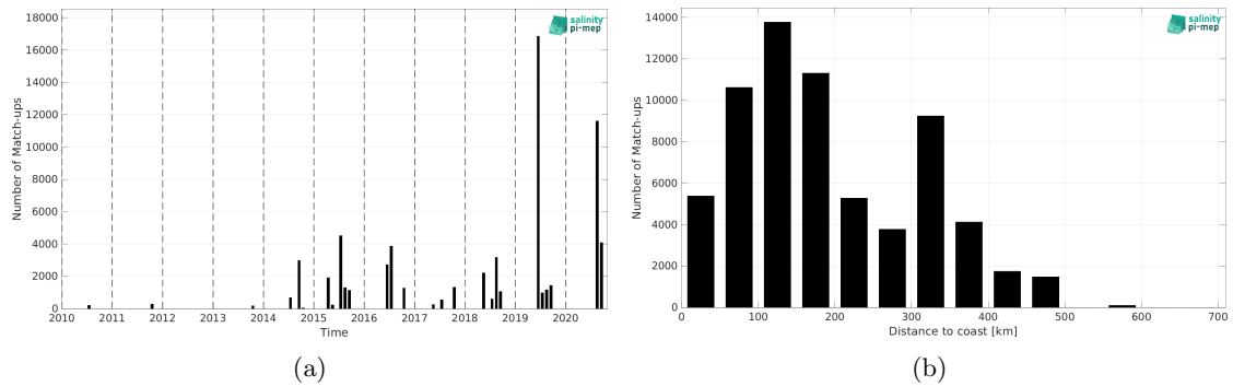
Figure 1: Number of match-ups between TSG (Amundsen) and CCI SSS L4 Merged-OI v3.2 - 7-day running (ESA) SSS as a function of time (a) and as function of the distance to coast (b) over the Global Ocean Pi-MEP region and for the full satellite product period.
