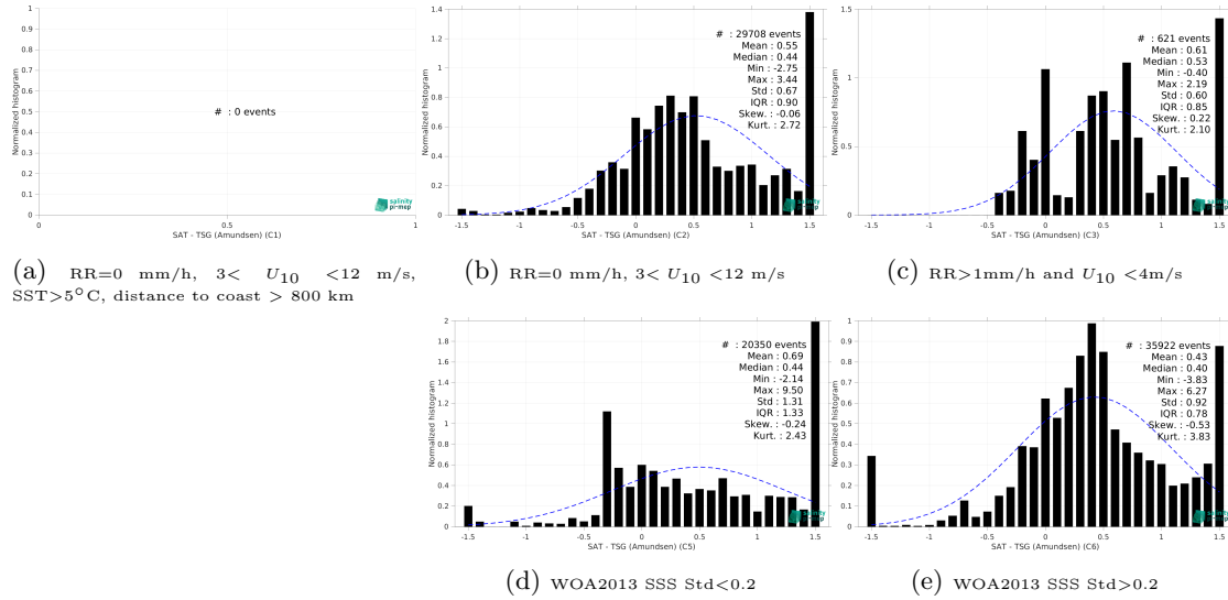
Figure 13: Normalized histogram of \Delta SSS (CCI SSS L4 Merged-OI v3.2 - 7-day running (ESA) - TSG (Amundsen)) for 5 different subdatasets corresponding to: RR=0 mm/h, 3 < U_{10} < 12 m/s, SST > 5°C, distance to coast > 800 km (a), RR=0 mm/h, 3 < U_{10} < 12 m/s (b), RR > 1mm/h and U_{10} < 4 m/s (c), WOA2013 SSS Std < 0.2 (d), WOA2013 SSS Std > 0.2 (e).
