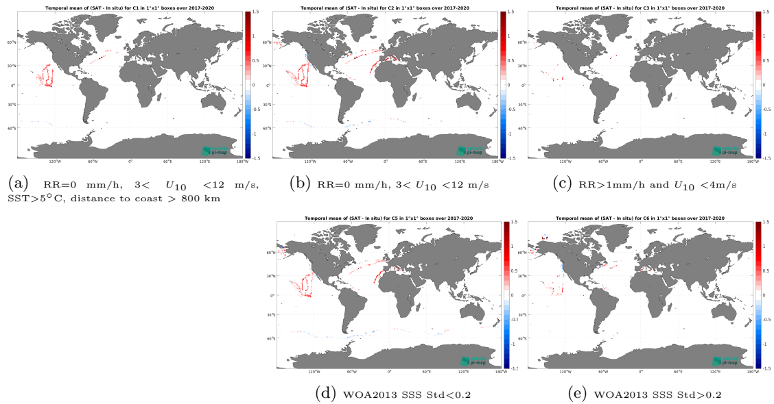
Figure 12: Temporal mean gridded over spatial boxes of size 1^\circ \times 1^\circ of \Delta SSS (CCI SSS L4 Merged-OI v3.2 - 7-day running (ESA) - Sailability) for 5 different subdatasets corresponding to:RR=0 mm/h, 3 < U_{10} < 12 m/s, SST > 5^\circ\text{C} , distance to coast > 800 km (a), RR=0 mm/h, 3 < U_{10} < 12 m/s (b), RR > 1 mm/h and U_{10} < 4 m/s (c), WOA2013 SSS Std < 0.2 (d), WOA2013 SSS Std > 0.2 (e).
