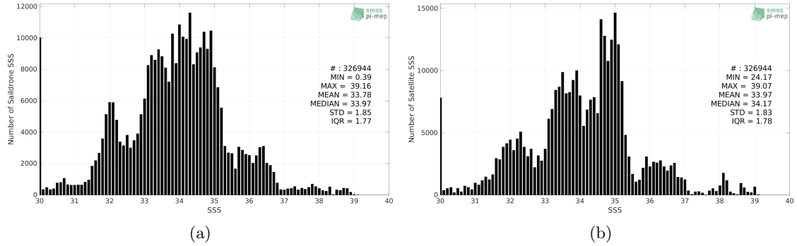
Figure 2: Histograms of SSS from Saildrone (a) and CCI SSS L4 Merged-OI v3.2 - 7-day running (ESA) (b) considering all match-up pairs per bins of 0.1 over the Global Ocean Pi-MEP region and for the full satellite product period.
