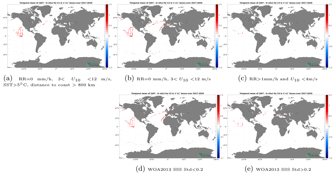
Figure 12: Temporal mean gridded over spatial boxes of size 1^\circ \times 1^\circ of \Delta SSS (CCI SSS L4 Merged-OI v3.2 - 7-day running (ESA) - Saildrone) for 5 different subdatasets corresponding to:RR=0 mm/h, 3 < U_{10} < 12 m/s, SST > 5^\circ\text{C} , distance to coast > 800 km (a), RR=0 mm/h, 3 < U_{10} < 12 m/s (b), RR > 1 mm/h and U_{10} < 4 m/s (c), WOA2013 SSS Std < 0.2 (d), WOA2013 SSS Std > 0.2 (e).
