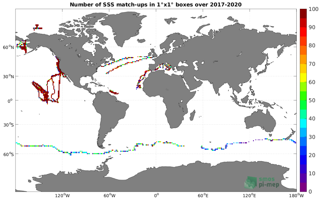
Figure 4: Number of SSS match-ups between Saildrone SSS and the CCI SSS L4 Merged-OI v3.2 - 7-day running (ESA) SSS product for the Global Ocean Pi-MEP region over 1^\circ \times 1^\circ boxes and for the full satellite product period.
