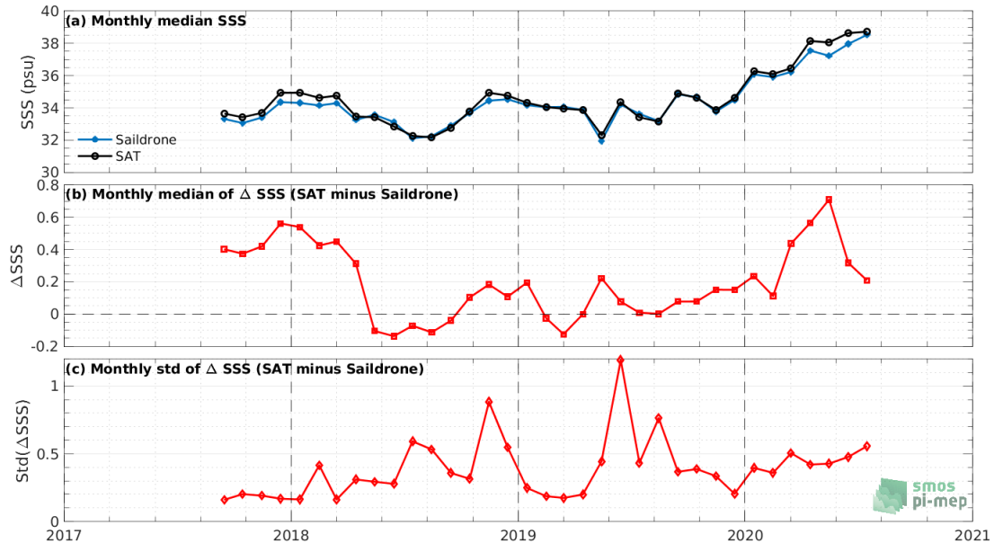
Figure 7: Time series of the monthly median SSS (top), median of \Delta SSS (Satellite - Sailldrone) and Std of \Delta SSS (Satellite - Sailldrone) over the Global Ocean Pi-MEP region considering all match-ups collected by the Pi-MEP.
