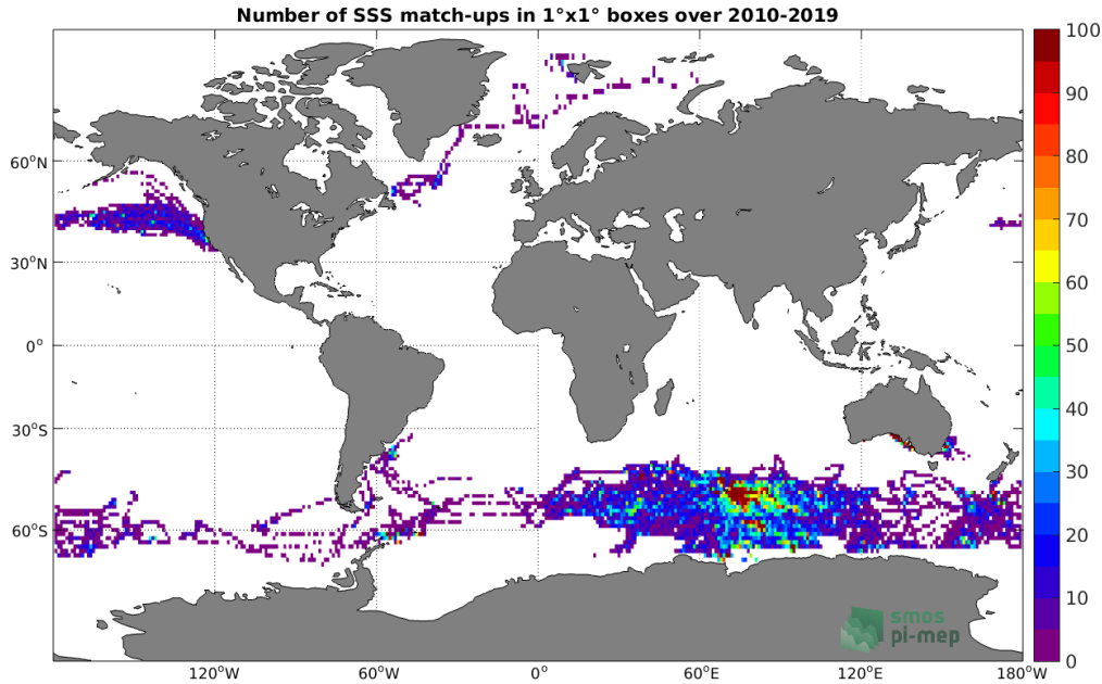
Figure 4: Number of SSS match-ups between Marine mammals SSS and the CCI SSS L4 Merged-OI v3.2 - 7-day running (ESA) SSS product for the Global Ocean Pi-MEP region over 1^\circ \times 1^\circ boxes and for the full satellite product period.
