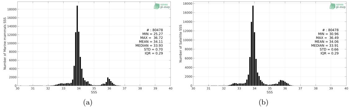
Figure 2: Histograms of SSS from Marine mammals (a) and CCI SSS L4 Merged-OI v3.2 - 7-day running (ESA) (b) considering all match-up pairs per bins of 0.1 over the Global Ocean Pi-MEP region and for the full satellite product period.
