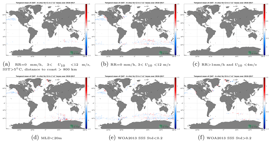
Figure 12: Temporal mean gridded over spatial boxes of size 1°x1° of \Delta SSS (CCI SSS L4 Merged-OI v3.2 - 7-day running (ESA) - Sea mammals) for 6 different subdatasets corresponding to:RR=0 mm/h, 3 < U_{10} < 12 m/s, SST > 5°C, distance to coast > 800 km (a), RR=0 mm/h, 3 < U_{10} < 12 m/s (b), RR > 1mm/h and U_{10} < 4 m/s (c),MLD < 20m (d),WOA2013 SSS Std < 0.2 (e),WOA2013 SSS Std > 0.2 (f).
