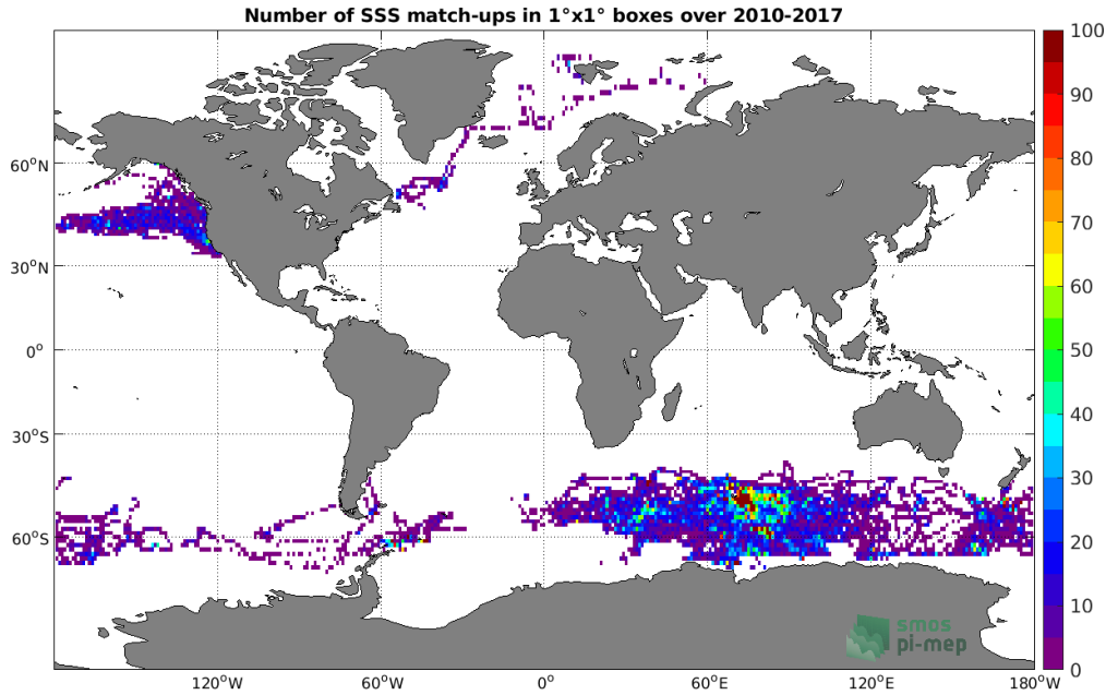
Figure 4: Number of SSS match-ups between Sea mammals SSS and the CCI SSS L4 Merged-OI v3.2 - 7-day running (ESA) SSS product for the Global Ocean Pi-MEP region over 1°x1° boxes and for the full satellite product period.
