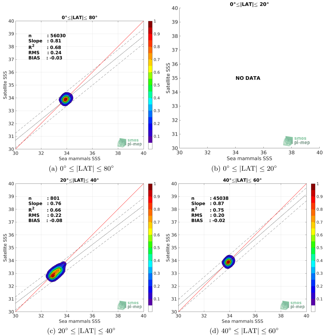
Figure 9: Contour maps of the concentration of CCI SSS L4 Merged-OI v3.2 - 7-day running (ESA) SSS (y-axis) versus Sea mammals SSS (x-axis) at match-up pairs for different latitude bands. For each plot, the red line shows x=y . The black thin and dashed lines indicate a linear fit through the data cloud and the \pm 95\% confidence levels, respectively. The number match-up pairs n , the slope and R^2 coefficient of the linear fit, the root mean square (RMS) and the mean bias between satellite and in situ data are indicated for each latitude band in each plots.
