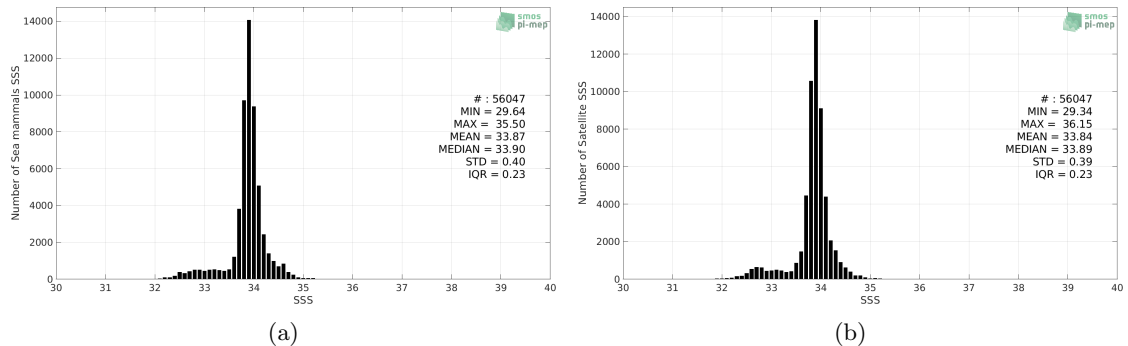
Figure 2: Histograms of SSS from Sea mammals (a) and CCI SSS L4 Merged-OI v3.2 - 7-day running (ESA) (b) considering all match-up pairs per bins of 0.1 over the Global Ocean Pi-MEP region and for the full satellite product period.
