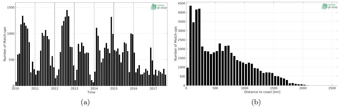
Figure 1: Number of match-ups between Sea mammals and CCI SSS L4 Merged-OI v3.2 - 7-day running (ESA) SSS as a function of time (a) and as function of the distance to coast (b) over the Global Ocean Pi-MEP region and for the full satellite product period.
