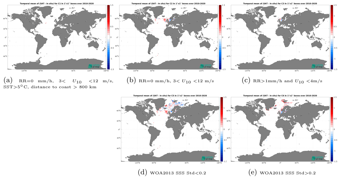
Figure 12: Temporal mean gridded over spatial boxes of size 1^\circ \times 1^\circ of \Delta SSS (CCI SSS L4 Merged-OI v3.2 - 7-day running (ESA) - ICES) for 5 different subdatasets corresponding to:RR=0 mm/h, 3 < U_{10} < 12 m/s, SST >5^\circ\text{C} , distance to coast > 800 km (a), RR=0 mm/h, 3 < U_{10} < 12 m/s (b), RR >1 mm/h and U_{10} < 4 m/s (c), WOA2013 SSS Std <0.2 (d), WOA2013 SSS Std >0.2 (e).
