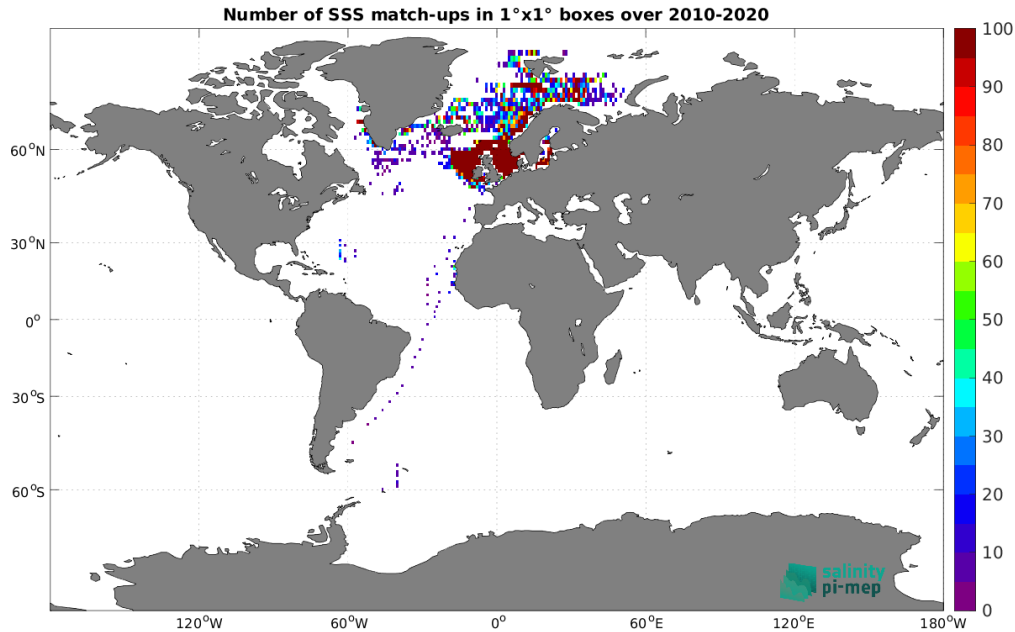
Figure 4: Number of SSS match-ups between ICES SSS and the CCI SSS L4 Merged-OI v3.2 - 7-day running (ESA) SSS product for the Global Ocean Pi-MEP region over 1^\circ \times 1^\circ boxes and for the full satellite product period.
