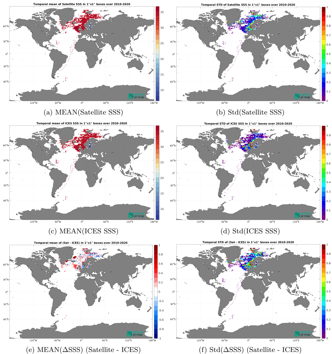
Figure 6: Temporal mean (left) and Std (right) of SSS from CCI SSS L4 Merged-OI v3.2 - 7-day running (ESA) (top), ICES (middle), and of \Delta SSS (Satellite - ICES). Only match-up pairs are used to generate these maps.
