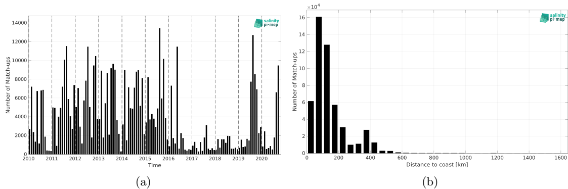
Figure 1: Number of match-ups between ICES and CCI SSS L4 Merged-OI v3.2 - 7-day running (ESA) SSS as a function of time (a) and as function of the distance to coast (b) over the Global Ocean Pi-MEP region and for the full satellite product period.
