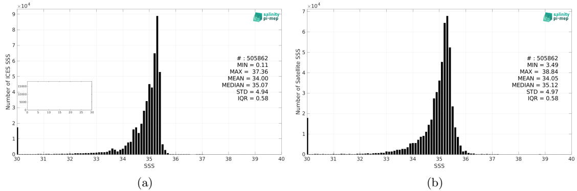
Figure 2: Histograms of SSS from ICES (a) and CCI SSS L4 Merged-OI v3.2 - 7-day running (ESA) (b) considering all match-up pairs per bins of 0.1 over the Global Ocean Pi-MEP region and for the full satellite product period.
