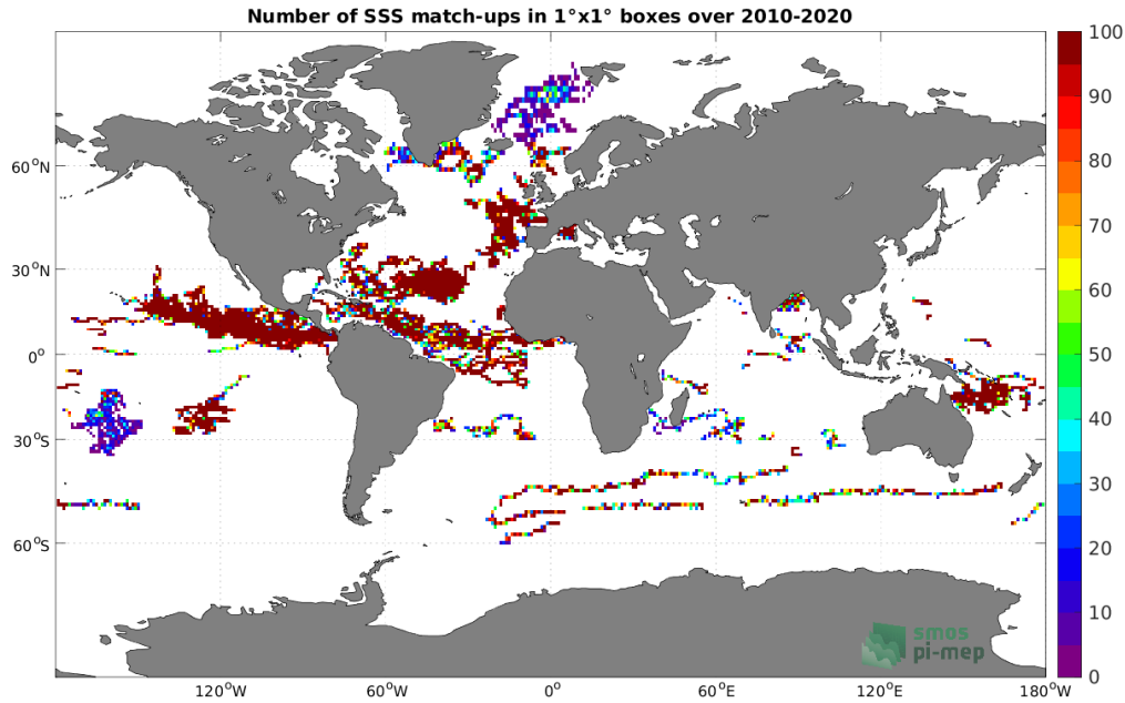
Figure 3: Number of SSS match-ups between Surface drifters SSS and the CCI SSS L4 Merged-OI v3.2 - 7-day running (ESA) SSS product for the Global Ocean Pi-MEP region over 1^\circ \times 1^\circ boxes and for the full satellite product period.
