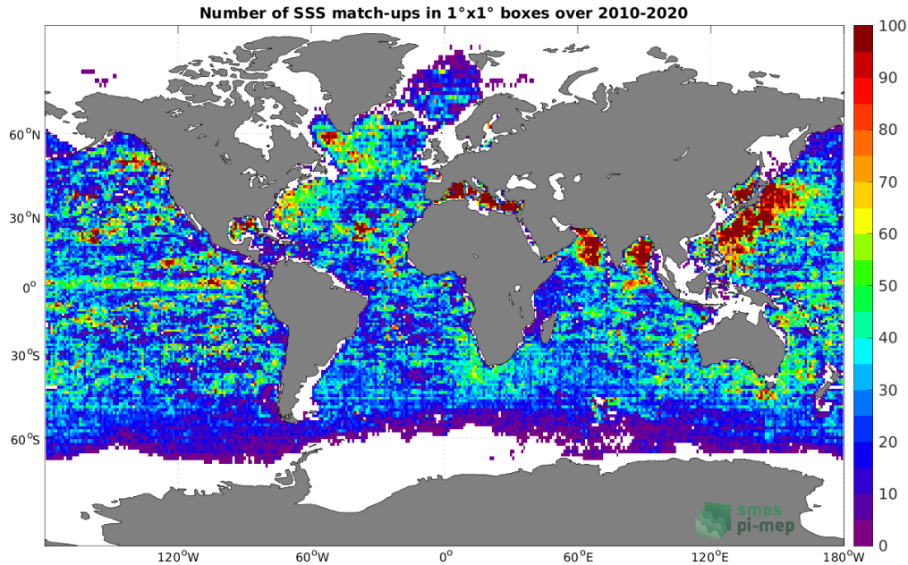
Figure 4: Number of SSS match-ups between Argo SSS and the CCI SSS L4 Merged-OI v3.2 - 7-day running (ESA) SSS product for the Global Ocean Pi-MEP region over 1^\circ \times 1^\circ boxes and for the full satellite product period.
