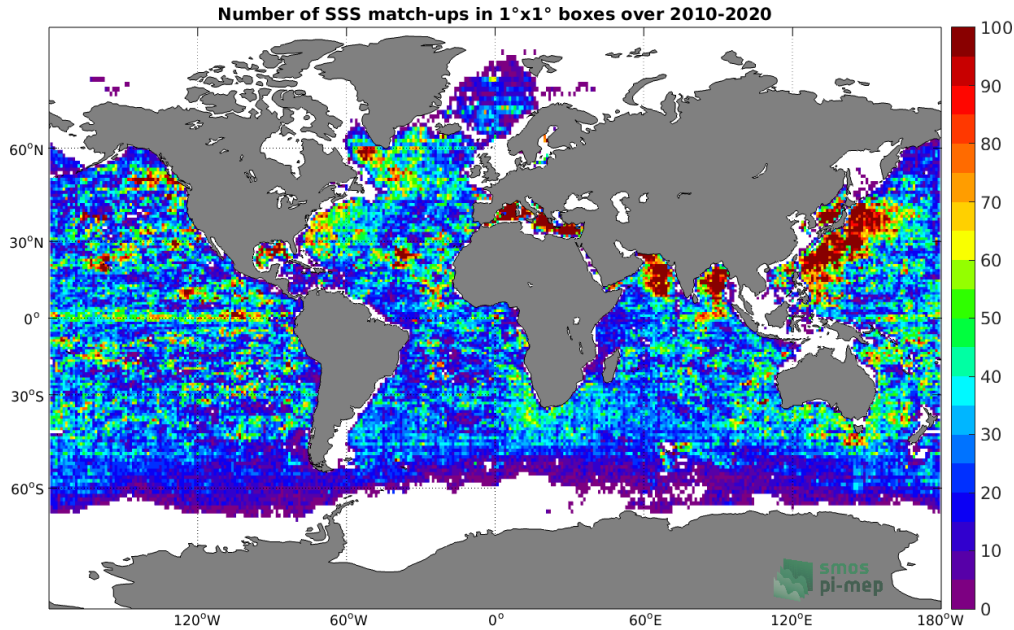
Figure 4: Number of SSS match-ups between Argo SSS and the CCI SSS L4 Merged-OI v3.2 - 7-day running (ESA) SSS product for the Global Ocean Pi-MEP region over 1^\circ \times 1^\circ boxes and for the full satellite product period.
