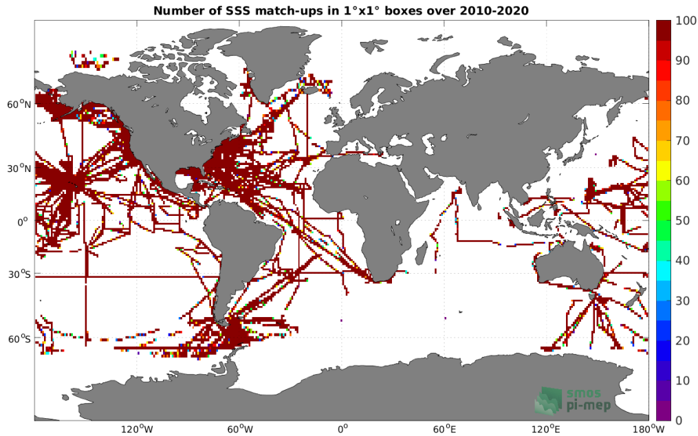
Figure 4: Number of SSS match-ups between TSG (SAMOS) SSS and the CCI SSS L4 Merged-OI v3.2 - 30-day running (ESA) SSS product for the Global Ocean Pi-MEP region over 1^\circ \times 1^\circ boxes and for the full satellite product period.
