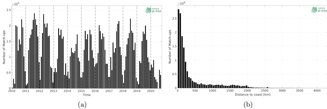
Figure 1: Number of match-ups between TSG (SAMOS) and CCI SSS L4 Merged-OI v3.2 - 30-day running (ESA) SSS as a function of time (a) and as function of the distance to coast (b) over the Global Ocean Pi-MEP region and for the full satellite product period.
