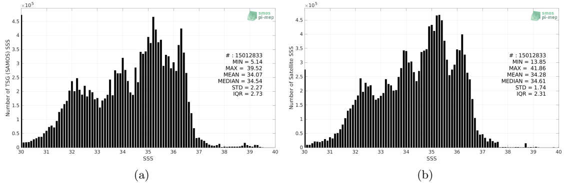
Figure 2: Histograms of SSS from TSG (SAMOS) (a) and CCI SSS L4 Merged-OI v3.2 - 30-day running (ESA) (b) considering all match-up pairs per bins of 0.1 over the Global Ocean Pi-MEP region and for the full satellite product period.
