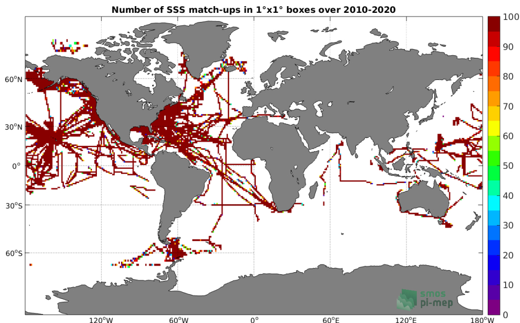
Figure 4: Number of SSS match-ups between TSG (SAMOS) SSS and the CCI SSS L4 Merged-OI v3.2 - 30-day running (ESA) SSS product for the Global Ocean Pi-MEP region over 1^\circ \times 1^\circ boxes and for the full satellite product period.
