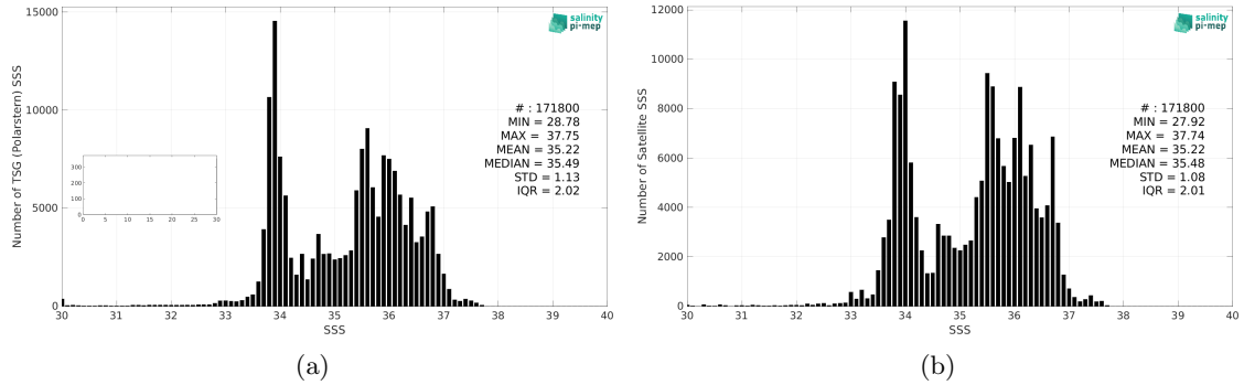
Figure 2: Histograms of SSS from TSG (Polarstern) (a) and CCI SSS L4 Merged-OI v3.2 - 30-day running (ESA) (b) considering all match-up pairs per bins of 0.1 over the Global Ocean Pi-MEP region and for the full satellite product period.
