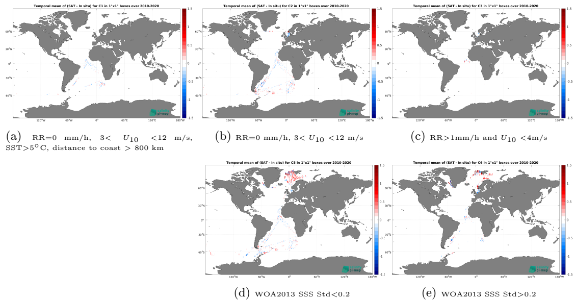
Figure 12: Temporal mean gridded over spatial boxes of size 1^\circ \times 1^\circ of \Delta\text{SSS} (CCI SSS L4 Merged-OI v3.2 - 30-day running (ESA) - TSG (Polarstern)) for 5 different subdatasets corresponding to: RR=0 mm/h, 3 < U_{10} < 12 m/s, SST > 5^\circ\text{C} , distance to coast > 800 km (a), RR=0 mm/h, 3 < U_{10} < 12 m/s (b), RR > 1\text{mm/h} and U_{10} < 4\text{m/s} (c), WOA2013 SSS Std < 0.2 (d), WOA2013 SSS Std > 0.2 (e).
