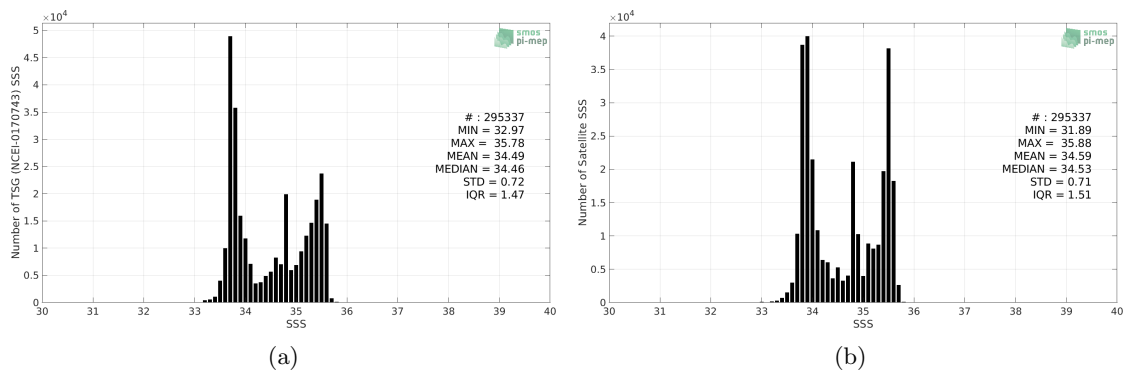
Figure 2: Histograms of SSS from TSG (NCEI-0170743) (a) and CCI SSS L4 Merged-OI v3.2 - 30-day running (ESA) (b) considering all match-up pairs per bins of 0.1 over the Global Ocean Pi-MEP region and for the full satellite product period.
