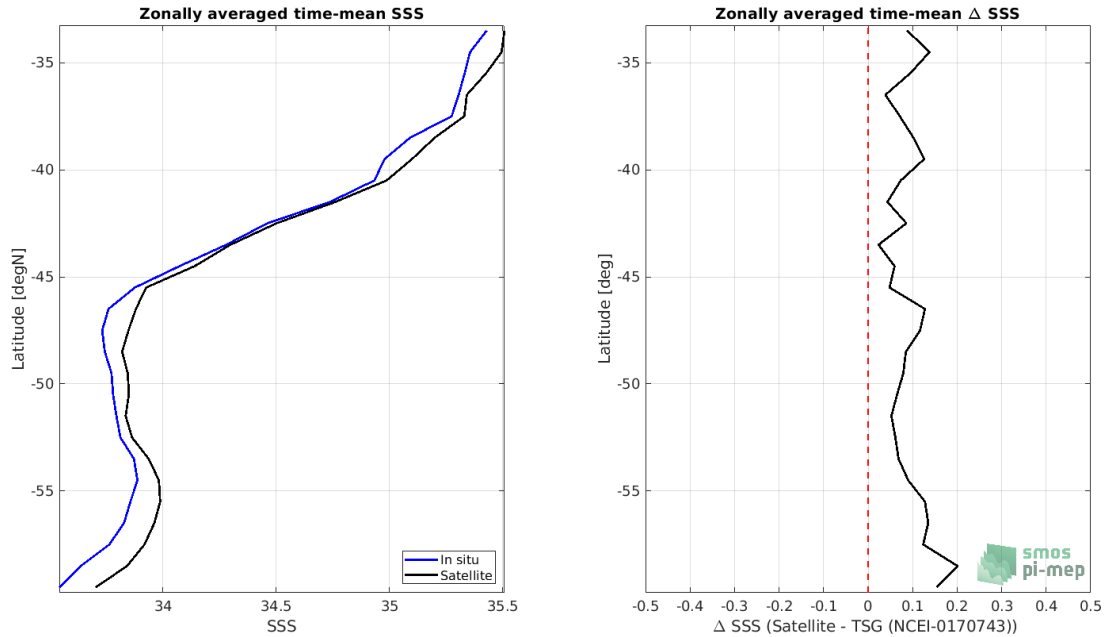
Figure 8: Left panel: Zonal mean SSS from CCI SSS L4 Merged-OI v3.2 - 30-day running (ESA) satellite product (black) and from TSG (NCEI-0170743) (blue). Right panel: Zonal mean of \Delta SSS (Satellite - TSG (NCEI-0170743)) for all the collected Pi-MEP match-up pairs estimated over the full satellite product period.
