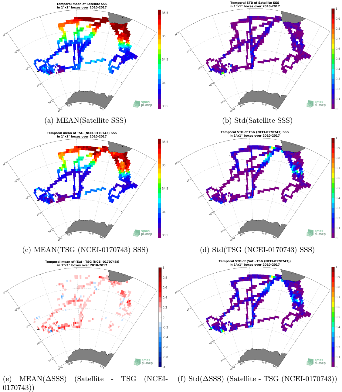
Figure 6: Temporal mean (left) and Std (right) of SSS from CCI SSS L4 Merged-OI v3.2 - 30-day running (ESA) (top), TSG (NCEI-0170743) (middle), and of \Delta SSS (Satellite - TSG (NCEI-0170743)). Only match-up pairs are used to generate these maps.
