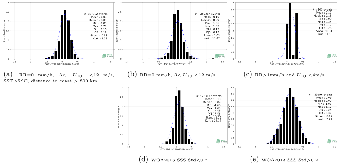
Figure 13: Normalized histogram of \Delta SSS (CCI SSS L4 Merged-OI v3.2 - 30-day running (ESA) - TSG (NCEI-0170743)) for 5 different subdatasets corresponding to: RR=0 mm/h, 3 < U_{10} < 12 m/s, SST>5°C, distance to coast > 800 km (a), RR=0 mm/h, 3 < U_{10} < 12 m/s (b), RR>1mm/h and U_{10} < 4 m/s (c), WOA2013 SSS Std<0.2 (d), WOA2013 SSS Std>0.2 (e).
