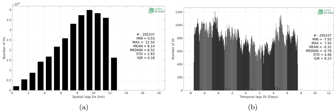
Figure 5: Histograms of the spatial (a) and temporal (b) lags between the location/time of the TSG (NCEI-0170743) measurement and the date of the corresponding CCI SSS L4 Merged-OI v3.2 - 30-day running (ESA) SSS pixel.
