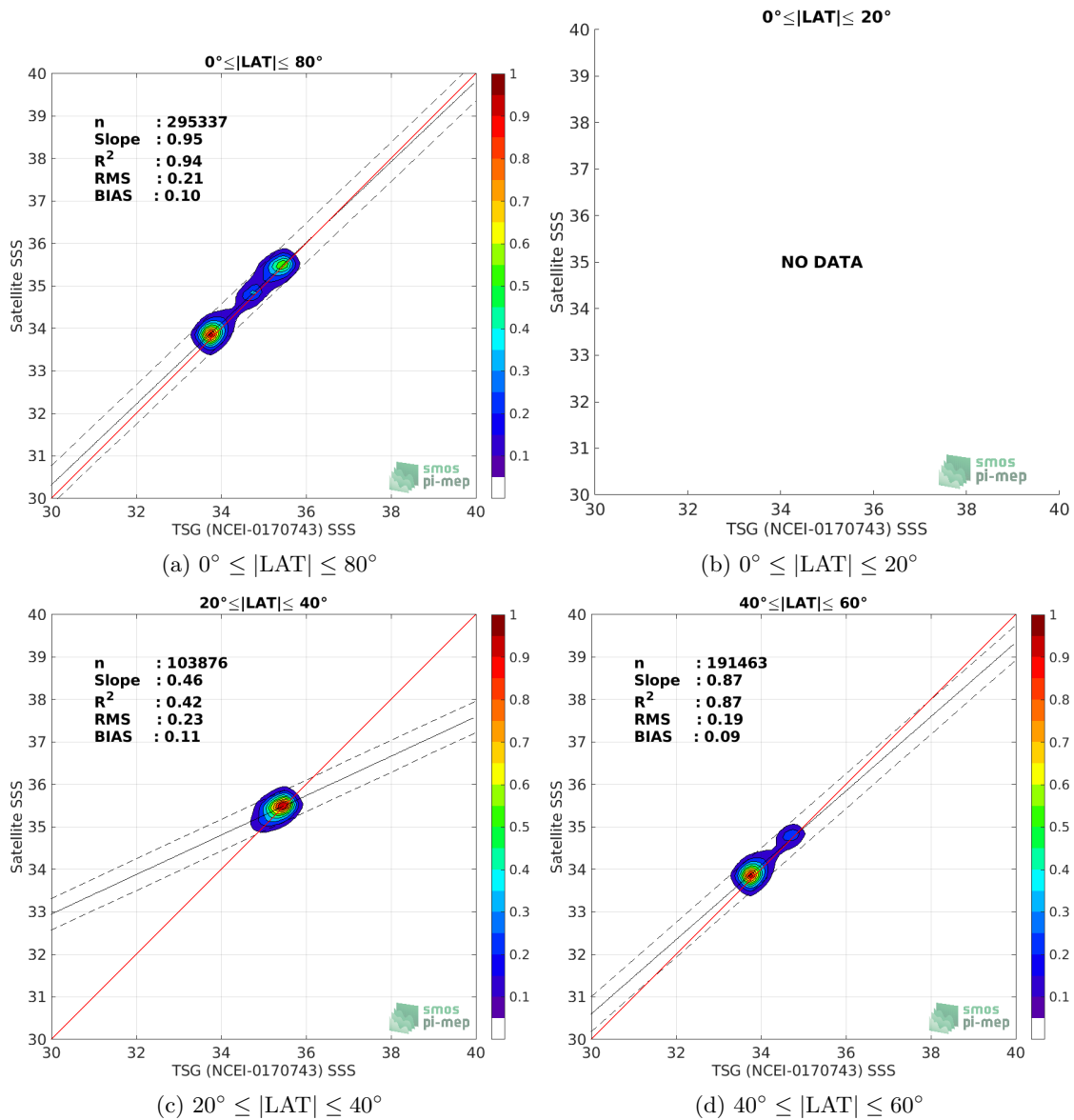
Figure 9: Contour maps of the concentration of CCI SSS L4 Merged-OI v3.2 - 30-day running (ESA) SSS (y-axis) versus TSG (NCEI-0170743) SSS (x-axis) at match-up pairs for different latitude bands. For each plot, the red line shows x=y . The black thin and dashed lines indicate a linear fit through the data cloud and the \pm 95\% confidence levels, respectively. The number match-up pairs n , the slope and R^2 coefficient of the linear fit, the root mean square (RMS) and the mean bias between satellite and in situ data are indicated for each latitude band in each plots.
