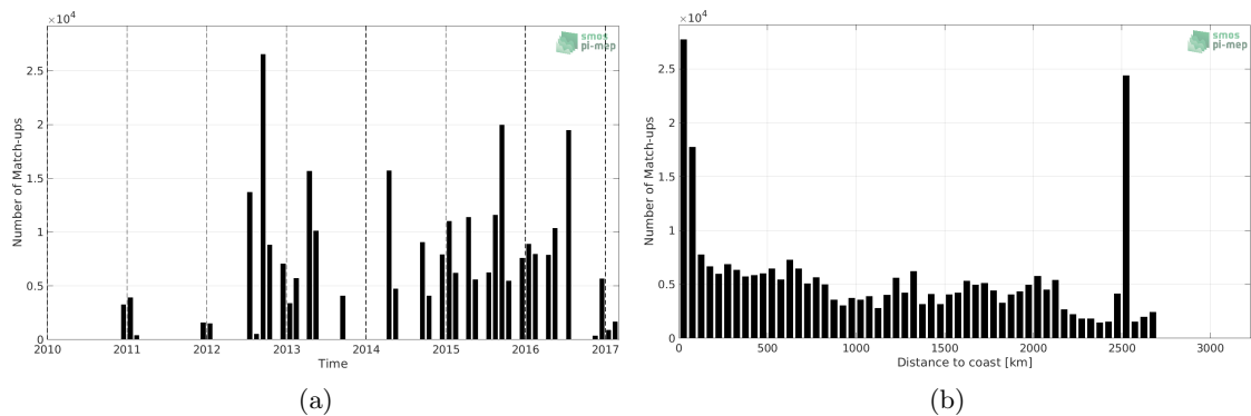
Figure 1: Number of match-ups between TSG (NCEI-0170743) and CCI SSS L4 Merged-OI v3.2 - 30-day running (ESA) SSS as a function of time (a) and as function of the distance to coast (b) over the Global Ocean Pi-MEP region and for the full satellite product period.
