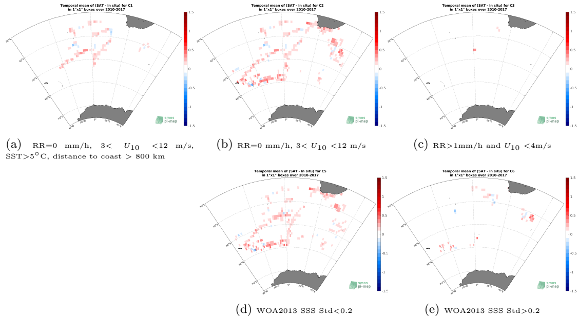
Figure 12: Temporal mean gridded over spatial boxes of size 1^{\circ}\times 1^{\circ} of \Delta\text{SSS} (CCI SSS L4 Merged-OI v3.2 - 30-day running (ESA) - TSG (NCEI-0170743)) for 5 different subdatasets corresponding to:RR=0 mm/h, 3 < U_{10} < 12 m/s, SST >5^{\circ}\text{C} , distance to coast > 800 km (a), RR=0 mm/h, 3 < U_{10} < 12 m/s (b), RR >1 mm/h and U_{10} < 4 m/s (c), WOA2013 SSS Std <0.2 (d), WOA2013 SSS Std >0.2 (e).
