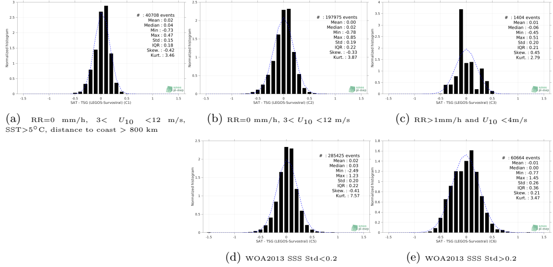
Figure 13: Normalized histogram of \Delta SSS (CCI SSS L4 Merged-OI v3.2 - 30-day running (ESA) - TSG (LEGOS-Survostral)) for 5 different subdatasets corresponding to: RR=0 mm/h, 3 < U_{10} < 12 m/s, SST > 5°C, distance to coast > 800 km (a), RR=0 mm/h, 3 < U_{10} < 12 m/s (b), RR > 1mm/h and U_{10} < 4 m/s (c), WOA2013 SSS Std < 0.2 (d), WOA2013 SSS Std > 0.2 (e).
