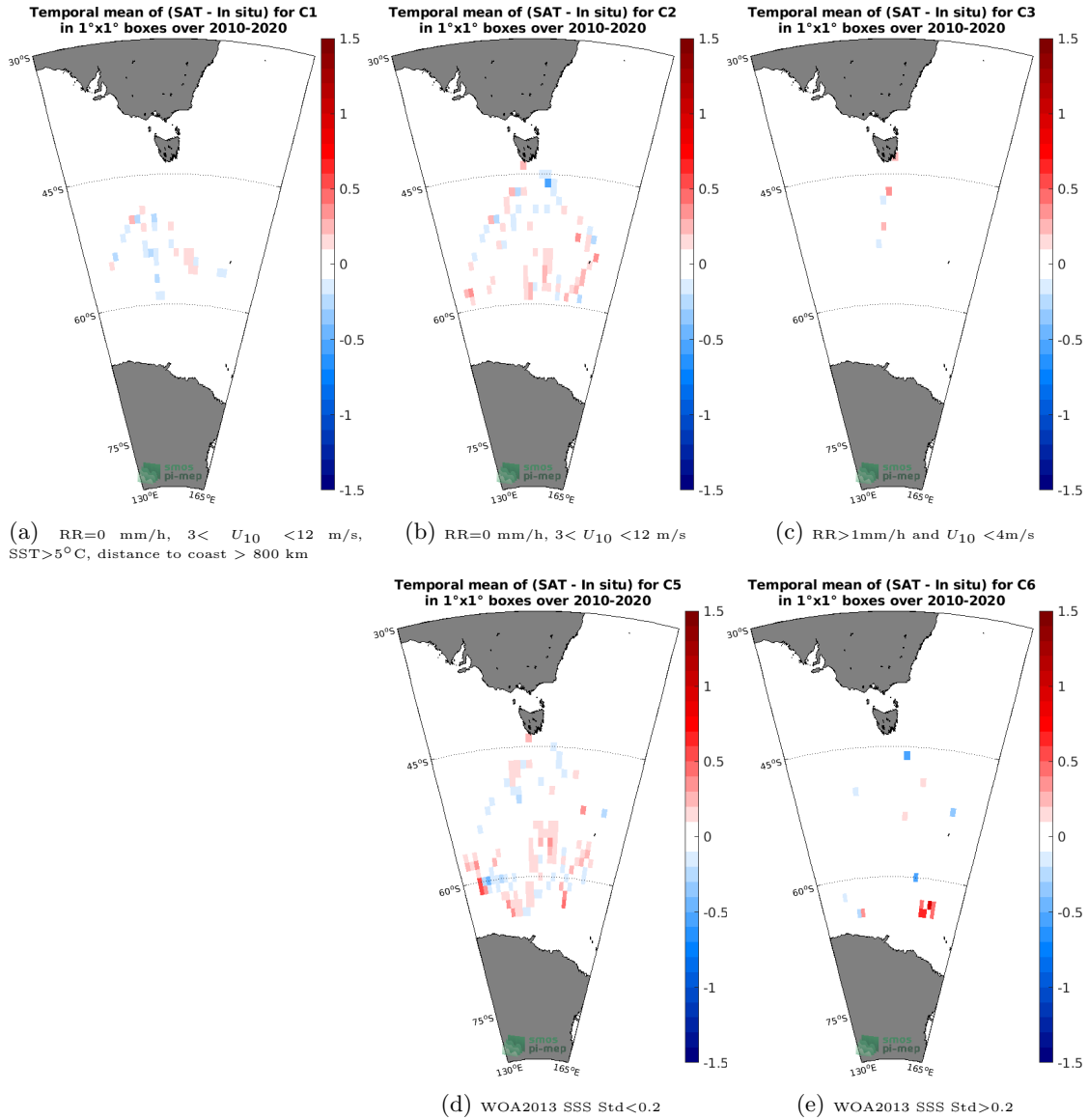
Figure 12: Temporal mean gridded over spatial boxes of size 1°x1° of \Delta SSS (CCI SSS L4 Merged-OI v3.2 - 30-day running (ESA) - TSG (LEGOS-Survostral)) for 5 different subdatasets corresponding to:RR=0 mm/h, 3 < U_{10} < 12 m/s, SST>5°C, distance to coast > 800 km (a), RR=0 mm/h, 3 < U_{10} < 12 m/s (b), RR>1mm/h and U_{10} < 4 m/s (c), WOA2013 SSS Std<0.2 (d), WOA2013 SSS Std>0.2 (e).
