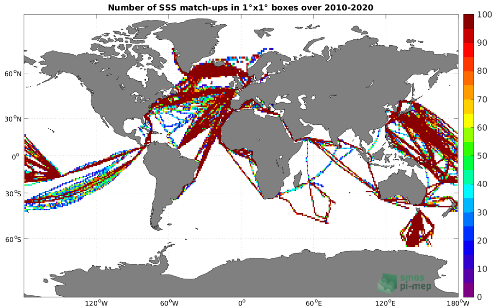
Figure 4: Number of SSS match-ups between TSG (LEGOS-DM) SSS and the CCI SSS L4 Merged-OI v3.2 - 30-day running (ESA) SSS product for the Global Ocean Pi-MEP region over 1^\circ \times 1^\circ boxes and for the full satellite product period.
