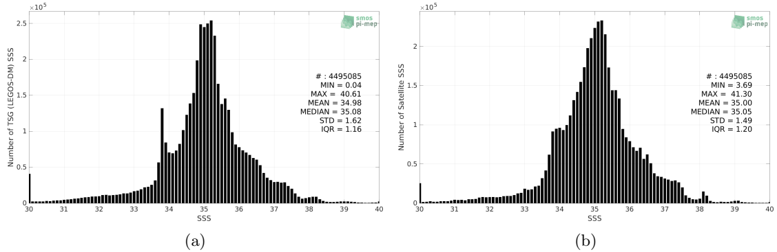
Figure 2: Histograms of SSS from TSG (LEGOS-DM) (a) and CCI SSS L4 Merged-OI v3.2 - 30-day running (ESA) (b) considering all match-up pairs per bins of 0.1 over the Global Ocean Pi-MEP region and for the full satellite product period.
