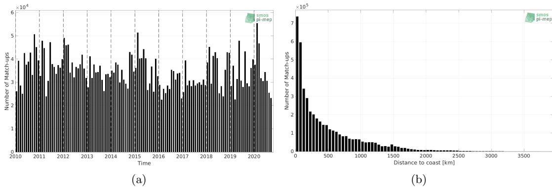
Figure 1: Number of match-ups between TSG (LEGOS-DM) and CCI SSS L4 Merged-OI v3.2 - 30-day running (ESA) SSS as a function of time (a) and as function of the distance to coast (b) over the Global Ocean Pi-MEP region and for the full satellite product period.
