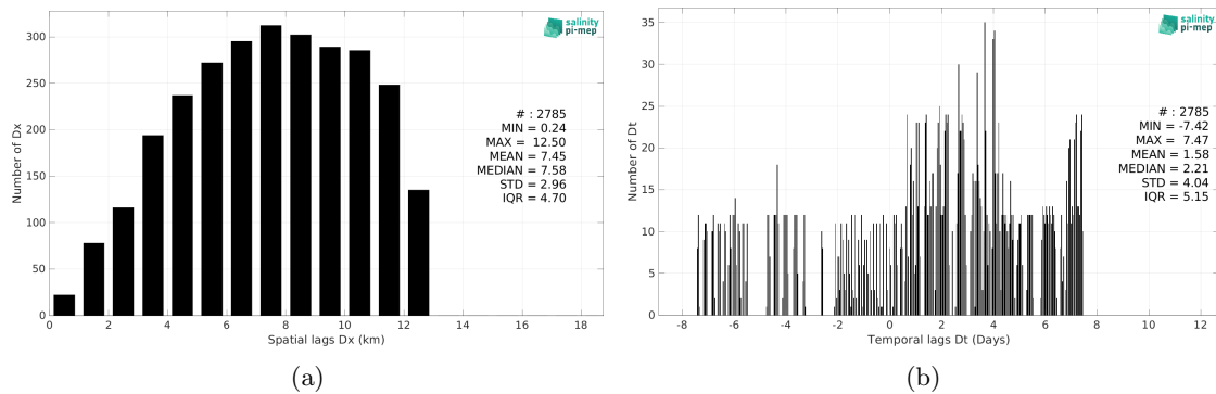
Figure 5: Histograms of the spatial (a) and temporal (b) lags between the location/time of the TSG (Lauge-Koch) measurement and the date of the corresponding CCI SSS L4 Merged-OI v3.2 - 30-day running (ESA) SSS pixel.
