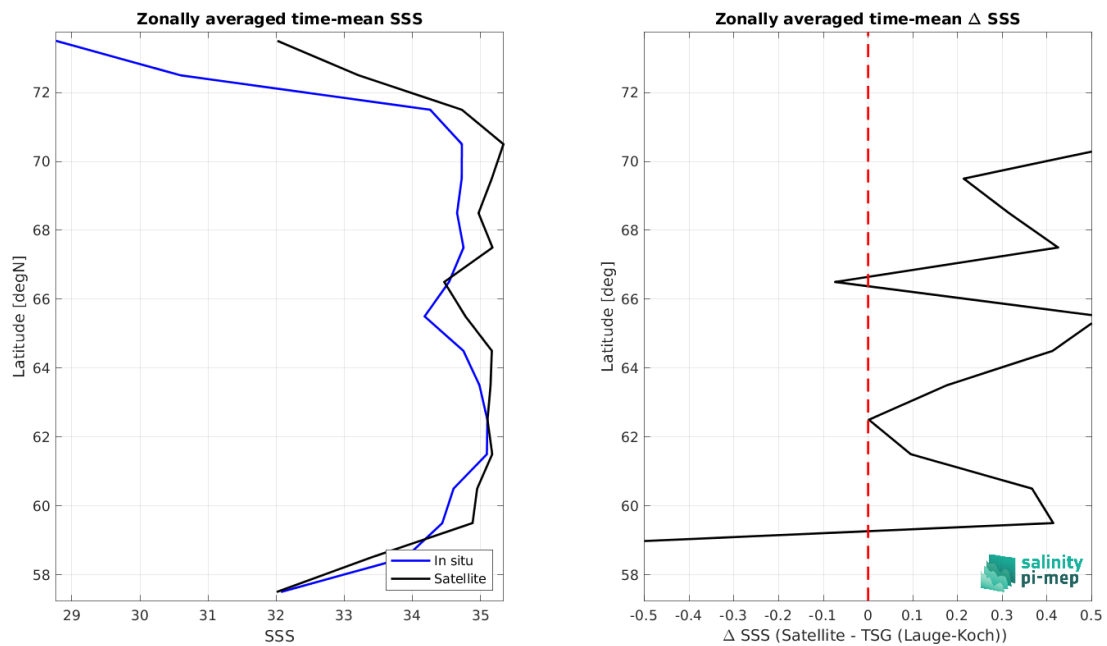
Figure 8: Left panel: Zonal mean SSS from CCI SSS L4 Merged-OI v3.2 - 30-day running (ESA) satellite product (black) and from TSG (Lauge-Koch) (blue). Right panel: Zonal mean of \Delta SSS (Satellite - TSG (Lauge-Koch)) for all the collected Pi-MEP match-up pairs estimated over the full satellite product period.
