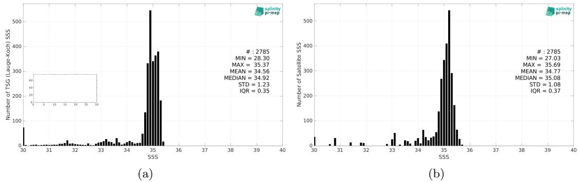
Figure 2: Histograms of SSS from TSG (Lauge-Koch) (a) and CCI SSS L4 Merged-OI v3.2 - 30-day running (ESA) (b) considering all match-up pairs per bins of 0.1 over the Global Ocean Pi-MEP region and for the full satellite product period.
