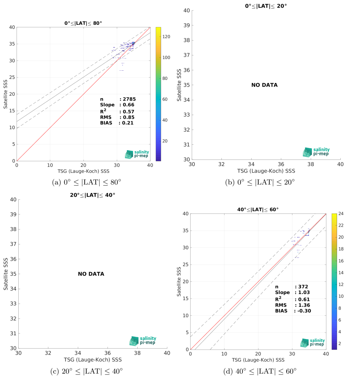
Figure 9: Contour maps of the concentration of CCI SSS L4 Merged-OI v3.2 - 30-day running (ESA) SSS (y-axis) versus TSG (Lauge-Koch) SSS (x-axis) at match-up pairs for different latitude bands. For each plot, the red line shows x=y . The black thin and dashed lines indicate a linear fit through the data cloud and the \pm 95\% confidence levels, respectively. The number match-up pairs n , the slope and R^2 coefficient of the linear fit, the root mean square (RMS) and the mean bias between satellite and in situ data are indicated for each latitude band in each plots.
