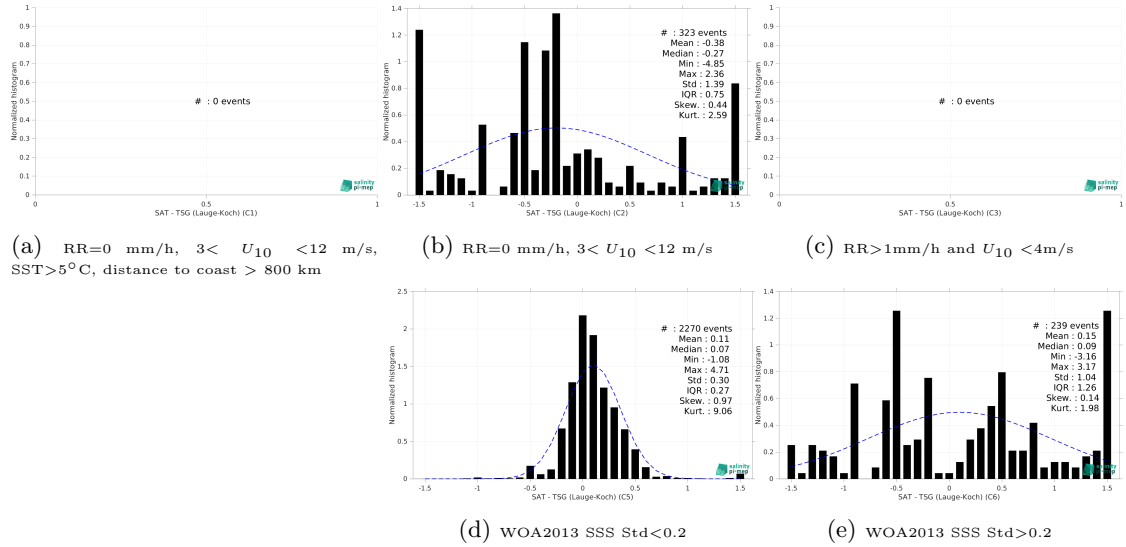
Figure 13: Normalized histogram of \Delta SSS (CCI SSS L4 Merged-OI v3.2 - 30-day running (ESA) - TSG (Laue-Koch)) for 5 different subdatasets corresponding to: RR=0 mm/h, 3 < U_{10} < 12 m/s, SST > 5°C, distance to coast > 800 km (a), RR=0 mm/h, 3 < U_{10} < 12 m/s (b), RR > 1mm/h and U_{10} < 4 m/s (c), WOA2013 SSS Std < 0.2 (d), WOA2013 SSS Std > 0.2 (e).
