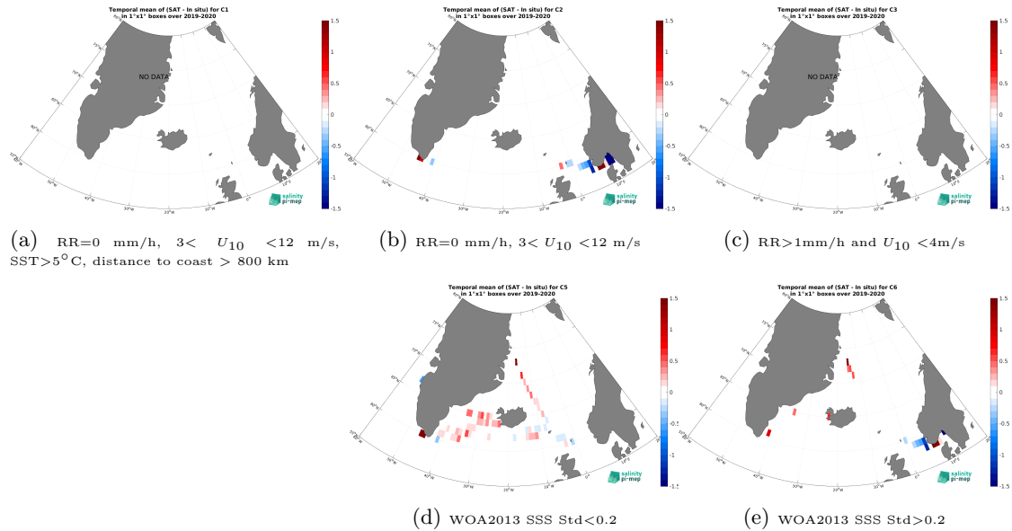
Figure 12: Temporal mean gridded over spatial boxes of size 1^{\circ}\times 1^{\circ} of \Delta\text{SSS} (CCI SSS L4 Merged-OI v3.2 - 30-day running (ESA) - TSG (Lauge-Koch)) for 5 different subdatasets corresponding to:RR=0 mm/h, 3 < U_{10} < 12 m/s, SST >5^{\circ}\text{C} , distance to coast > 800 km (a), RR=0 mm/h, 3 < U_{10} < 12 m/s (b), RR >1 mm/h and U_{10} < 4 m/s (c), WOA2013 SSS Std <0.2 (d), WOA2013 SSS Std >0.2 (e).
