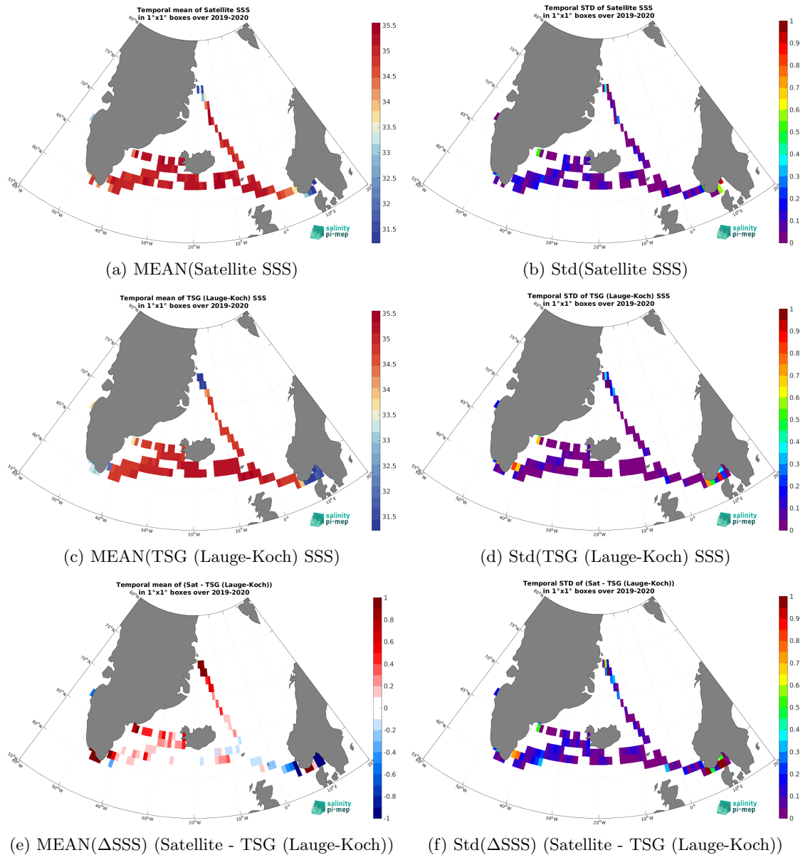
Figure 6: Temporal mean (left) and Std (right) of SSS from CCI SSS L4 Merged-OI v3.2 - 30-day running (ESA) (top), TSG (Lauge-Koch) (middle), and of \Delta SSS (Satellite - TSG (Lauge-Koch)). Only match-up pairs are used to generate these maps.
