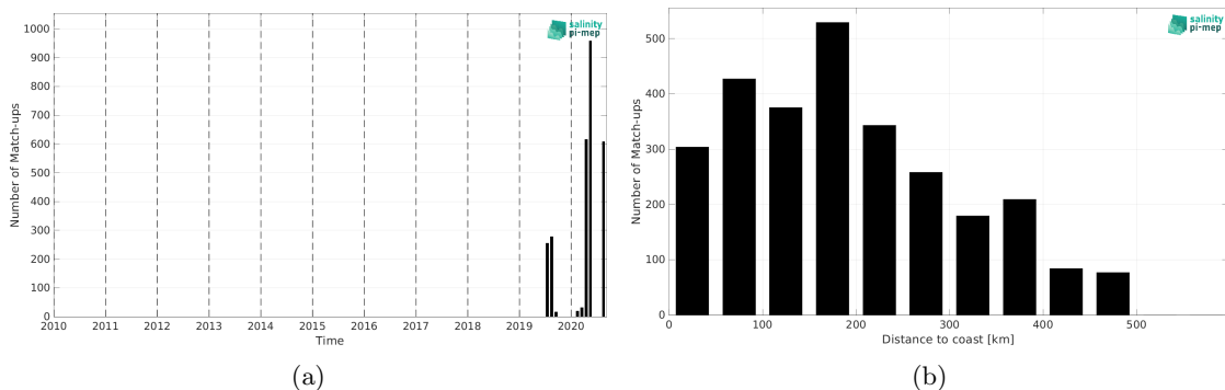
Figure 1: Number of match-ups between TSG (Lauge-Koch) and CCI SSS L4 Merged-OI v3.2 - 30-day running (ESA) SSS as a function of time (a) and as function of the distance to coast (b) over the Global Ocean Pi-MEP region and for the full satellite product period.
