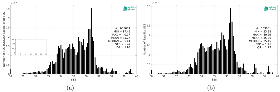
Figure 2: Histograms of SSS from TSG (GOSUD-Sailing-ship) (a) and CCI SSS L4 Merged-OI v3.2 - 30-day running (ESA) (b) considering all match-up pairs per bins of 0.1 over the Global Ocean Pi-MEP region and for the full satellite product period.
