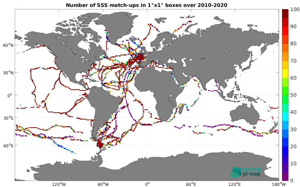
Figure 4: Number of SSS match-ups between TSG (GOSUD-Sailing-ship) SSS and the CCI SSS L4 Merged-OI v3.2 - 30-day running (ESA) SSS product for the Global Ocean Pi-MEP region over 1^\circ \times 1^\circ boxes and for the full satellite product period.
