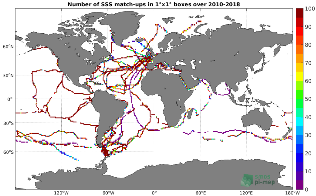
Figure 4: Number of SSS match-ups between TSG (GOSUD-Sailing-ship) SSS and the CCI SSS L4 Merged-OI v3.2 - 30-day running (ESA) SSS product for the Global Ocean Pi-MEP region over 1^\circ \times 1^\circ boxes and for the full satellite product period.
