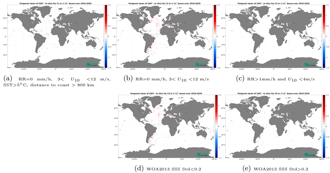
Figure 12: Temporal mean gridded over spatial boxes of size 1^\circ \times 1^\circ of \Delta\text{SSS} (CCI SSS L4 Merged-OI v3.2 - 30-day running (ESA) - TSG (CSIC-UTM)) for 5 different subdatasets corresponding to: RR=0 mm/h, 3 < U_{10} < 12 m/s, SST > 5^\circ\text{C} , distance to coast > 800 km (a), RR=0 mm/h, 3 < U_{10} < 12 m/s (b), RR > 1\text{mm/h} and U_{10} < 4\text{m/s} (c), WOA2013 SSS Std < 0.2 (d), WOA2013 SSS Std > 0.2 (e).
