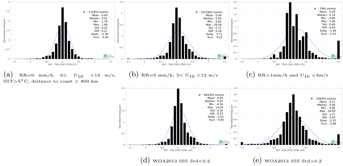
Figure 13: Normalized histogram of \Delta\text{SSS} (CCI SSS L4 Merged-OI v3.2 - 30-day running (ESA) - TSG (CSIC-UTM)) for 5 different subdatasets corresponding to: RR=0 mm/h, 3 < U_{10} < 12 m/s, SST>5°C, distance to coast > 800 km (a), RR=0 mm/h, 3 < U_{10} < 12 m/s (b), RR>1mm/h and U_{10} < 4 m/s (c), WOA2013 SSS Std<0.2 (d), WOA2013 SSS Std>0.2 (e).
