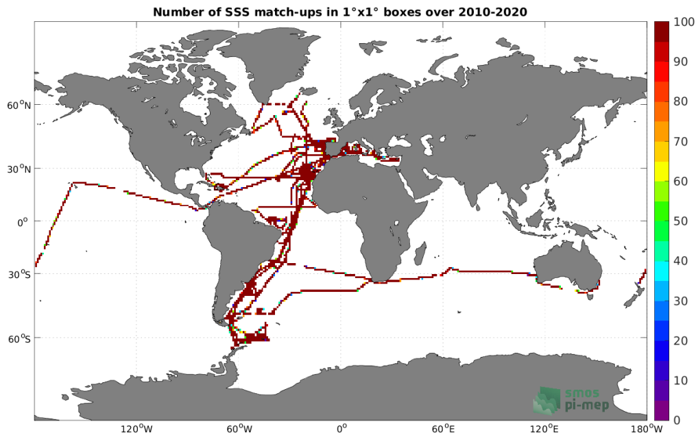
Figure 4: Number of SSS match-ups between TSG (CSIC-UTM) SSS and the CCI SSS L4 Merged-OI v3.2 - 30-day running (ESA) SSS product for the Global Ocean Pi-MEP region over 1^\circ \times 1^\circ boxes and for the full satellite product period.
