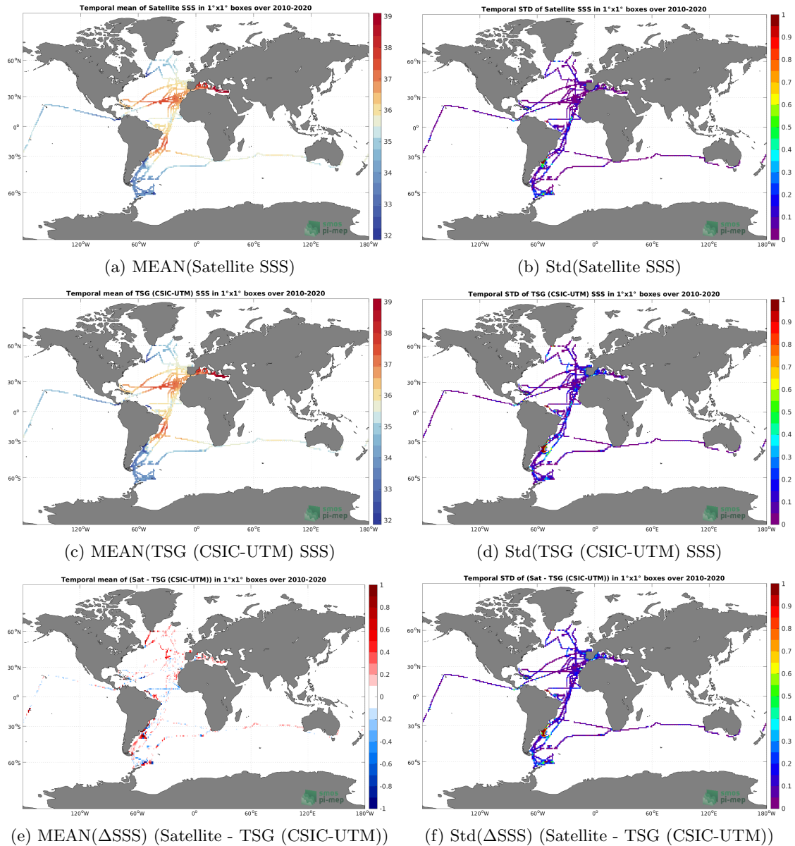
Figure 6: Temporal mean (left) and Std (right) of SSS from CCI SSS L4 Merged-OI v3.2 - 30-day running (ESA) (top), TSG (CSIC-UTM) (middle), and of \Delta SSS (Satellite - TSG (CSIC-UTM)). Only match-up pairs are used to generate these maps.
