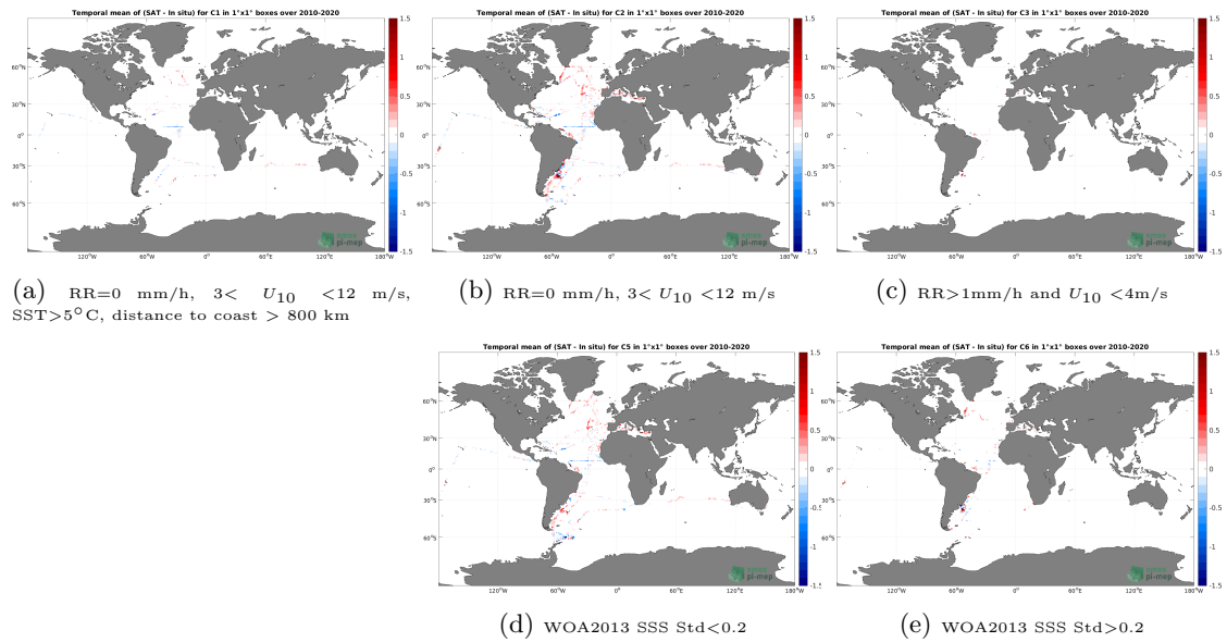
Figure 12: Temporal mean gridded over spatial boxes of size 1^\circ \times 1^\circ of \Delta SSS (CCI SSS L4 Merged-OI v3.2 - 30-day running (ESA) - TSG (CSIC-UTM)) for 5 different subdatasets corresponding to:RR=0 mm/h, 3 < U_{10} < 12 m/s, SST >5^\circ C, distance to coast > 800 km (a), RR=0 mm/h, 3 < U_{10} < 12 m/s (b), RR >1 mm/h and U_{10} < 4 m/s (c), WOA2013 SSS Std <0.2 (d), WOA2013 SSS Std >0.2 (e).
