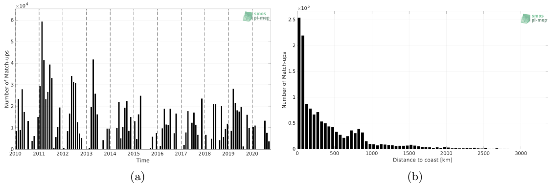
Figure 1: Number of match-ups between TSG (CSIC-UTM) and CCI SSS L4 Merged-OI v3.2 - 30-day running (ESA) SSS as a function of time (a) and as function of the distance to coast (b) over the Global Ocean Pi-MEP region and for the full satellite product period.
