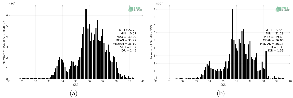
Figure 2: Histograms of SSS from TSG (CSIC-UTM) (a) and CCI SSS L4 Merged-OI v3.2 - 30-day running (ESA) (b) considering all match-up pairs per bins of 0.1 over the Global Ocean Pi-MEP region and for the full satellite product period.
