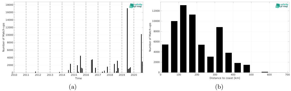
Figure 1: Number of match-ups between TSG (Amundsen) and CCI SSS L4 Merged-OI v3.2 - 30-day running (ESA) SSS as a function of time (a) and as function of the distance to coast (b) over the Global Ocean Pi-MEP region and for the full satellite product period.
