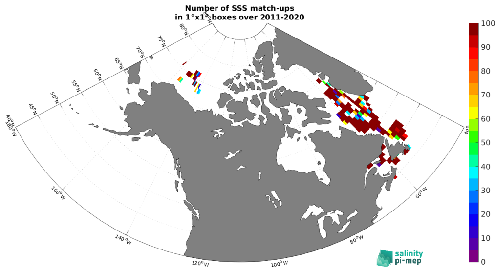
Figure 4: Number of SSS match-ups between TSG (Amundsen) SSS and the CCI SSS L4 Merged-OI v3.2 - 30-day running (ESA) SSS product for the Global Ocean Pi-MEP region over 1^\circ \times 1^\circ boxes and for the full satellite product period.
