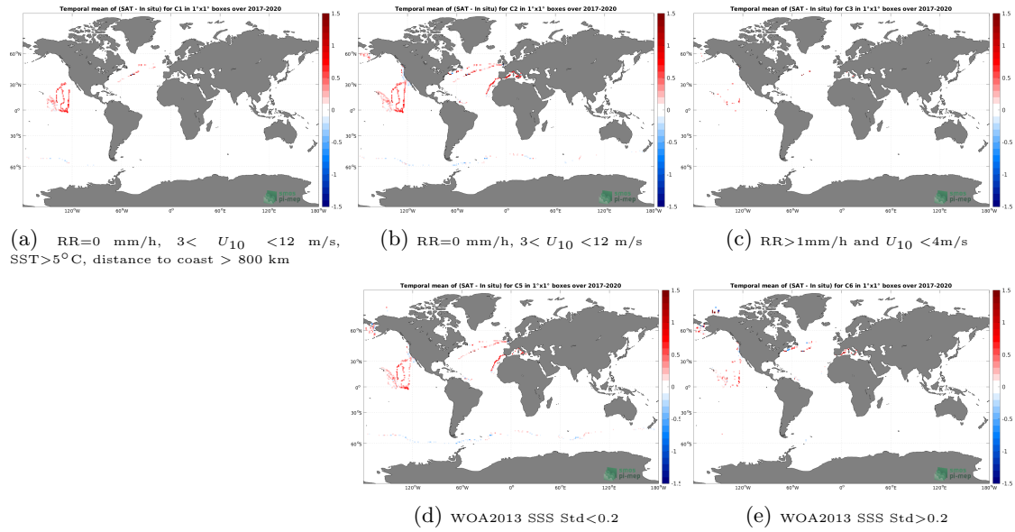
Figure 12: Temporal mean gridded over spatial boxes of size 1^\circ \times 1^\circ of \Delta SSS (CCI SSS L4 Merged-OI v3.2 - 30-day running (ESA) - Saildrone) for 5 different subdatasets corresponding to:RR=0 mm/h, 3 < U_{10} < 12 m/s, SST > 5^\circ\text{C} , distance to coast > 800 km (a), RR=0 mm/h, 3 < U_{10} < 12 m/s (b), RR > 1 mm/h and U_{10} < 4 m/s (c), WOA2013 SSS Std < 0.2 (d), WOA2013 SSS Std > 0.2 (e).
