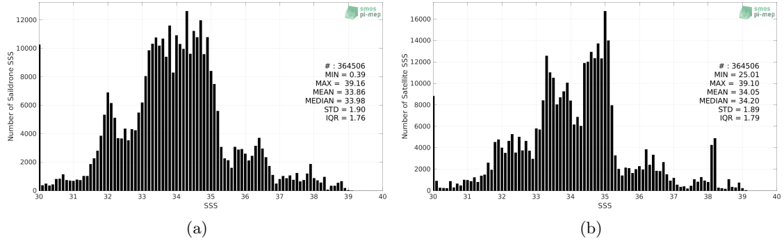
Figure 2: Histograms of SSS from Saildrone (a) and CCI SSS L4 Merged-OI v3.2 - 30-day running (ESA) (b) considering all match-up pairs per bins of 0.1 over the Global Ocean Pi-MEP region and for the full satellite product period.
