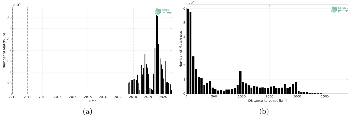
Figure 1: Number of match-ups between Saildrone and CCI SSS L4 Merged-OI v3.2 - 30-day running (ESA) SSS as a function of time (a) and as function of the distance to coast (b) over the Global Ocean Pi-MEP region and for the full satellite product period.
