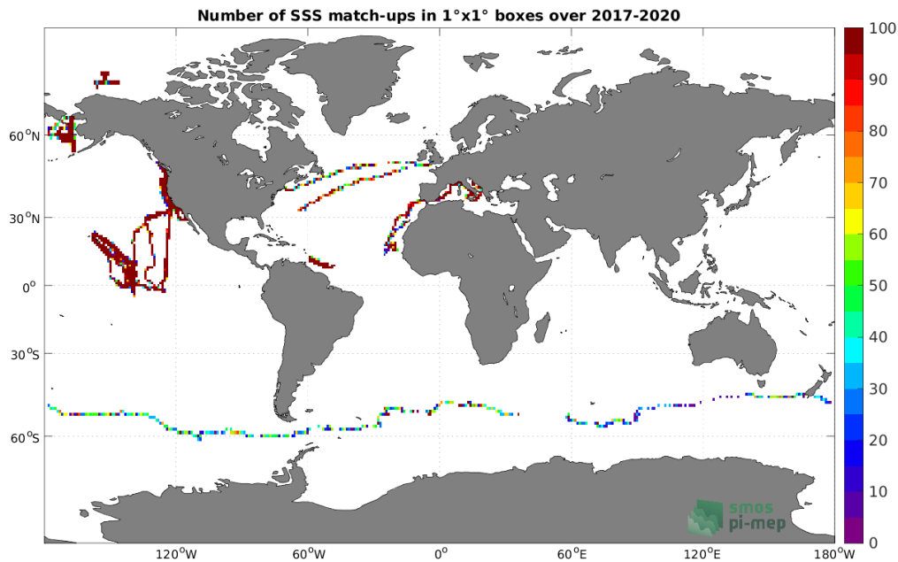
Figure 4: Number of SSS match-ups between Saildrone SSS and the CCI SSS L4 Merged-OI v3.2 - 30-day running (ESA) SSS product for the Global Ocean Pi-MEP region over 1^\circ \times 1^\circ boxes and for the full satellite product period.
